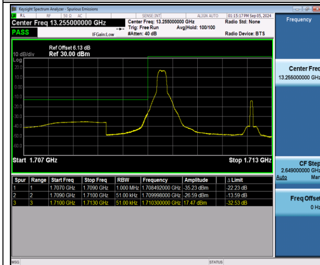
Band66-5MHz-QPSK-131997-1RB#0-PASS
