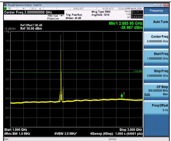
Band66-20MHz-QPSK-132572-1RB#0-1000~3000-PASS
