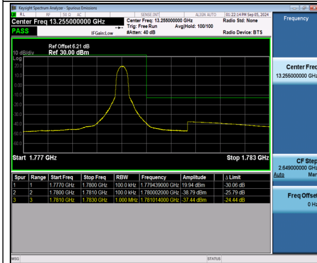
Band66-10MHz-QPSK-132622-1RB#49-PASS
