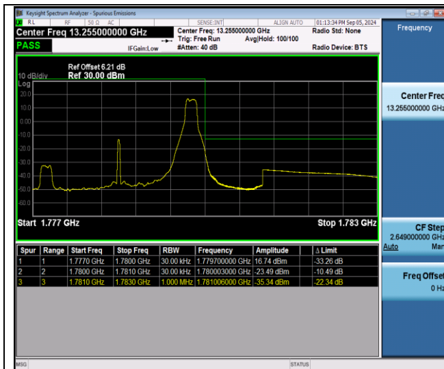
Band66-3MHz-QPSK-132657-1RB#14-PASS
