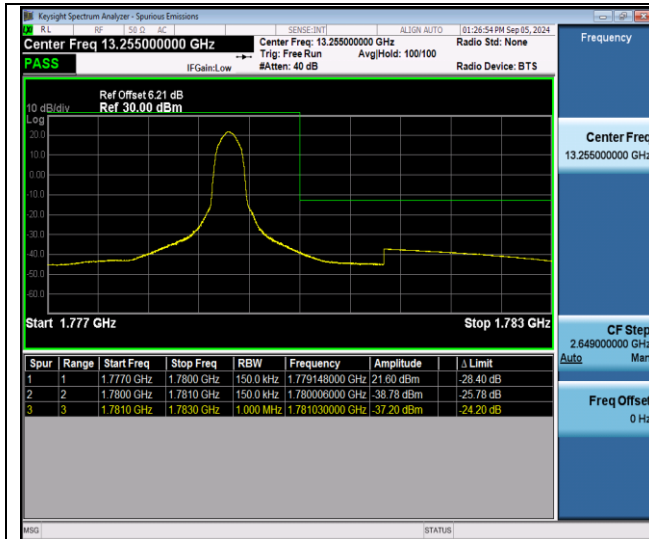
Band66-15MHz-QPSK-132597-1RB#74-PASS
