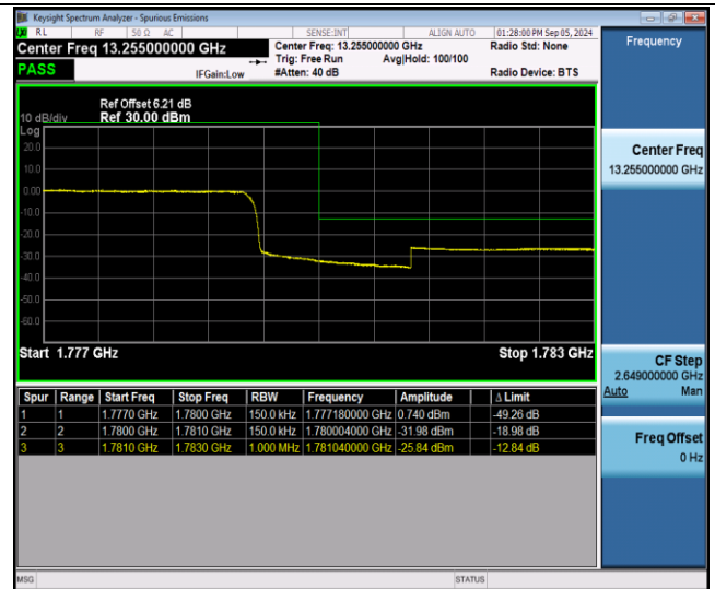
Band66-15MHz-QPSK-132597-75RB#0-PASS
