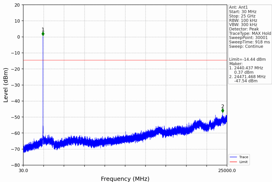
Pi/4DQPSK_2DH5_MCH_2441MHz_Ant1_NTNV
