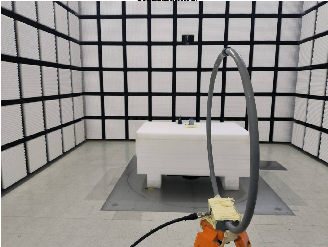
Radiated Emission 9kHz-30MHz View Ground-parallel-Worst Adapter 3# +Configuration 2#
