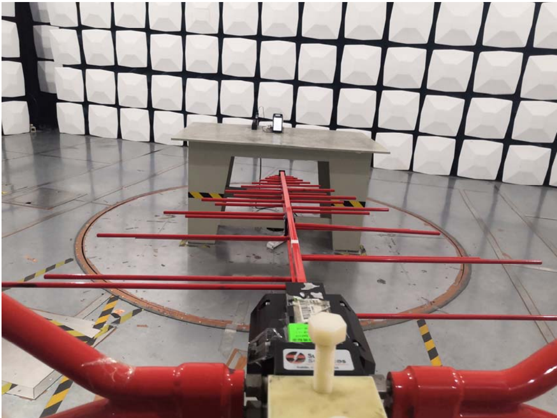
Radiated Emission Above 30MHz View
