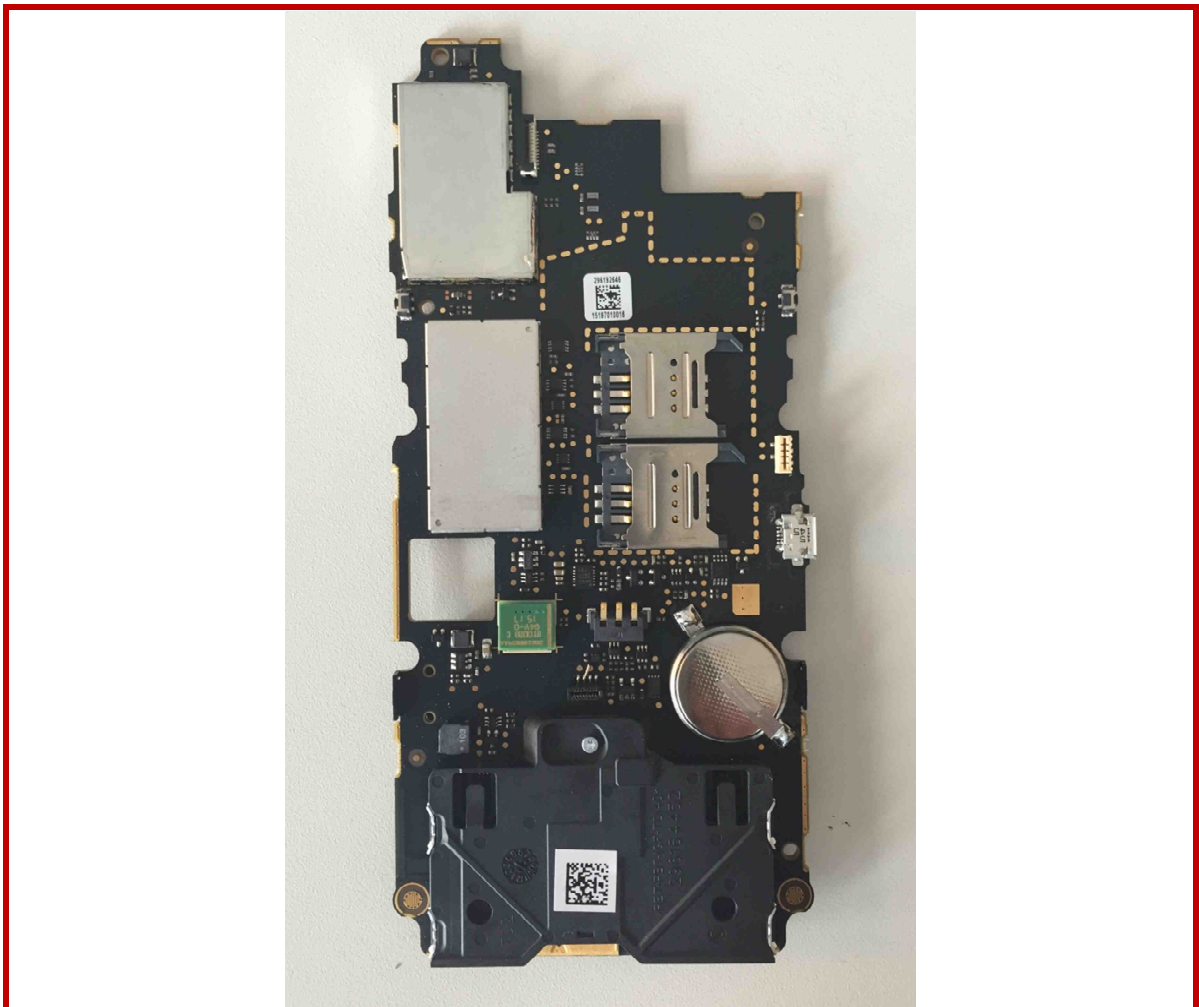
Figure #9 : Bottom side of the Main board
