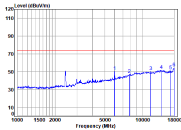
11n_40M_TX_CH_03_Horizontal-Peak
