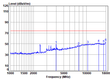
11n_40M_TX_CH_09_Vertical-Peak
