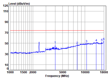
11n_40M_TX_CH_03_Vertical-Peak
