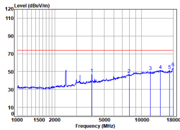
11n_40M_TX_CH_09_Horizontal-Peak
