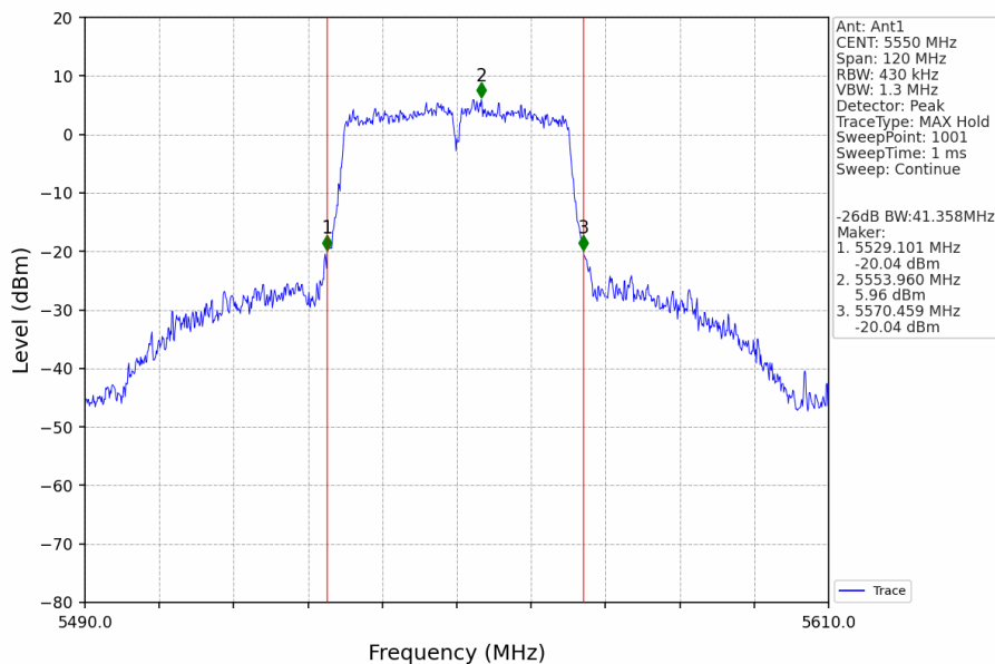
802.11ac(VHT40)_MCH_5550MHz_Ant1_NTNV
