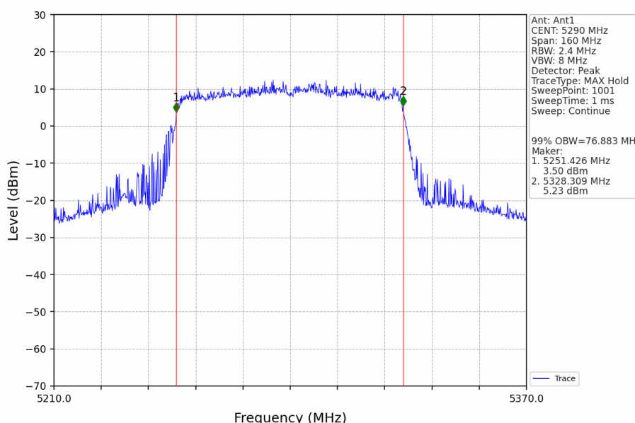
802.11ac(VHT80)_MCH_5290MHz_Ant1_NTNV
