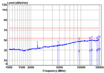
BT_DH5_TX_CH_78_Vertical
