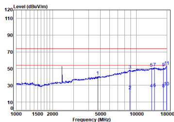
BT_DH5_TX_CH_00_Horizontal
