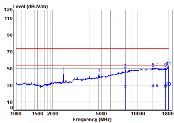
BT_DH5_TX_CH_39_Vertical
