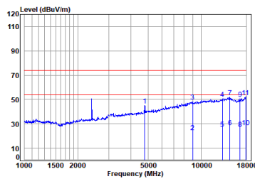
BT_DH5_TX_CH_00_Vertical
