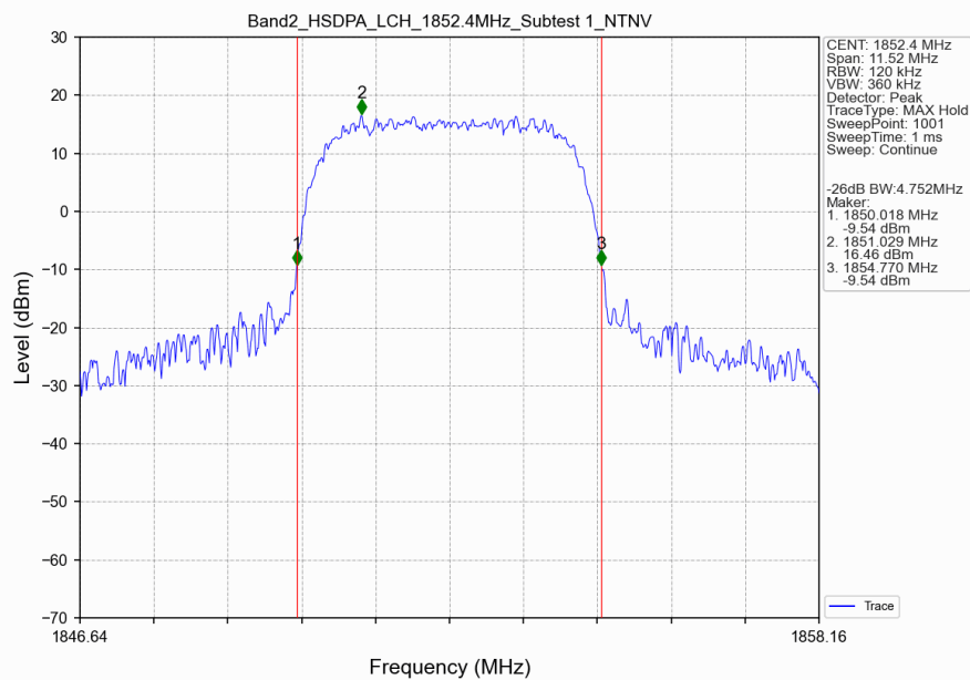
Band2_HSDPA_LCH_1852.4MHz_Subtest 1_NTNV
