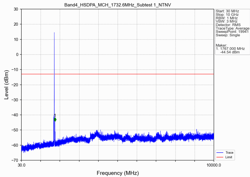
Band4_HSDPA_MCH_1732.6MHz_Subtest 1_NTNV
