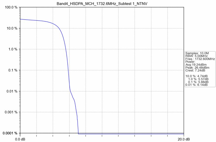
Band4_HSDPA_MCH_1732.6MHz_Subtest 1_NTNV
