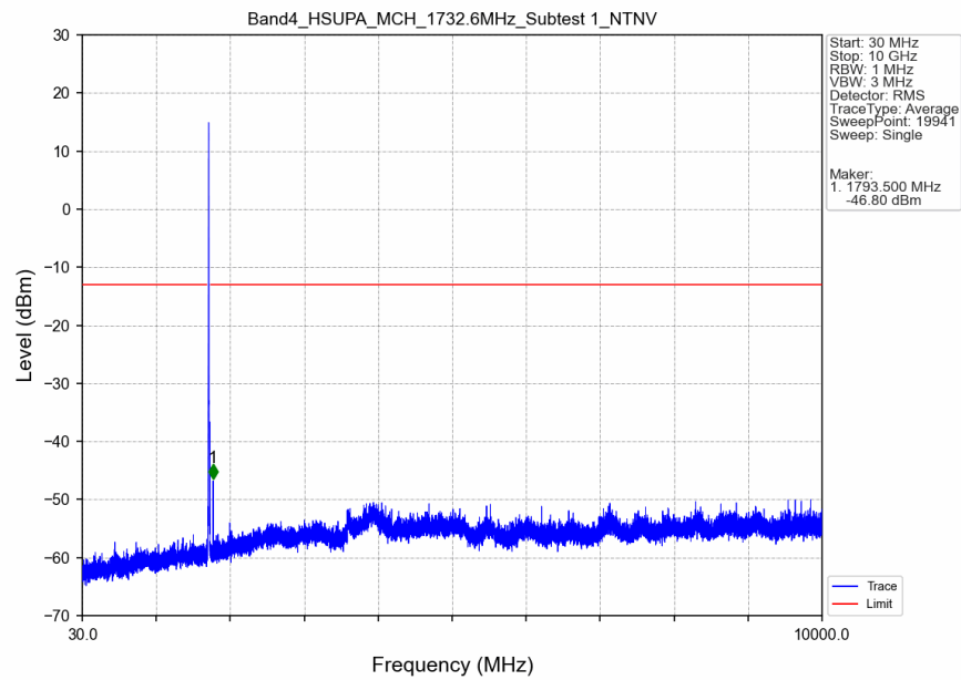
Band4_HSUPA_MCH_1732.6MHz_Subtest 1_NTNV
