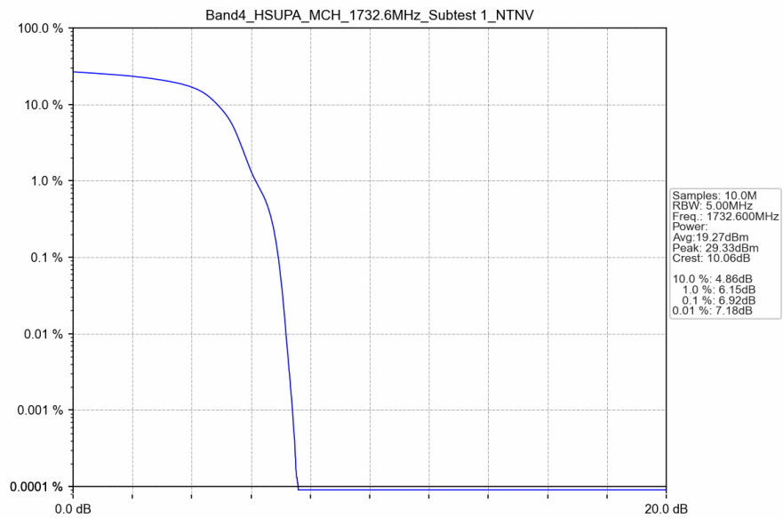
Band4_HSUPA_MCH_1732.6MHz_Subtest 1_NTNV
