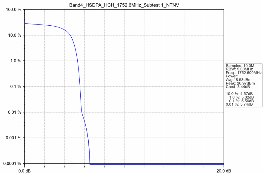
Band4_HSDPA_HCH_1752.6MHz_Subtest 1_NTNV
