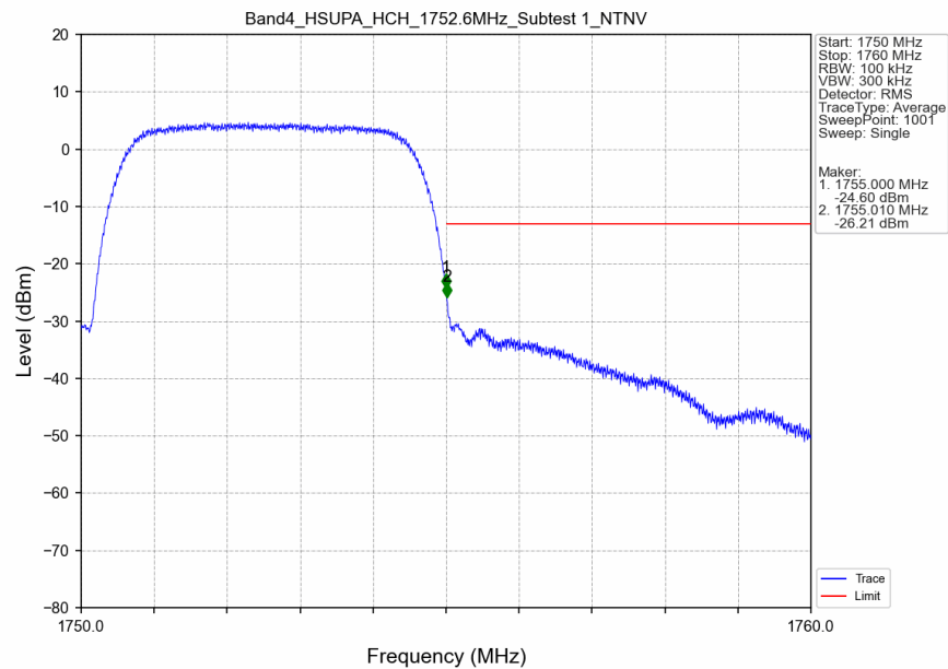
Band4_HSUPA_HCH_1752.6MHz_Subtest 1_NTNV
