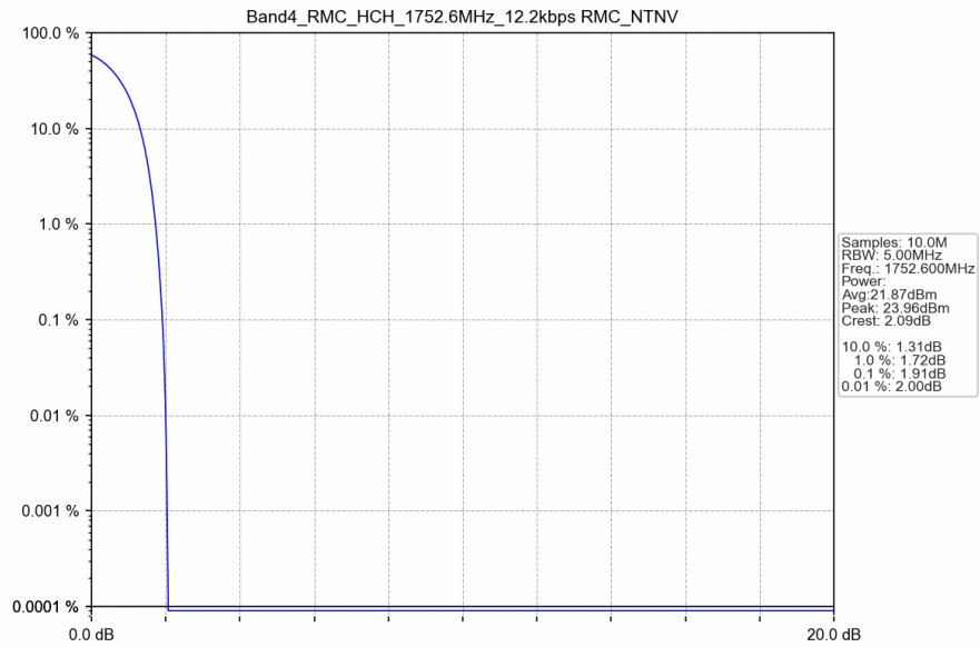
Band4_RMC_HCH_1752.6MHz_12.2kbps RMC_NTNV
