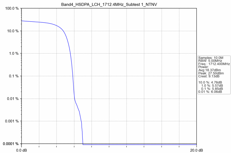
Band4_HSDPA_LCH_1712.4MHz_Subtest 1_NTNV
