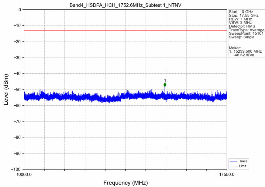
Band4_HSDPA_HCH_1752.6MHz_Subtest 1_NTNV
