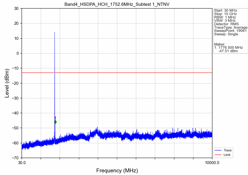
Band4_HSDPA_HCH_1752.6MHz_Subtest 1_NTNV
