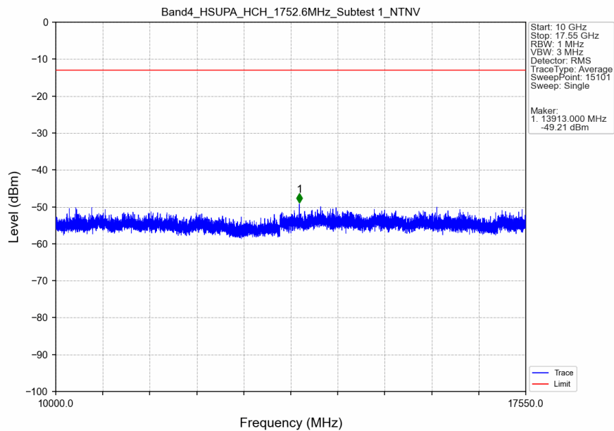
Band4_HSUPA_HCH_1752.6MHz_Subtest 1_NTNV
