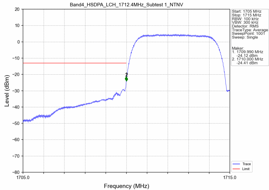
Band4_HSDPA_LCH_1712.4MHz_Subtest 1_NTNV
