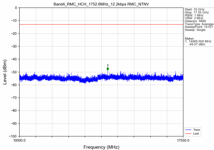
Band4_RMC_HCH_1752.6MHz_12.2kbps RMC_NTNV
