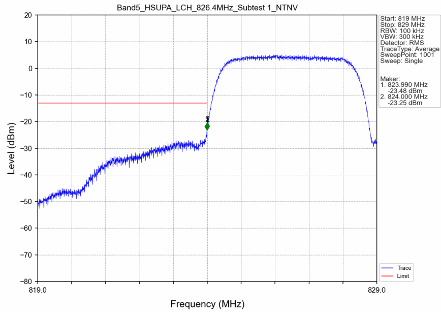
Band5_HSUPA_LCH_826.4MHz_Subtest 1_NTNV
