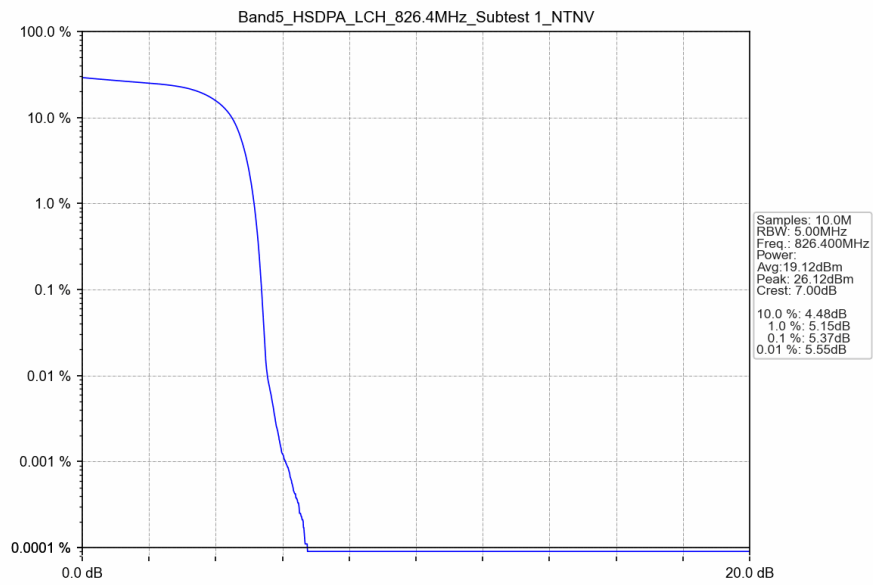
Band5_HSDPA_LCH_826.4MHz_Subtest 1_NTNV
