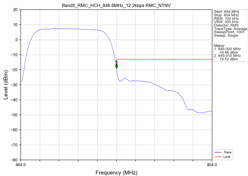
Band5_RMC_HCH_846.6MHz_12.2kbps RMC_NTNV
