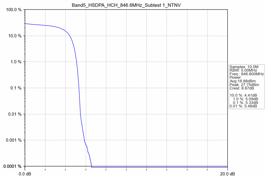
Band5_HSDPA_HCH_846.6MHz_Subtest 1_NTNV
