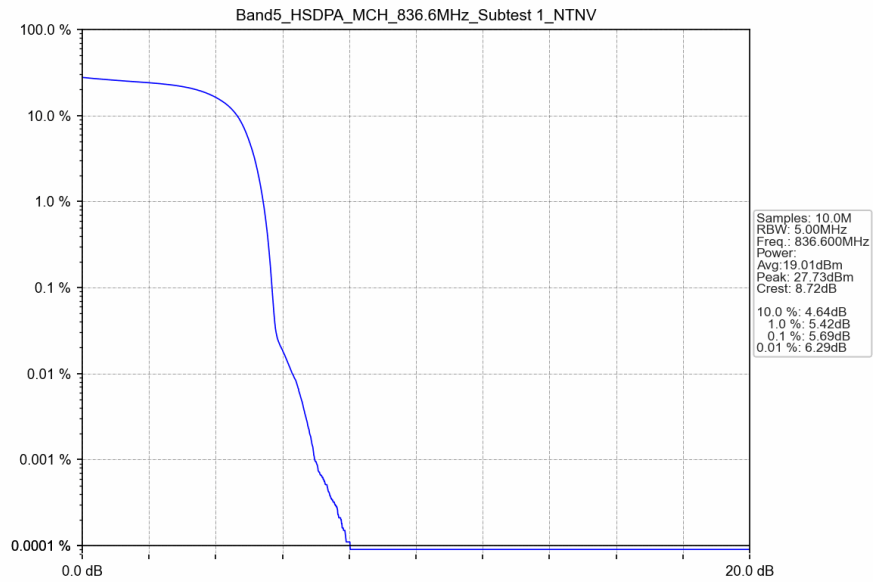
Band5_HSDPA_MCH_836.6MHz_Subtest 1_NTNV
