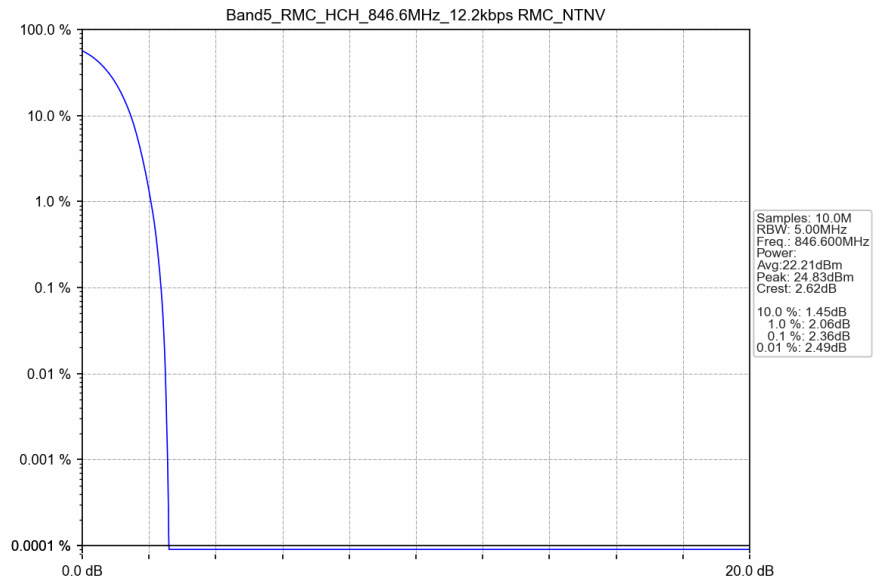
Band5_RMC_HCH_846.6MHz_12.2kbps RMC_NTNV
