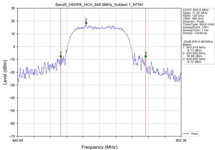
Band5_HSDPA_HCH_846.6MHz_Subtest 1_NTNV
