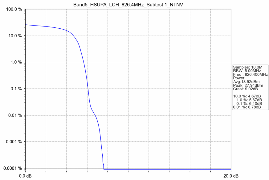
Band5_HSUPA_LCH_826.4MHz_Subtest 1_NTNV
