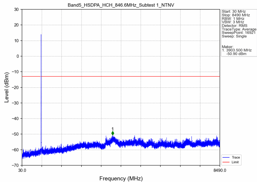
Band5_HSDPA_HCH_846.6MHz_Subtest 1_NTNV
