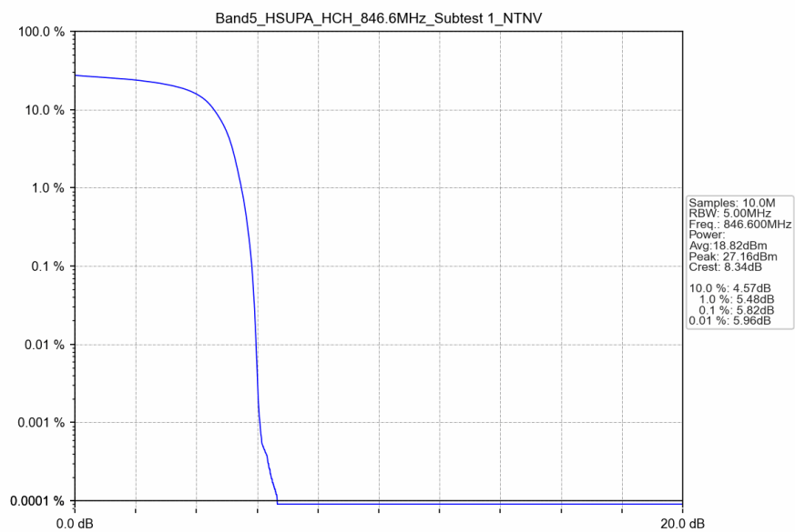
Band5_HSUPA_HCH_846.6MHz_Subtest 1_NTNV
