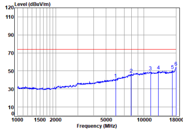
11n_40M_TX_CH_06_Horizontal-Peak
