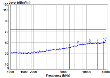
11n_40M_TX_CH_03_Horizontal-Peak
