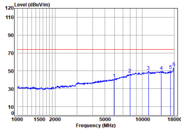
11n_40M_TX_CH_06_Vertical-Peak
