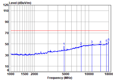
11n_40M_TX_CH_03_Vertical-Peak
