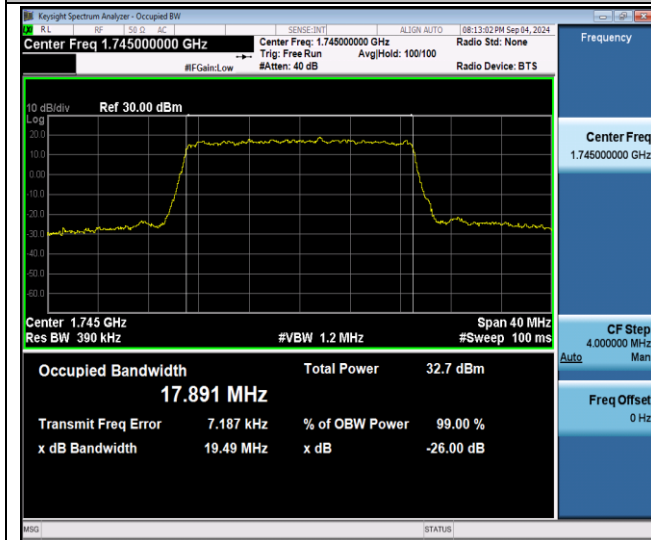
Band4-20MHz-QPSK-20300-100RB#0-PASS
