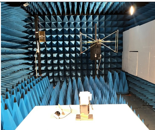
Axis XY on FAR < 1GHz
