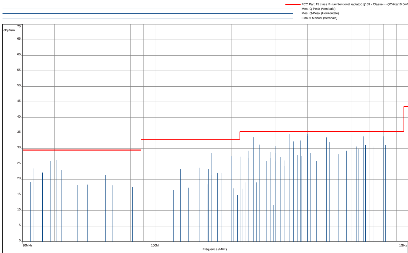
Diagram N°1 Horizontal & vertical Polarization (30MHz-1GHz)
