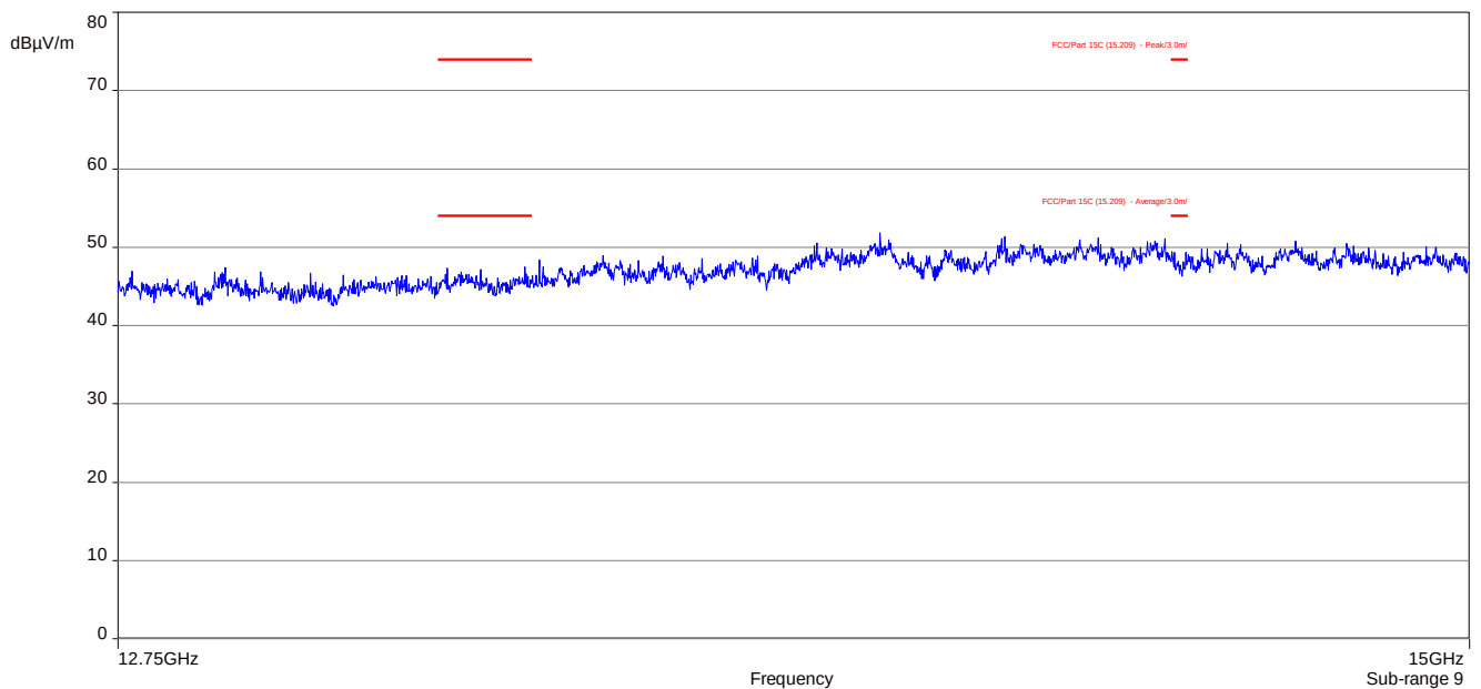
Plot 2: 12.75 GHz to 15 GHz, RX / idle – mode, vertical & horizontal polarization
