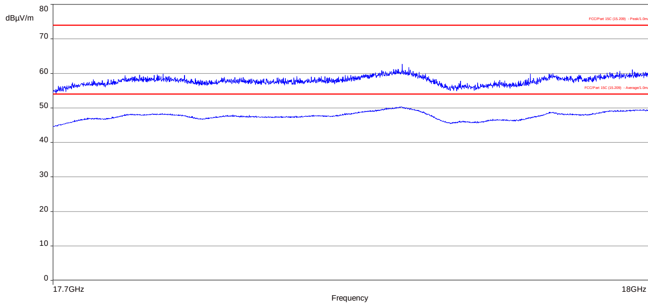
Plot 5: 17.7 GHz to 18 GHz, TX mode, GFSK, channel 39, vertical & horizontal polarization
