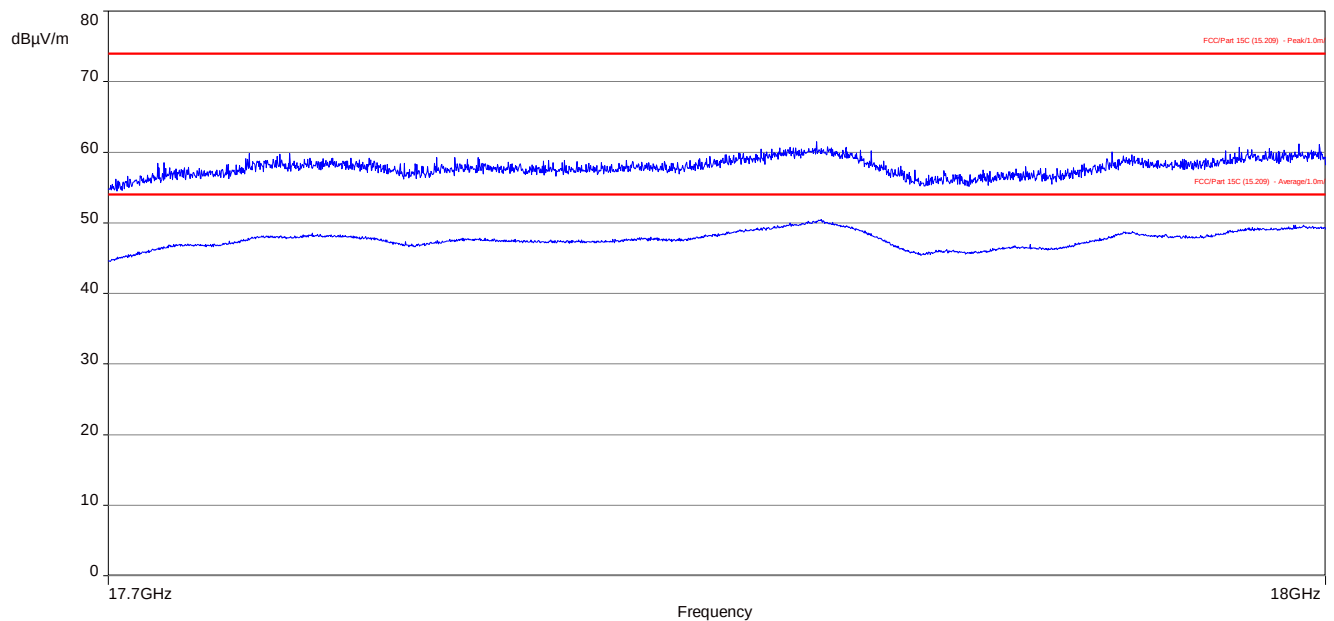
Plot 2: 17.7 GHz to 18 GHz, TX mode, GFSK, channel 00, vertical & horizontal polarization
