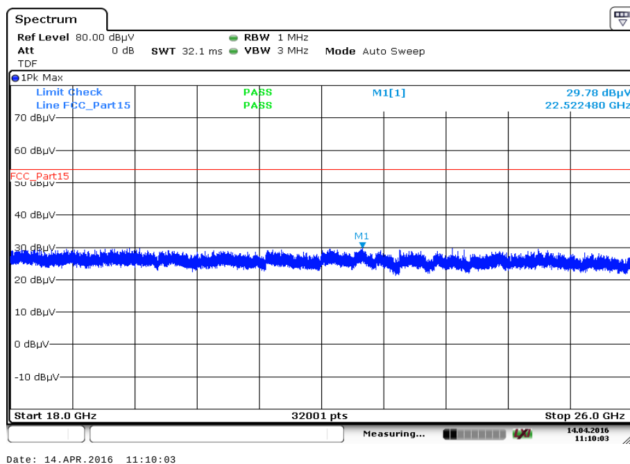
Plot 6: 18 GHz to 26 GHz, TX mode, GFSK, channel 39, vertical & horizontal polarization
