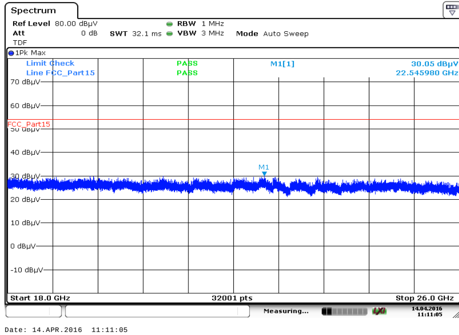
Plot 9: 18 GHz to 26 GHz, TX mode, GFSK, channel 78, vertical & horizontal polarization
