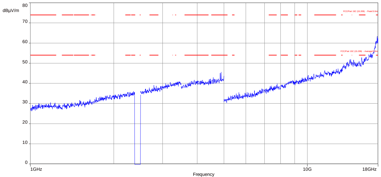
Plot 4: 1 GHz to 18 GHz, TX mode, GFSK, channel 39, vertical & horizontal polarization
