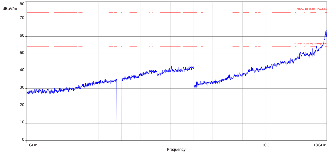
Plot 1: 1 GHz to 18 GHz, TX mode, GFSK, channel 00, vertical & horizontal polarization
