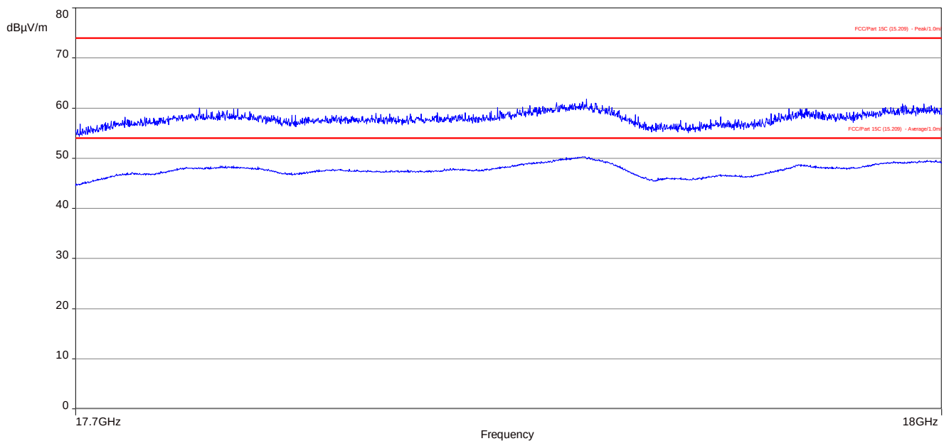
Plot 8: 17.7 GHz to 18 GHz, TX mode, GFSK, channel 78, vertical & horizontal polarization
