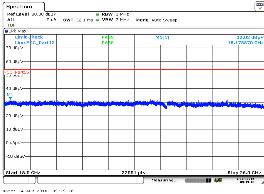
Plot 5: 18 GHz to 26 GHz, RX / idle – mode, vertical & horizontal polarization
