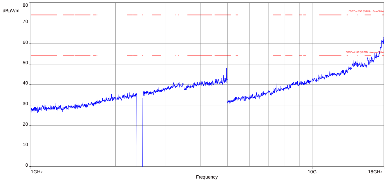
Plot 7: 1 GHz to 18 GHz, TX mode, GFSK, channel 78, vertical & horizontal polarization
