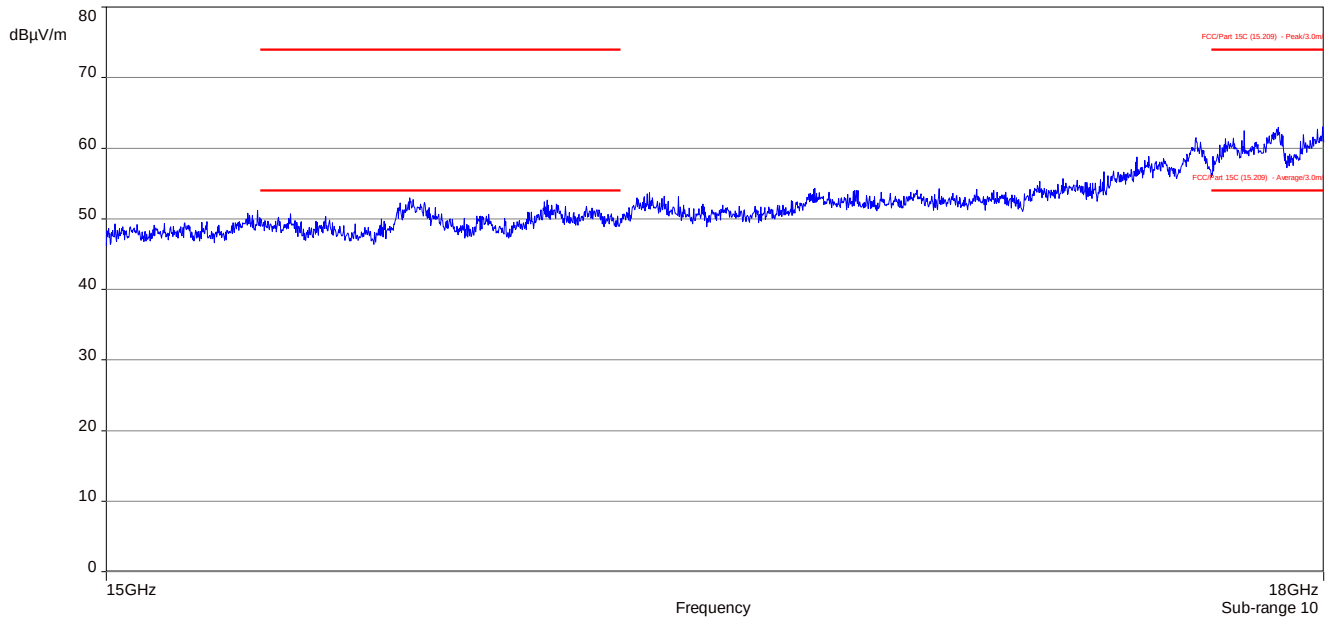
Plot 3: 15 GHz to 18 GHz, RX / idle – mode, vertical & horizontal polarization
