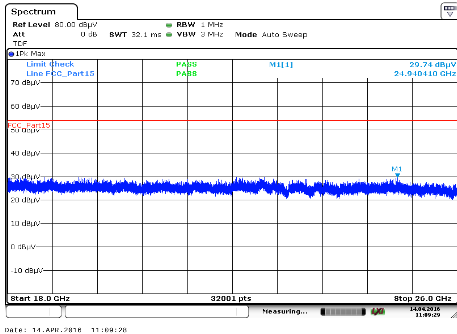
Plot 3: 18 GHz to 26 GHz, TX mode, GFSK, channel 00, vertical & horizontal polarization
