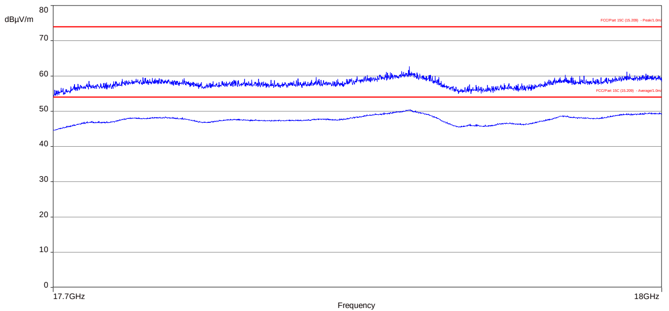
Plot 4: 17.7 GHz to 18 GHz, RX / idle – mode, vertical & horizontal polarization
