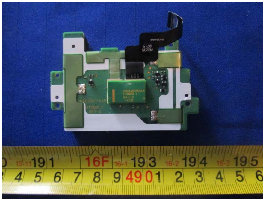
EUT- SCR Board Bottom View
