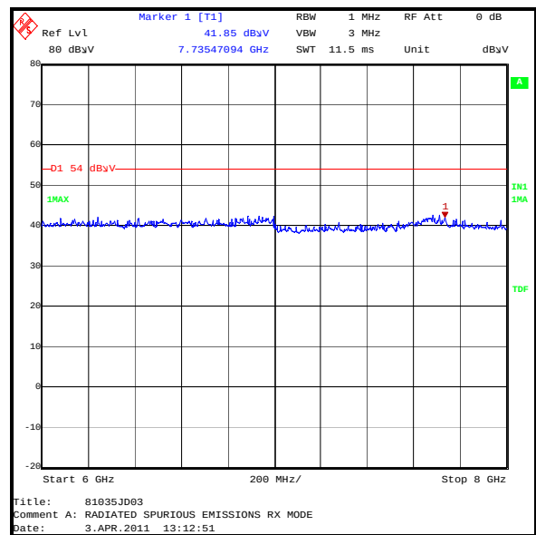
Average
