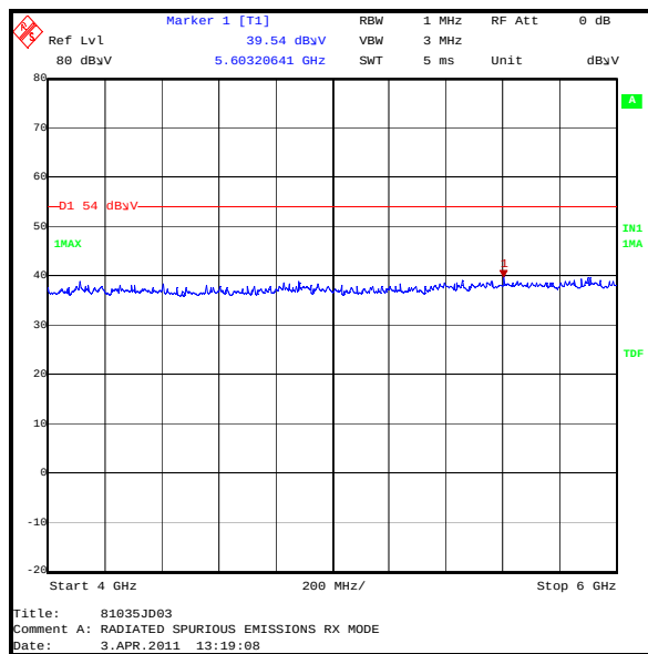
Peak
