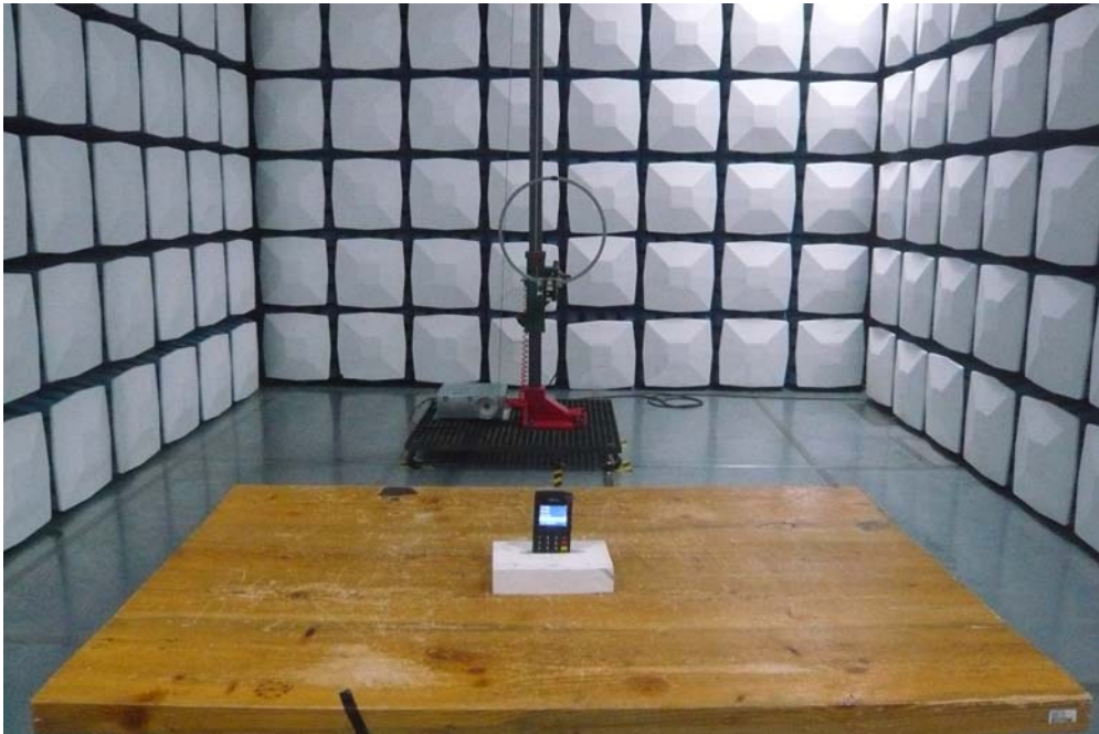
Radiated Emission - View (9 kHz-30 MHz)
