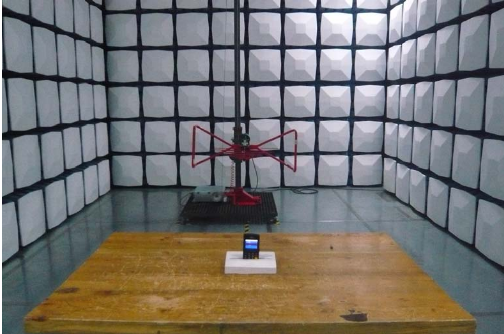
Radiated Emission - View (30 MHz-1GHz)
