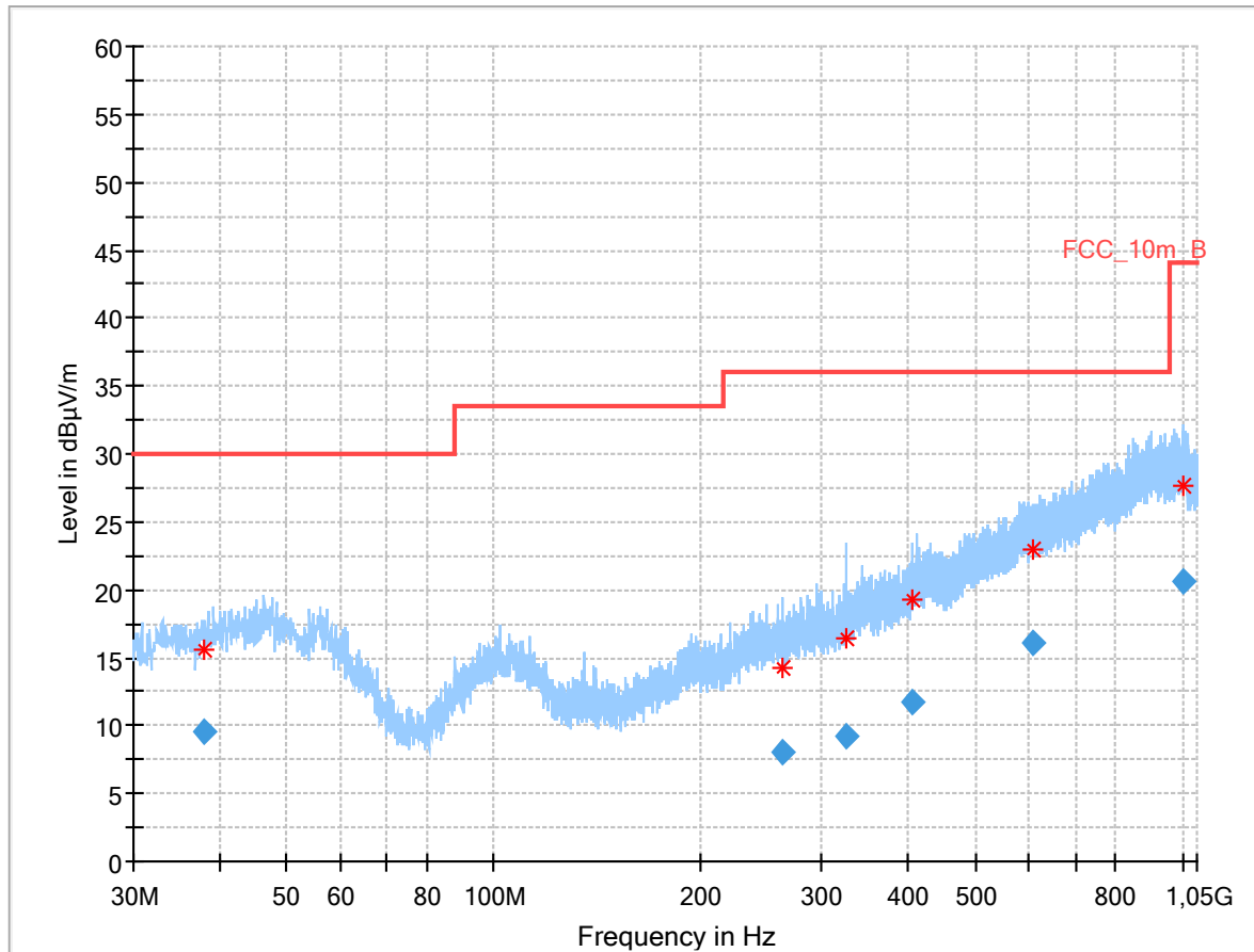
Plot 5: 30 MHz – 1 GHz, vertical and horizontal polarisation
