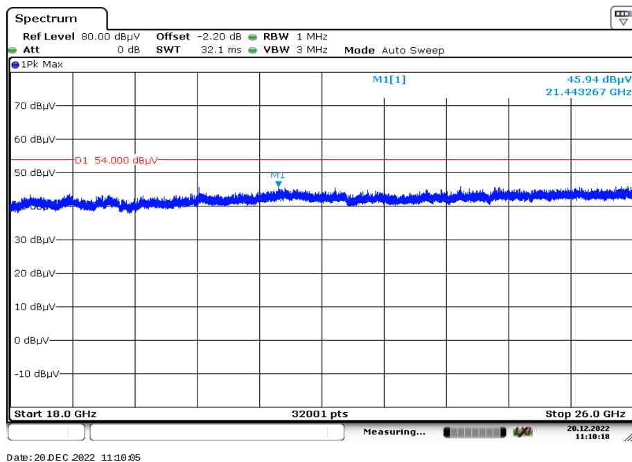
Plot 4: 18 GHz to 26 GHz, TX mode, vertical & horizontal polarization, valid for all channels and modulations
