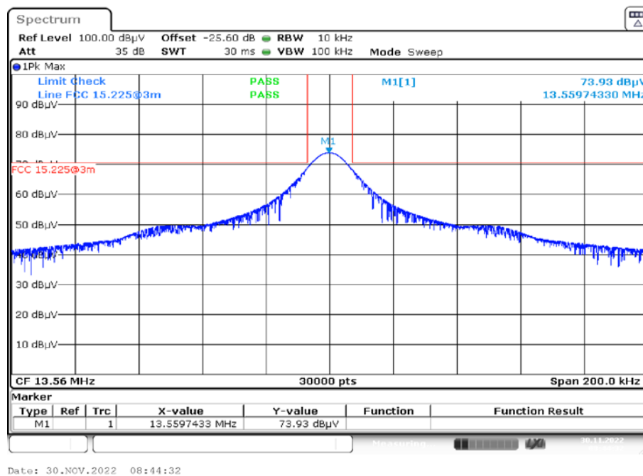
Plot 4: Spectrum mask zoomed
