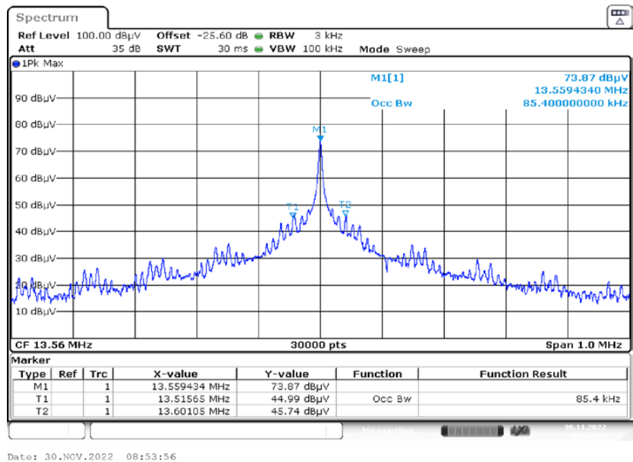
Plot 3: 99 % emission bandwidth mode 3
