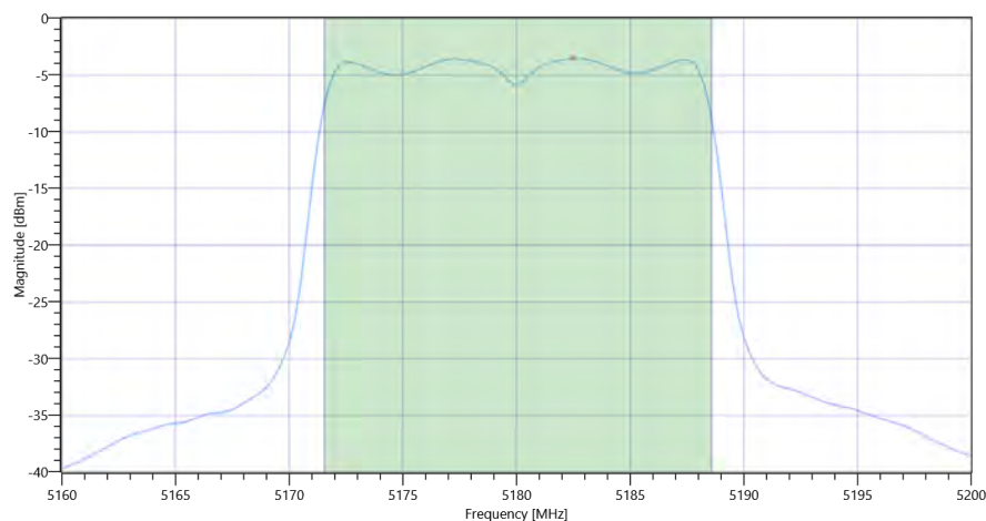
ISSED RSS247 # Max output power and psd ~ WLAN5Gx a mode U-NII-1 Max OP and PSD
