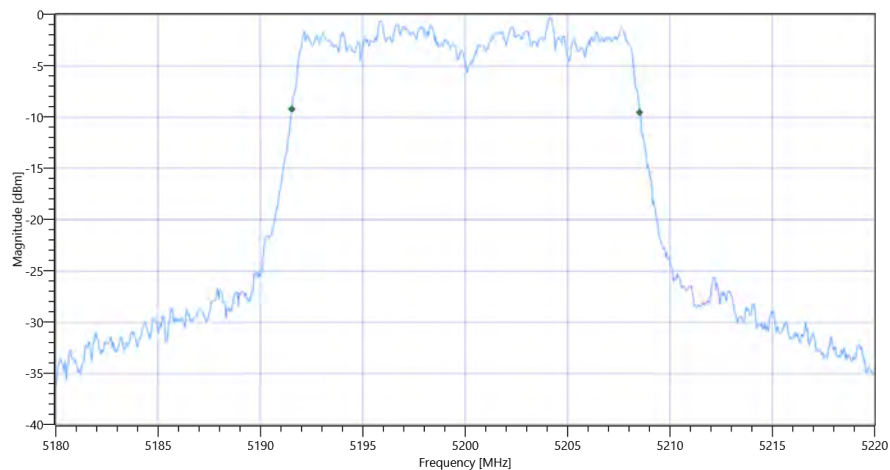
ISSED RSS247 # Max output power and psd ~ WLAN5Gx a mode U-NII-1_BW
