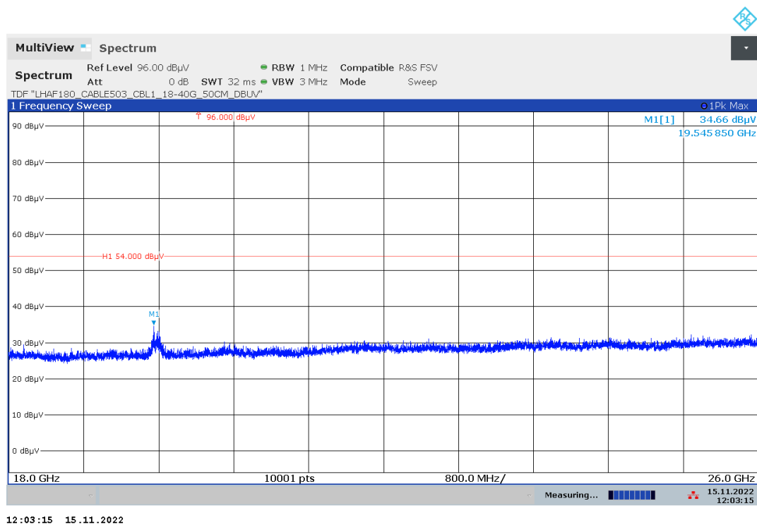
Plot 6: Three channels max hold, 18 GHz to 26 GHz, vertical & horizontal polarization
