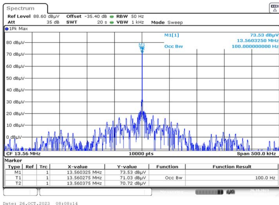
Plot 2: 99 % emission bandwidth ISO 14443 Type B mode
