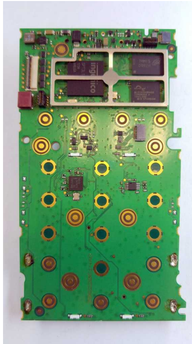
Photo 7: Main UC board Up
