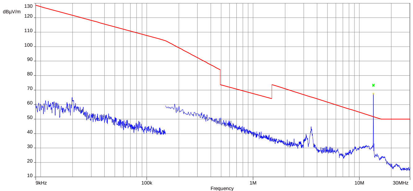
Plot 2: 9 kHz – 30 MHz; magnetic emissions; loop 90°
