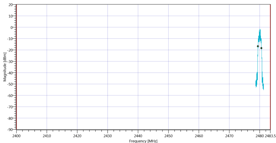
Plot_FCC Part 15.247 Bandwidth 99PCT-20dB ~ BT Classic EDR Pi-4DQPSK_14012020_142227.png
