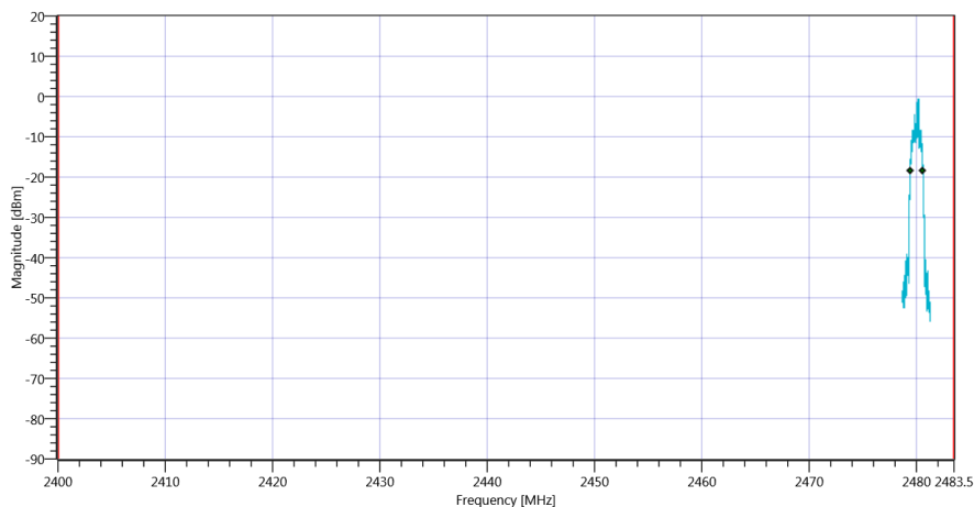
Plot_FCC Part 15.247 Bandwidth 99PCT-20dB ~ BT Classic EDR 8DPSK_14012020_144813.png
