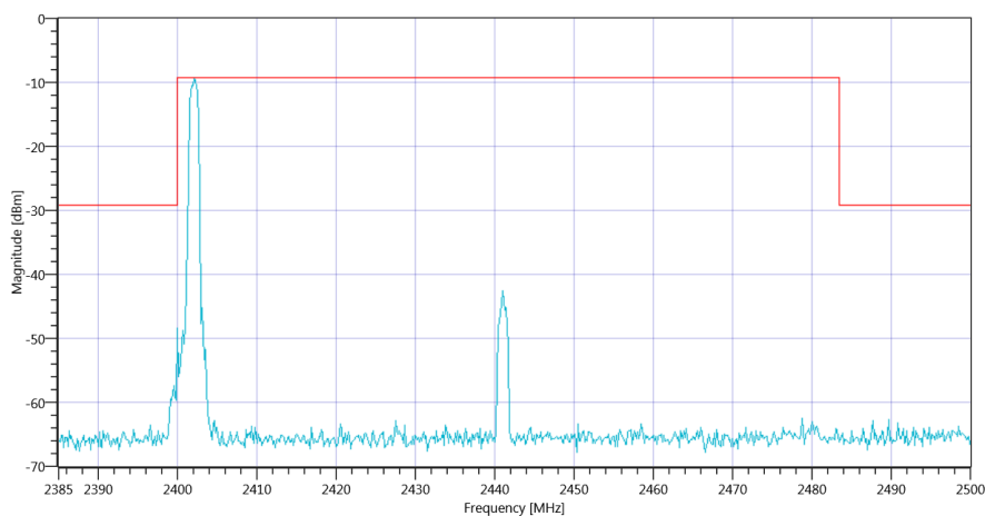
Plot_FCC Part 15.247 TX Spurious Conducted ~ BT Classic EDR Pi-4DQPSK 2402_14012020_141133.png
