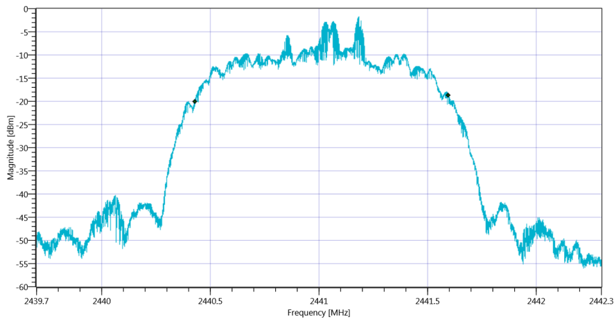
Plot_FCC Part 15.247 Bandwidth 99PCT-20dB ~ BT Classic EDR 8DPSK_14012020_144021.png
