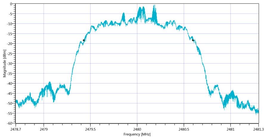
Plot_FCC Part 15.247 Bandwidth 99PCT-20dB ~ BT Classic EDR 8DPSK_99PCT_14012020_144809.png
