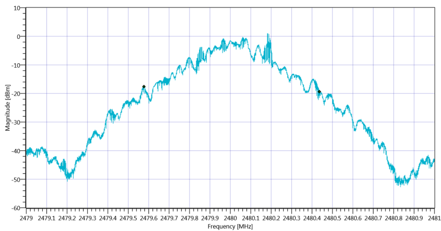
Plot_FCC Part 15.247 Bandwidth 99PCT-20dB ~ BT Classic Basic rate 99PCT_14012020_151303.png
