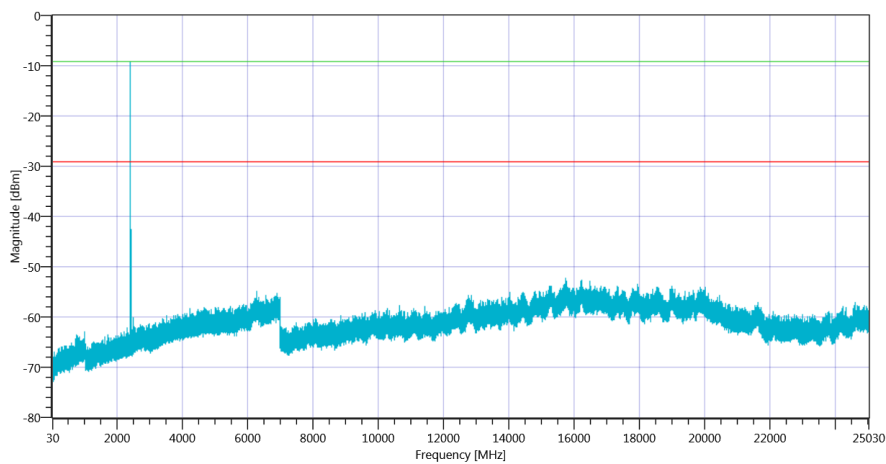
Plot_FCC Part 15.247 TX Spurious Conducted ~ BT Classic EDR Pi-4DQPSK 2402_14012020_141130.png
