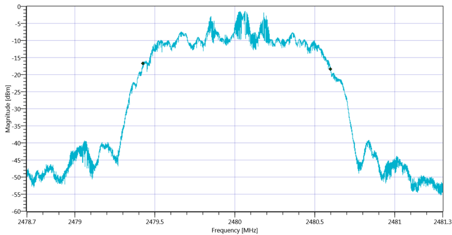
Plot_FCC Part 15.247 Bandwidth 99PCT-20dB ~ BT Classic EDR Pi-4DQPSK 99PCT_14012020_142223.png
