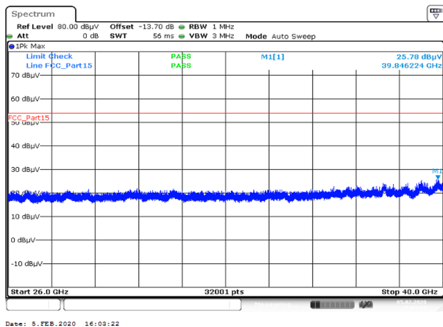
Plot 33: 26 GHz to 40 GHz, 5825 MHz, vertical & horizontal polarization, cabinet radiation
