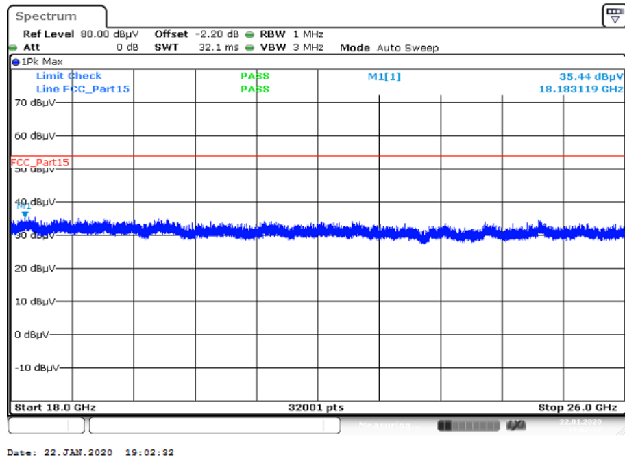
Plot 32: 18 GHz to 26 GHz, 5825 MHz, vertical & horizontal polarization, cabinet radiation
