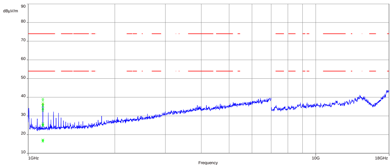
Plot 31: 1 GHz to 18 GHz, 5825 MHz, vertical & horizontal polarization, cabinet radiation
