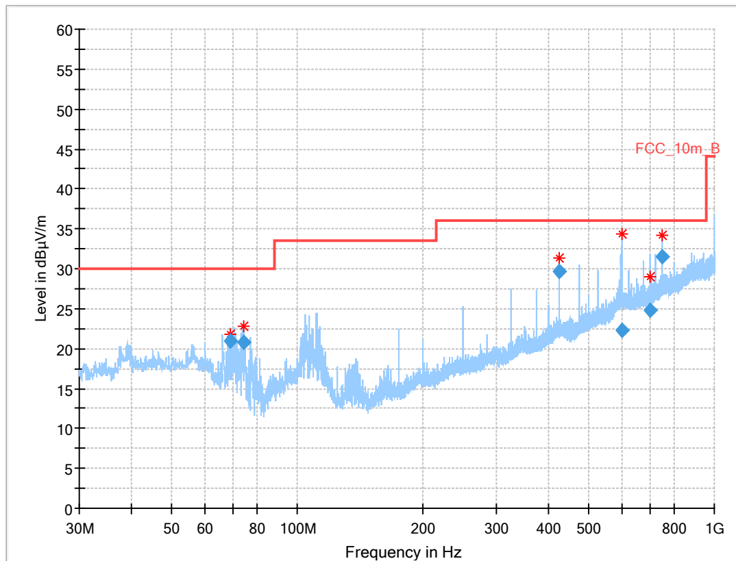
Plot 13: 30 MHz to 1 GHz, cabinet radiation, vertical & horizontal polarization
