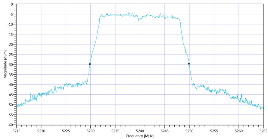
Plot_FCC Part 15.407 & ISM Bandwidths ~ WLAN5Gx a mode U-NII-1 26dB_15012020_151713.png
