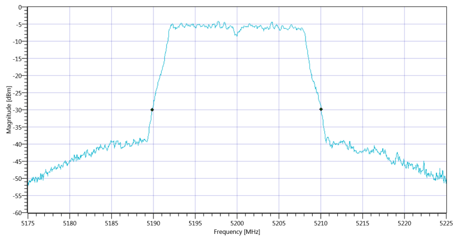
Plot_FCC Part 15.407 & ISSED Bandwidths ~ WLAN5Gx a mode U-NII-1 26dB_15012020_151400.png
