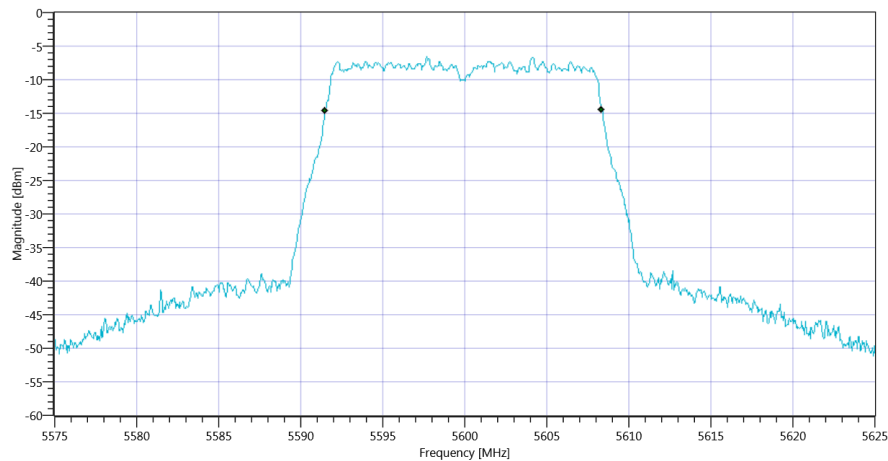
Plot_FCC Part 15.407 & ISM Bandwidths ~ WLAN5Gx a mode U-NII-2C 99PCT_15012020_154359.png
