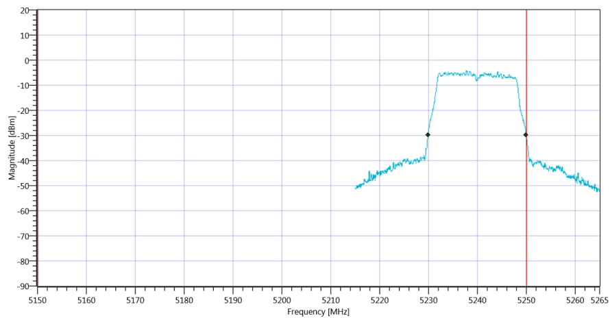
Plot_FCC Part 15.407 & ISM Bandwidths ~ WLAN5Gx a mode U-NII-1_15012020_151717.png
