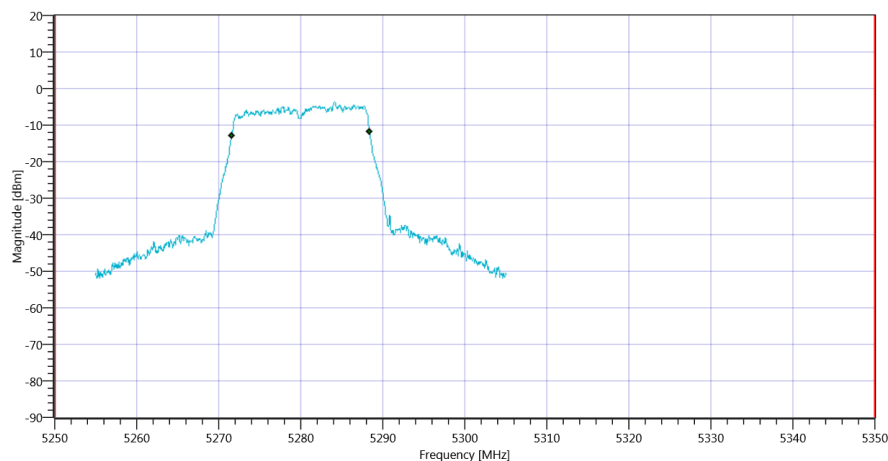
Plot_FCC Part 15.407 & ISSED Bandwidths ~ WLAN5Gx a mode U-NII-2A_15012020_153306.png
