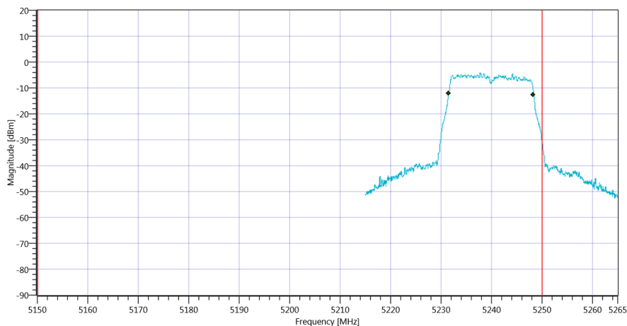
Plot_FCC Part 15.407 & ISCED Bandwidths ~ WLAN5Gx a mode U-NII-1_15012020_151708.png
