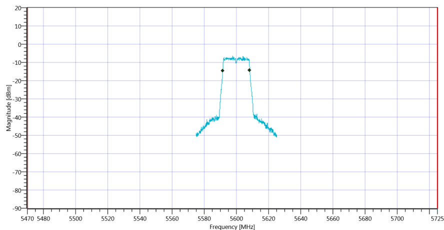
Plot_FCC Part 15.407 & ISM Bandwidths ~ WLAN5Gx a mode U-NII-2C_15012020_154403.png
