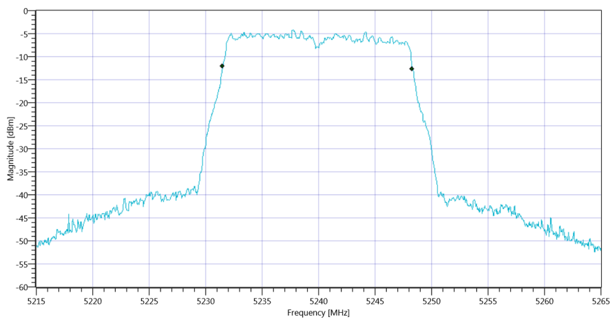
Plot_FCC Part 15.407 & ISCED Bandwidths ~ WLAN5Gx a mode U-NII-1 99PCT_15012020_151704.png
