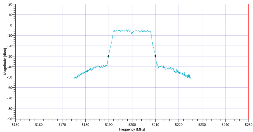
Plot_FCC Part 15.407 & ISSED Bandwidths ~ WLAN5Gx a mode U-NII-1_15012020_151404.png
