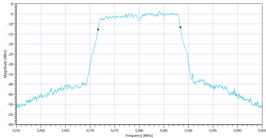
Plot_FCC Part 15.407 & ISSED Bandwidths ~ WLAN5Gx a mode U-NII-2A 99PCT_15012020_153302.png
