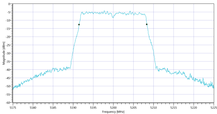
Plot_FCC Part 15.407 & ISSED Bandwidths ~ WLAN5Gx a mode U-NII-1 99PCT_15012020_151351.png
