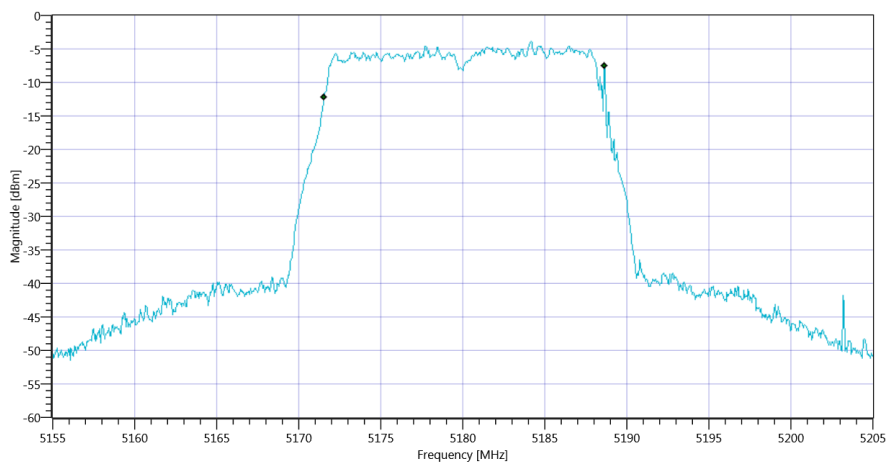
Plot_FCC Part 15.407 & ISCED Bandwidths ~ WLAN5Gx a mode U-NII-1 99PCT_15012020_150213.png
