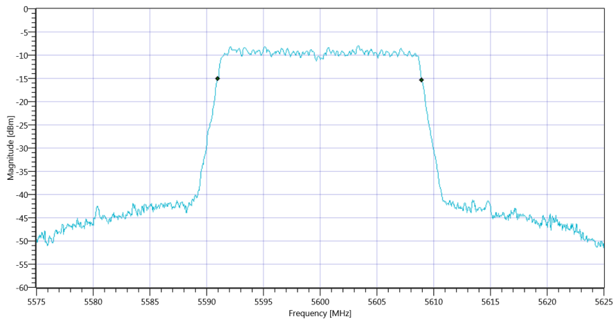
Plot_FCC Part 15.407 & ISSED Bandwidths ~ WLAN5Gx n-HT20 mode U-NII-2C 99PCT_16012020_095401.png
