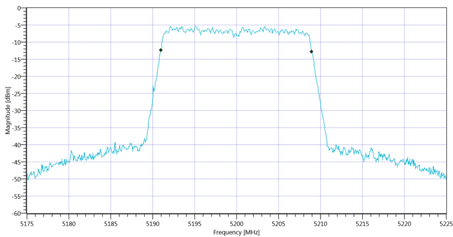
Plot_FCC Part 15.407 & ISCED Bandwidths ~ WLAN5Gx n-HT20 mode U-NII-1 99PCT_16012020_090556.png
