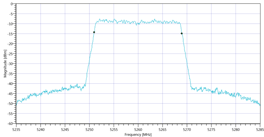
Plot_FCC Part 15.407 & ISSED Bandwidths ~ WLAN5Gx n-HT20 mode U-NII-2A 99PCT_16012020_092231.png
