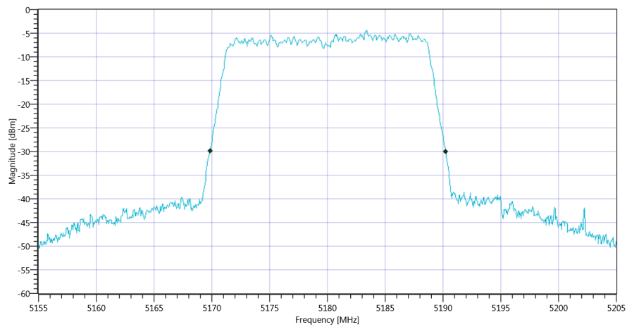
Plot_FCC Part 15.407 & ISSED Bandwidths ~ WLAN5Gx n-HT20 mode U-NII-1 26dB_16012020_090236.png
