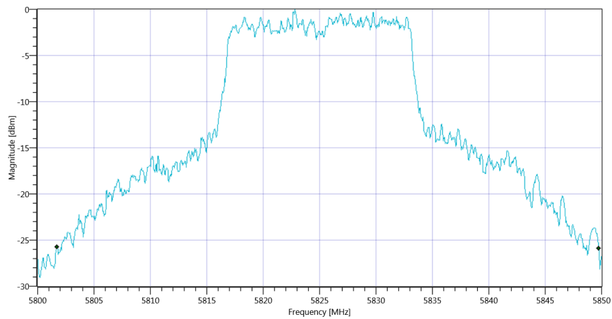
Plot_FCC Part 15.407 & ISM Bandwidths ~ WLAN5Gx a mode U-NII-3 26dB_15012020_161640.png
