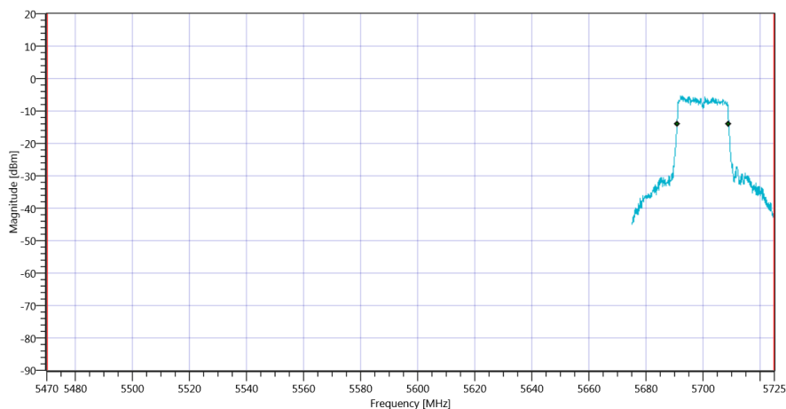
Plot_FCC Part 15.407 & ISSED Bandwidths ~ WLAN5Gx n-HT20 mode U-NII-2C_16012020_100838.png
