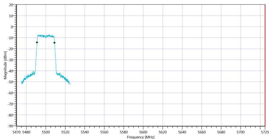
Plot_FCC Part 15.407 & ISSED Bandwidths ~ WLAN5Gx n-HT20 mode U-NII-2C_16012020_094847.png
