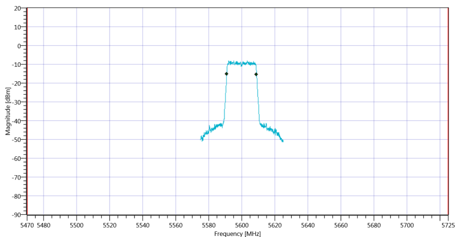
Plot_FCC Part 15.407 & ISSED Bandwidths ~ WLAN5Gx n-HT20 mode U-NII-2C_16012020_095404.png
