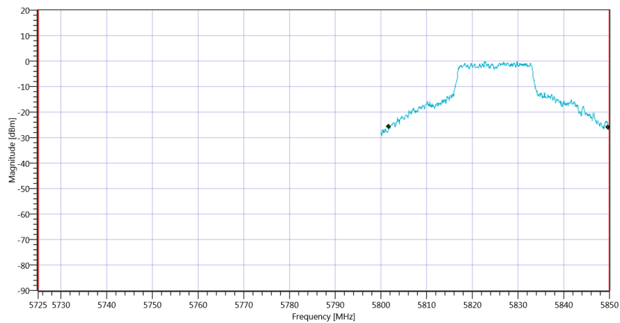
Plot_FCC Part 15.407 & ISM Bandwidths ~ WLAN5Gx a mode U-NII-3_15012020_161644.png
