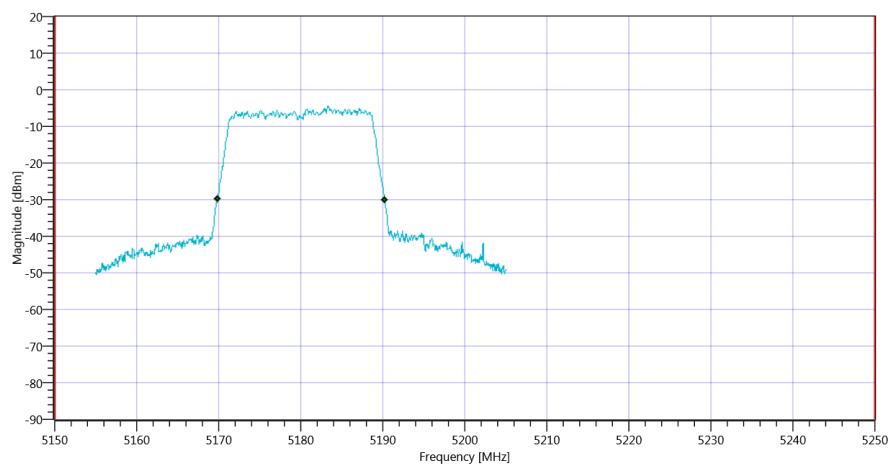
Plot_FCC Part 15.407 & ISSED Bandwidths ~ WLAN5Gx n-HT20 mode U-NII-1_16012020_090240.png
