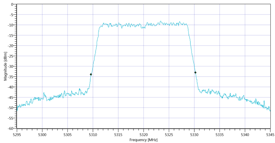
Plot_FCC Part 15.407 & ISSED Bandwidths ~ WLAN5Gx n-HT20 mode U-NII-2A_16012020_094134.png
