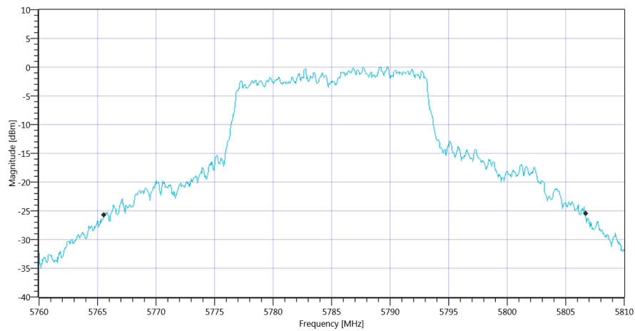
Plot_FCC Part 15.407 & ISSED Bandwidths ~ WLAN5Gx a mode U-NII-3 26dB_15012020_155750.png
