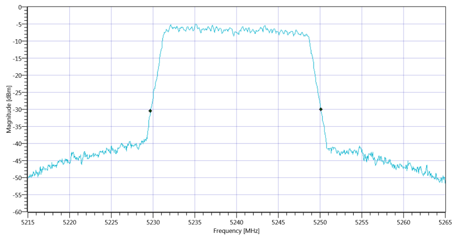
Plot_FCC Part 15.407 & ISSED Bandwidths ~ WLAN5Gx n-HT20 mode U-NII-1 26dB_16012020_091307.png
