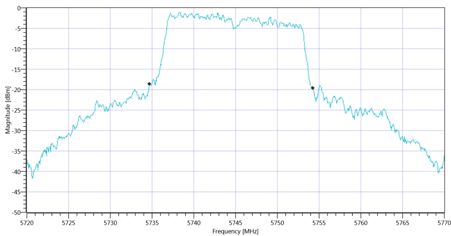
Plot_FCC Part 15.407 & ISM Bandwidths ~ WLAN5Gx a mode U-NII-3 99PCT_15012020_155205.png
