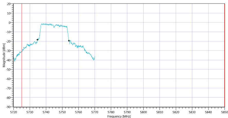
Plot_FCC Part 15.407 & ISM Bandwidths ~ WLAN5Gx a mode U-NII-3_15012020_155210.png
