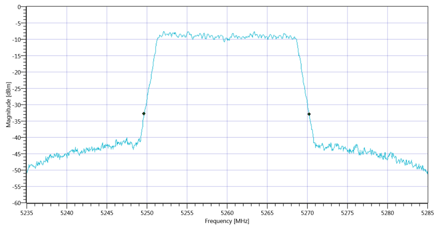
Plot_FCC Part 15.407 & ISSED Bandwidths ~ WLAN5Gx n-HT20 mode U-NII-2A 26dB_16012020_092242.png
