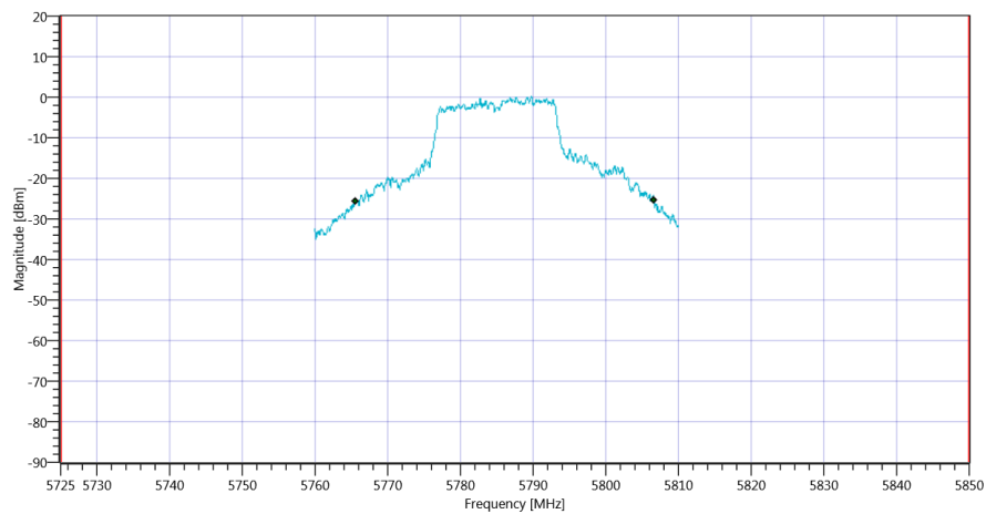
Plot_FCC Part 15.407 & ISSED Bandwidths ~ WLAN5Gx a mode U-NII-3_15012020_155754.png
