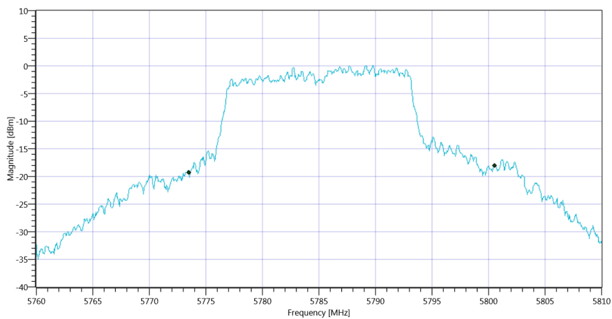
Plot_FCC Part 15.407 & ISM Bandwidths ~ WLAN5Gx a mode U-NII-3 99PCT_15012020_155737.png
