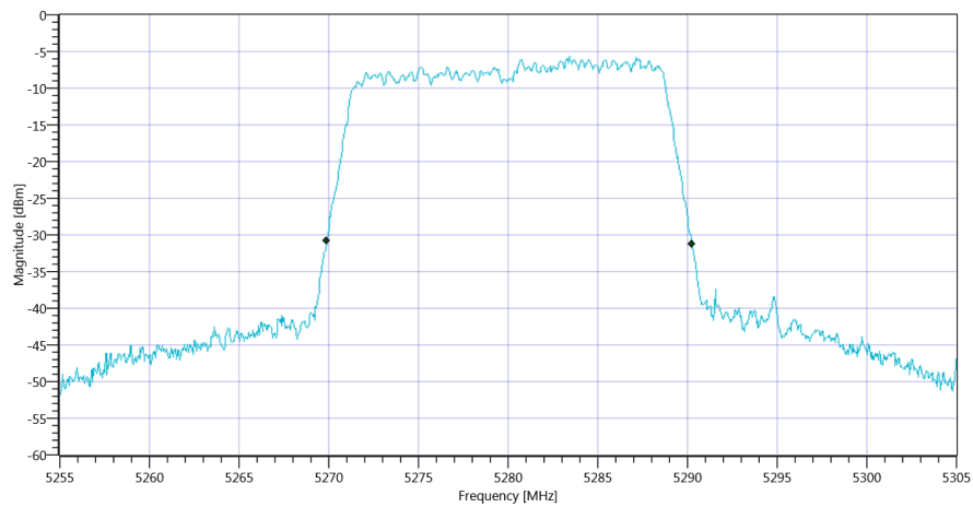
Plot_FCC Part 15.407 & ISSED Bandwidths ~ WLAN5Gx n-HT20 mode U-NII-2A_16012020_092802.png
