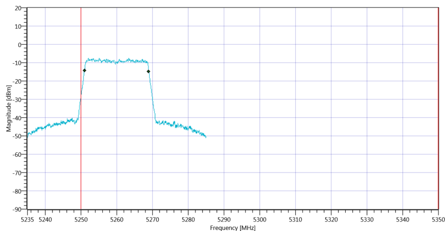
Plot_FCC Part 15.407 & ISSED Bandwidths ~ WLAN5Gx n-HT20 mode U-NII-2A_16012020_092235.png
