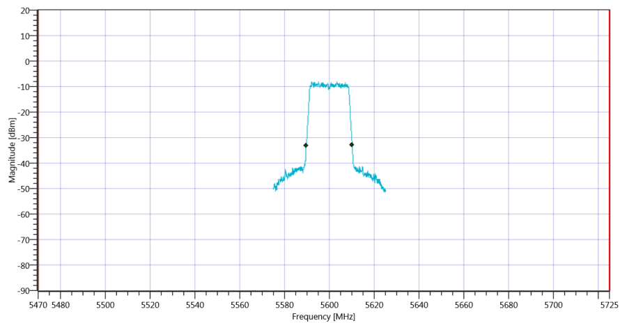
Plot_FCC Part 15.407 & ISSED Bandwidths ~ WLAN5Gx n-HT20 mode U-NII-2C_16012020_095414.png
