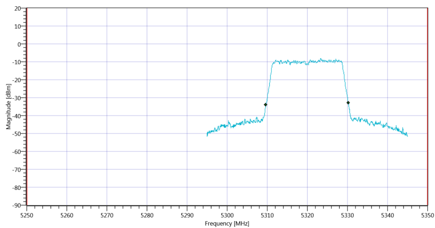
Plot_FCC Part 15.407 & ISSED Bandwidths ~ WLAN5Gx n-HT20 mode U-NII-2A_16012020_094137.png
