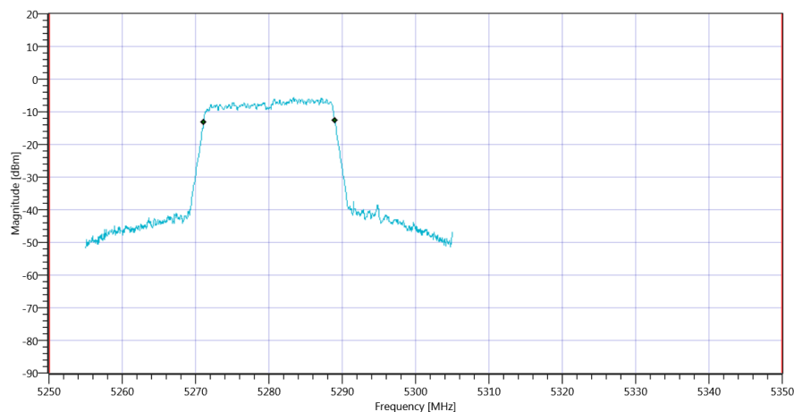
Plot_FCC Part 15.407 & ISSED Bandwidths ~ WLAN5Gx n-HT20 mode U-NII-2A_16012020_092757.png
