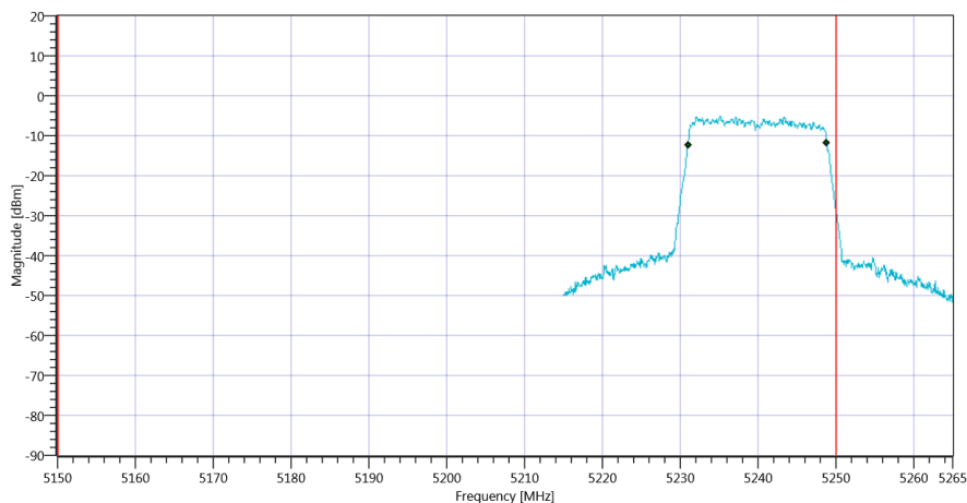
Plot_FCC Part 15.407 & ISCED Bandwidths ~ WLAN5Gx n-HT20 mode U-NII-1_16012020_091301.png
