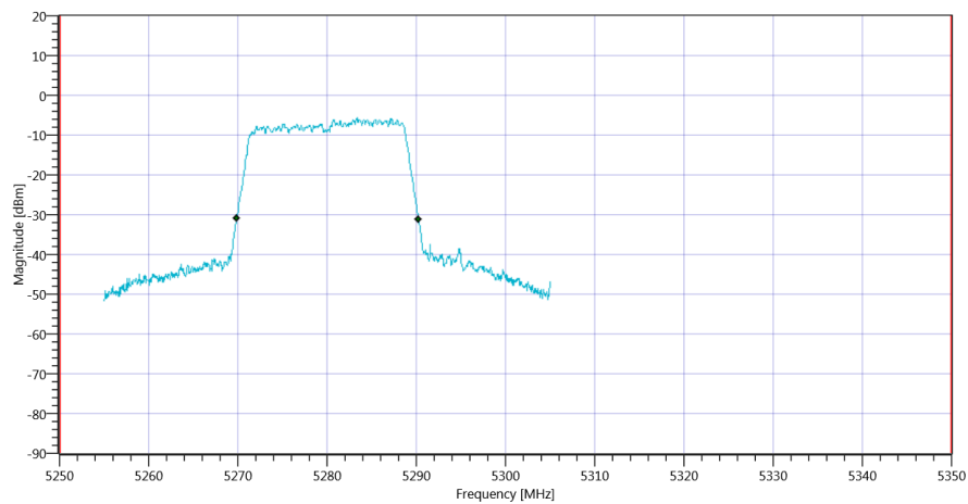
Plot_FCC Part 15.407 & ISSED Bandwidths ~ WLAN5Gx n-HT20 mode U-NII-2A_16012020_092806.png
