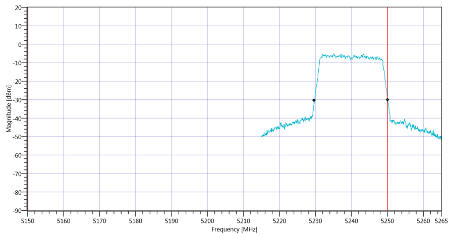
Plot_FCC Part 15.407 & ISSED Bandwidths ~ WLAN5Gx n-HT20 mode U-NII-1_16012020_091311.png
