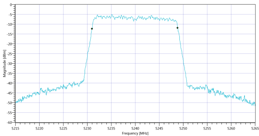
Plot_FCC Part 15.407 & ISCED Bandwidths ~ WLAN5Gx n-HT20 mode U-NII-1 99PCT_16012020_091258.png
