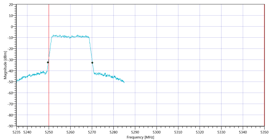
Plot_FCC Part 15.407 & ISSED Bandwidths ~ WLAN5Gx n-HT20 mode U-NII-2A_16012020_092246.png
