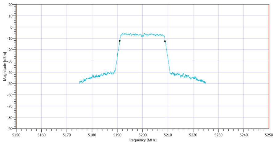
Plot_FCC Part 15.407 & ISCED Bandwidths ~ WLAN5Gx n-HT20 mode U-NII-1_16012020_090600.png
