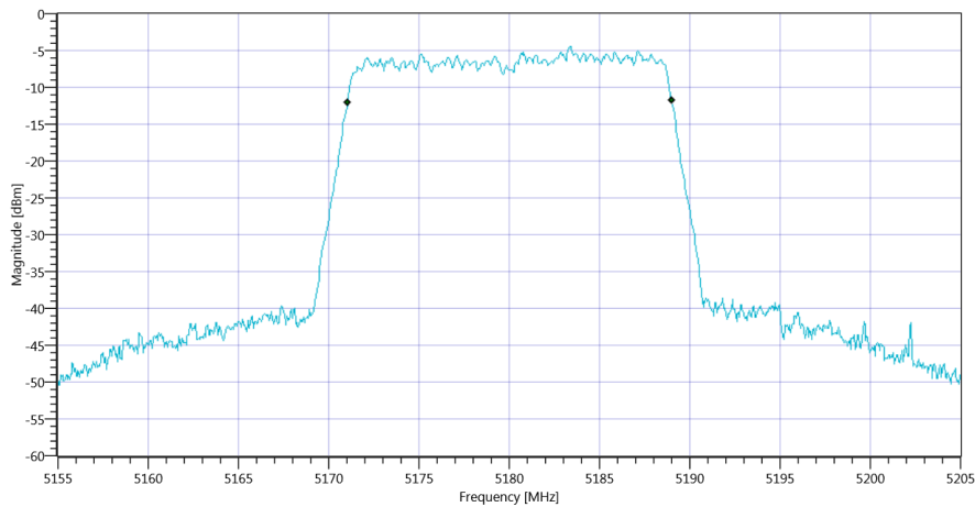
Plot_FCC Part 15.407 & ISCED Bandwidths ~ WLAN5Gx n-HT20 mode U-NII-1 99PCT_16012020_090227.png
