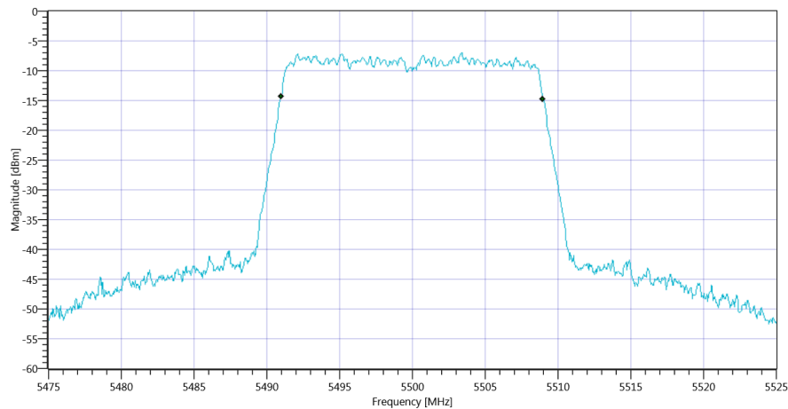
Plot_FCC Part 15.407 & ISSED Bandwidths ~ WLAN5Gx n-HT20 mode U-NII-2C 99PCT_16012020_094842.png
