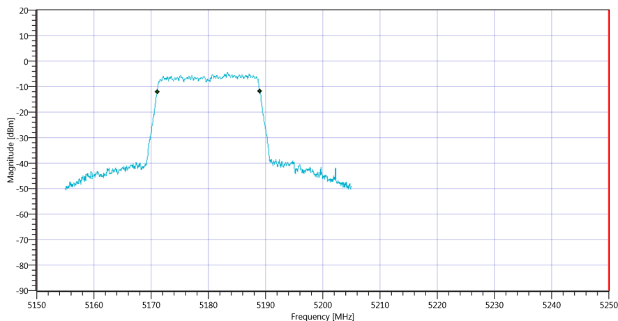
Plot_FCC Part 15.407 & ISCED Bandwidths ~ WLAN5Gx n-HT20 mode U-NII-1_16012020_090231.png
