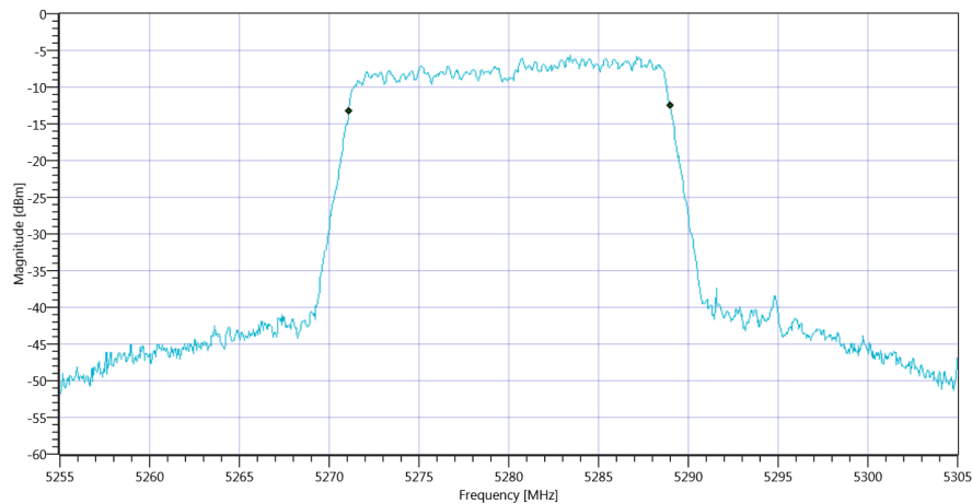
Plot_FCC Part 15.407 & ISSED Bandwidths ~ WLAN5Gx n-HT20 mode U-NII-2A 99PCT_16012020_092753.png
