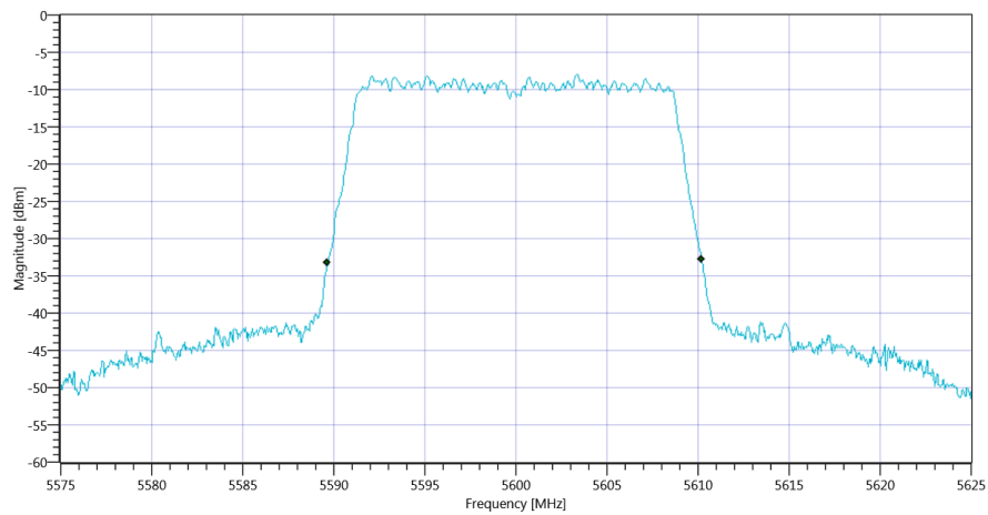
Plot_FCC Part 15.407 & ISSED Bandwidths ~ WLAN5Gx n-HT20 mode U-NII-2C 26dB_16012020_095410.png
