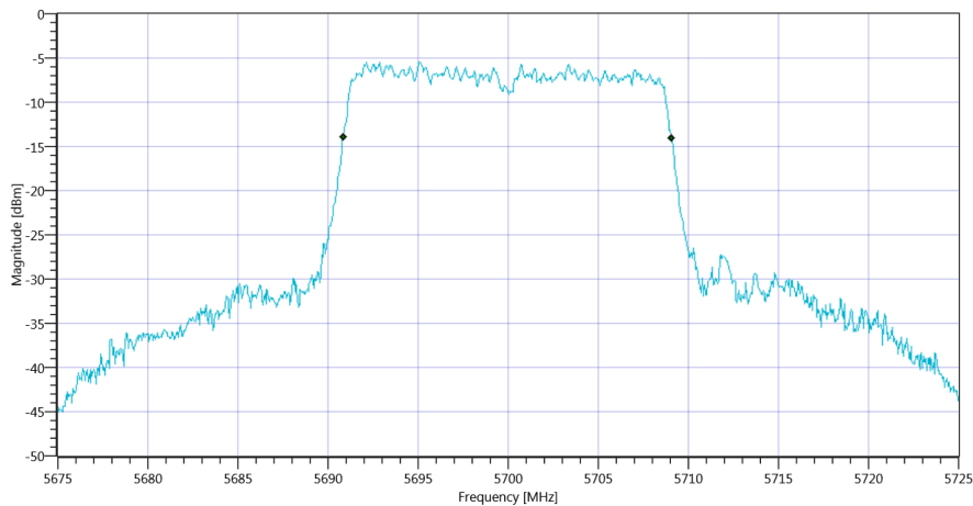
Plot_FCC Part 15.407 & ISSED Bandwidths ~ WLAN5Gx n-HT20 mode U-NII-2C 99PCT_16012020_100834.png
