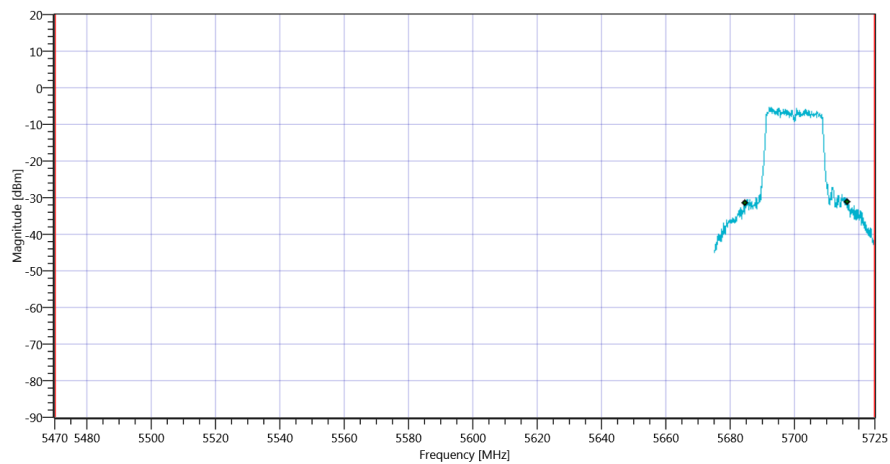
Plot_FCC Part 15.407 & ISSED Bandwidths ~ WLAN5Gx n-HT20 mode U-NII-2C_16012020_100847.png
