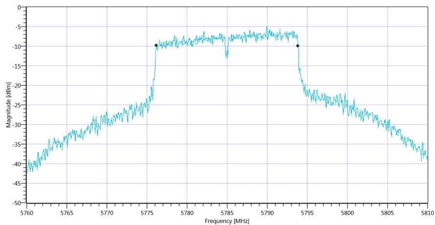
Plot_FCC Part 15.407 & ISSED Minimum Emission BW ~ WLAN5Gx n-HT20 mode U-NII-3_16012020_102610.png
