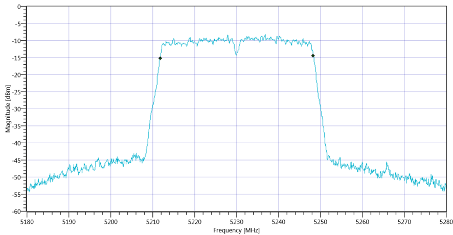
Plot_FCC Part 15.407 & ISCED Bandwidths ~ WLAN5Gx n-HT40 mode U-NII-1 99PCT_16012020_111453.png
