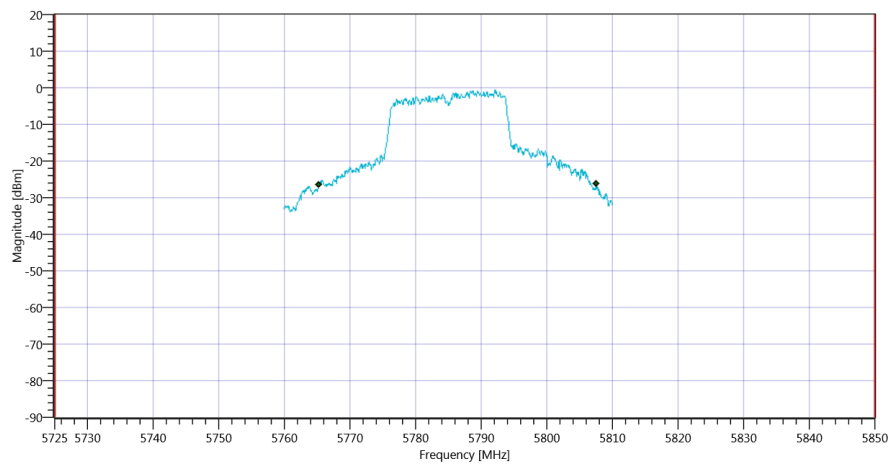
Plot_FCC Part 15.407 & ISSED Bandwidths ~ WLAN5Gx n-HT20 mode U-NII-3_16012020_102520.png
