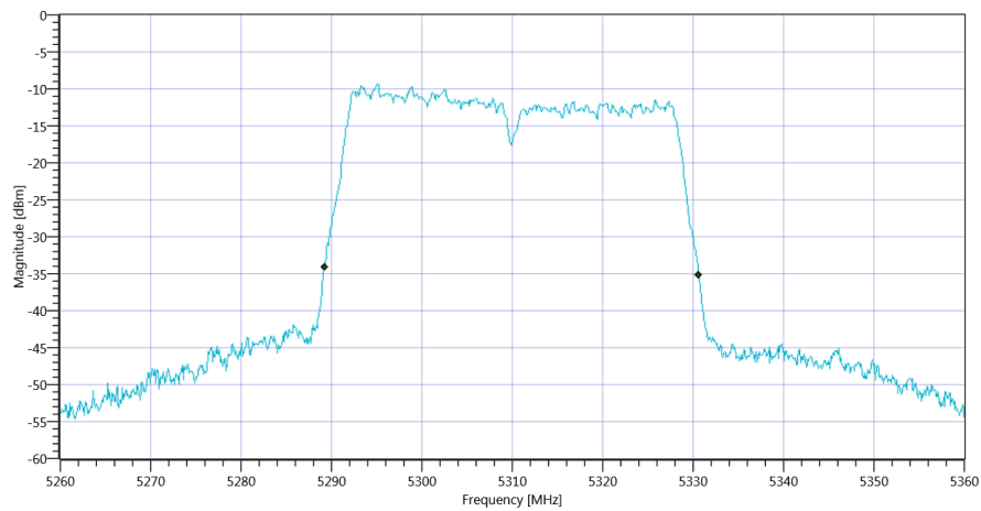
Plot_FCC Part 15.407 & ISM Bandwidths ~ WLAN5Gx n-HT40 mode U-NII-2A_16012020_115315.png
