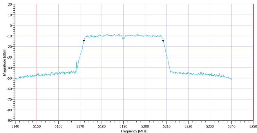
Plot_FCC Part 15.407 & ISCED Bandwidths ~ WLAN5Gx n-HT40 mode U-NII-1_16012020_104309.png
