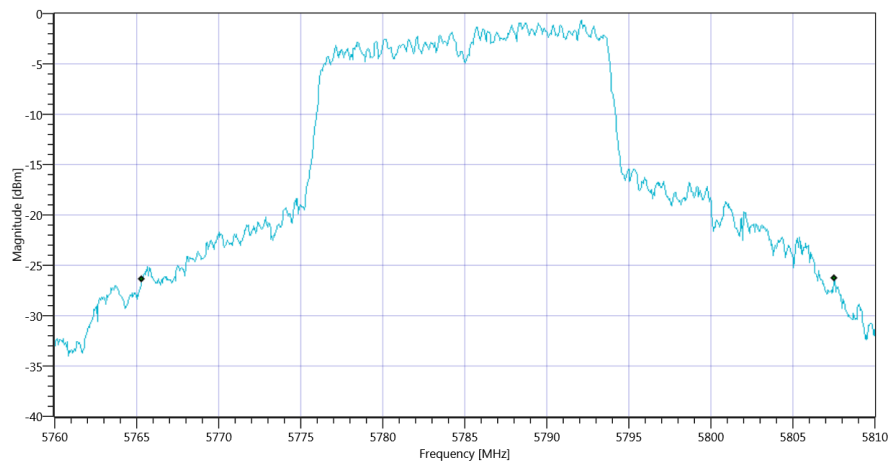
Plot_FCC Part 15.407 & ISSED Bandwidths ~ WLAN5Gx n-HT20 mode U-NII-3 26dB_16012020_102516.png
