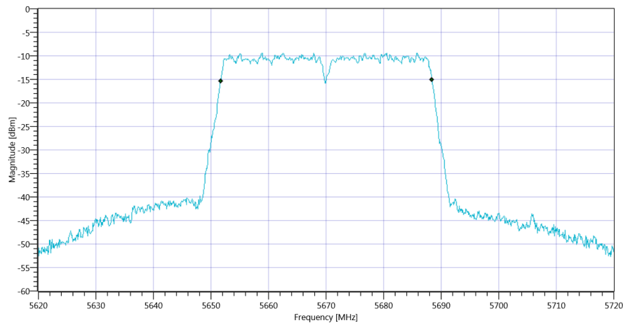
Plot_FCC Part 15.407 & ISSED Bandwidths ~ WLAN5Gx n-HT40 mode U-NII-2C 99PCT_16012020_120729.png
