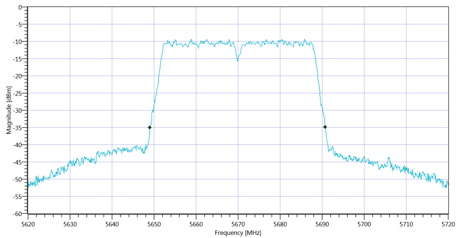
Plot_FCC Part 15.407 & ISM Bandwidths ~ WLAN5Gx n-HT40 mode U-NII-2C 26dB_16012020_120738.png
