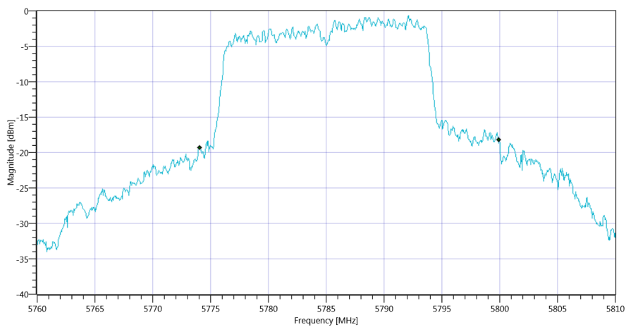
Plot_FCC Part 15.407 & ISCED Bandwidths ~ WLAN5Gx n-HT20 mode U-NII-3 99PCT_16012020_102507.png
