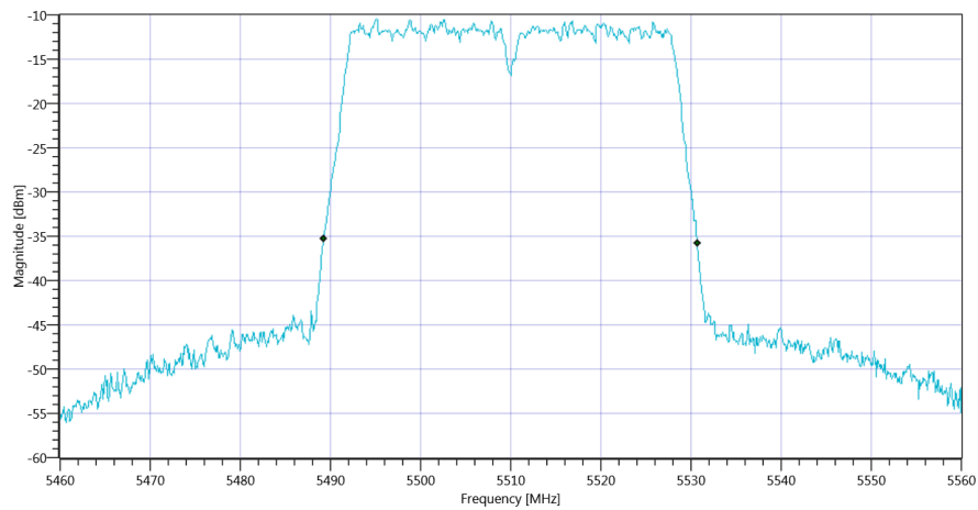
Plot_FCC Part 15.407 & ISSED Bandwidths ~ WLAN5Gx n-HT40 mode U-NII-2C 26dB_16012020_115834.png
