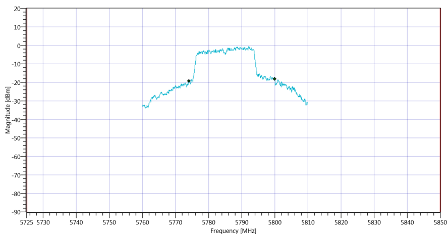
Plot_FCC Part 15.407 & ISCED Bandwidths ~ WLAN5Gx n-HT20 mode U-NII-3_16012020_102511.png
