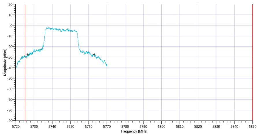
Plot_FCC Part 15.407 & ISSED Bandwidths ~ WLAN5Gx n-HT20 mode U-NII-3_16012020_101457.png
