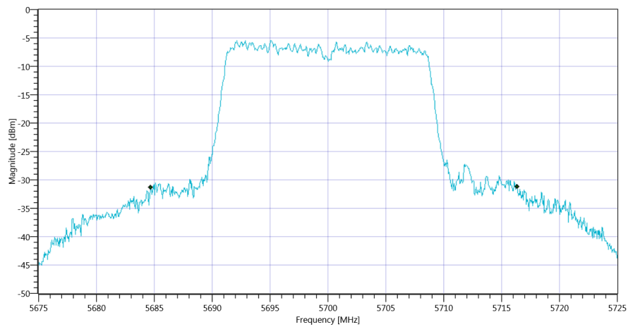
Plot_FCC Part 15.407 & ISSED Bandwidths ~ WLAN5Gx n-HT20 mode U-NII-2C 26dB_16012020_100843.png
