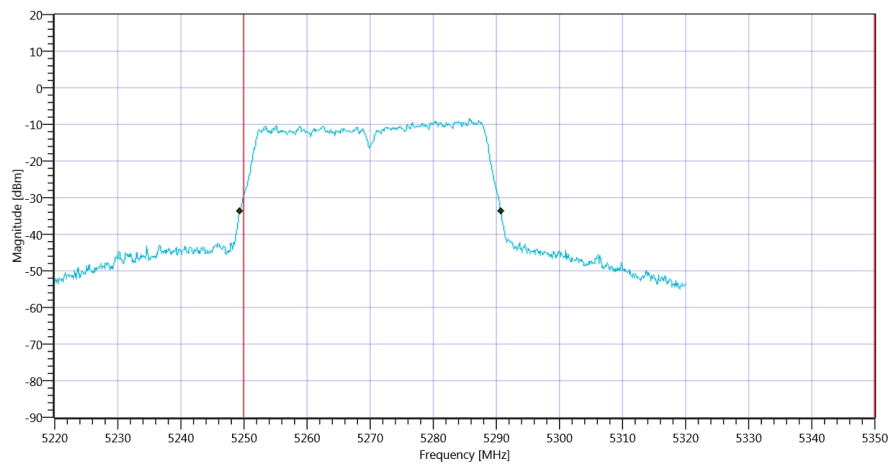
Plot_FCC Part 15.407 & ISSED Bandwidths ~ WLAN5Gx n-HT40 mode U-NII-2A_16012020_114709.png
