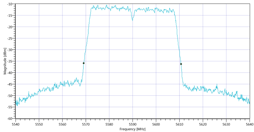
Plot_FCC Part 15.407 & ISSED Bandwidths ~ WLAN5Gx n-HT40 mode U-NII-2C 26dB_16012020_120312.png
