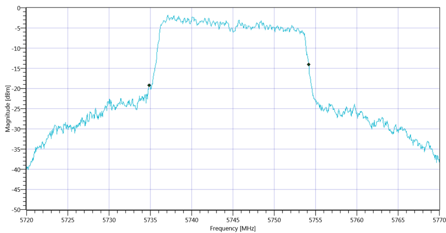
Plot_FCC Part 15.407 & ISCED Bandwidths ~ WLAN5Gx n-HT20 mode U-NII-3 99PCT_16012020_101444.png
