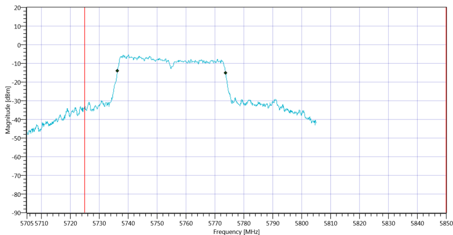
Plot_FCC Part 15.407 & ISSED Bandwidths ~ WLAN5Gx n-HT40 mode U-NII-3_16012020_121314.png
