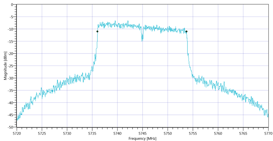
Plot_FCC Part 15.407 & ISSED Minimum Emission BW ~ WLAN5Gx n-HT20 mode U-NII-3_16012020_101542.png
