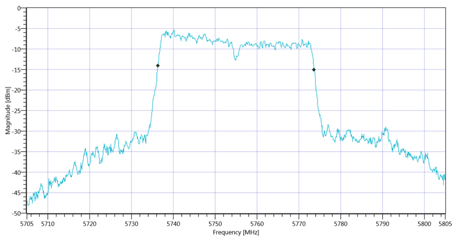
Plot_FCC Part 15.407 & ISSED Bandwidths ~ WLAN5Gx n-HT40 mode U-NII-3 99PCT_16012020_121311.png
