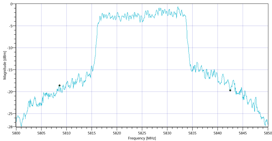
Plot_FCC Part 15.407 & ISCED Bandwidths ~ WLAN5Gx n-HT20 mode U-NII-3 99PCT_16012020_103047.png
