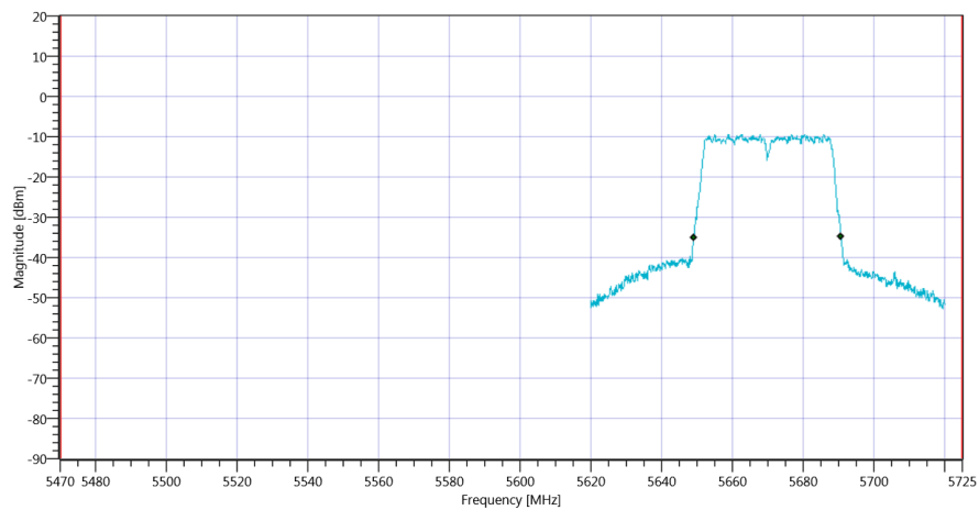
Plot_FCC Part 15.407 & ISM Bandwidths ~ WLAN5Gx n-HT40 mode U-NII-2C_16012020_120742.png
