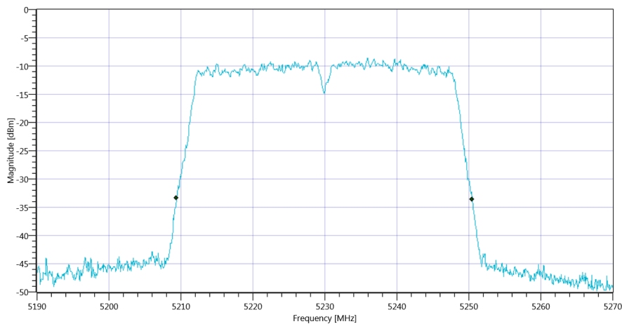
Plot_FCC Part 15.407 Max Output Power and PSD ~ WLAN5Gx n-HT40 mode U-NII-1 BW_16012020_111255.png
