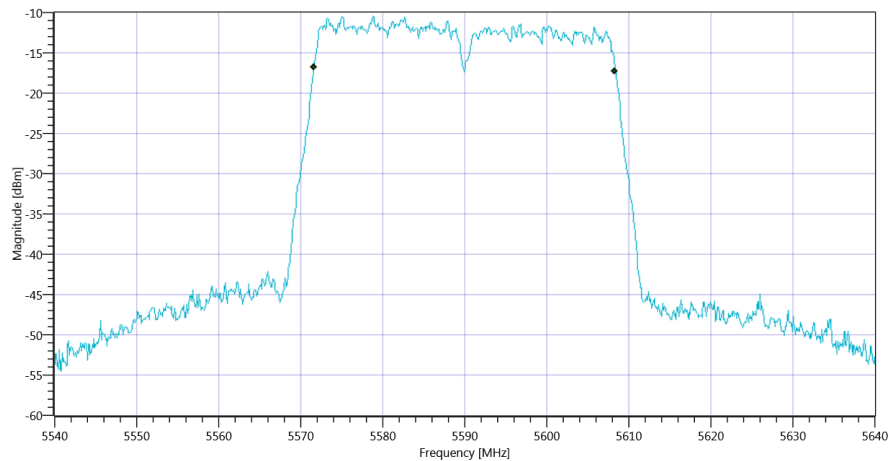
Plot_FCC Part 15.407 & ISSED Bandwidths ~ WLAN5Gx n-HT40 mode U-NII-2C 99PCT_16012020_120303.png
