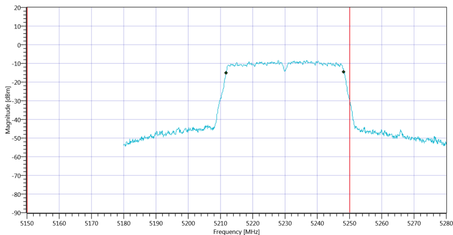
Plot_FCC Part 15.407 & ISCED Bandwidths ~ WLAN5Gx n-HT40 mode U-NII-1_16012020_111457.png
