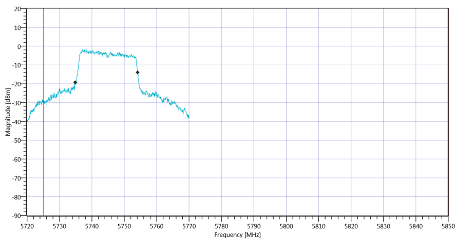
Plot_FCC Part 15.407 & ISCED Bandwidths ~ WLAN5Gx n-HT20 mode U-NII-3_16012020_101448.png
