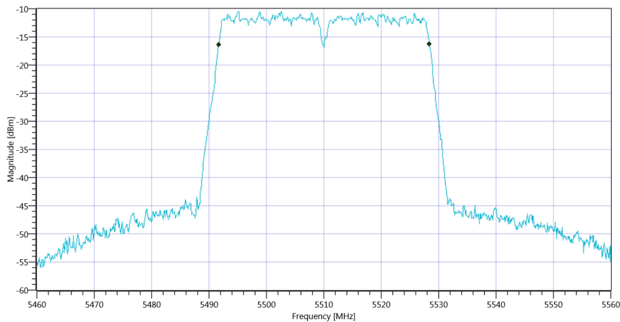
Plot_FCC Part 15.407 & ISSED Bandwidths ~ WLAN5Gx n-HT40 mode U-NII-2C 99PCT_16012020_115825.png
