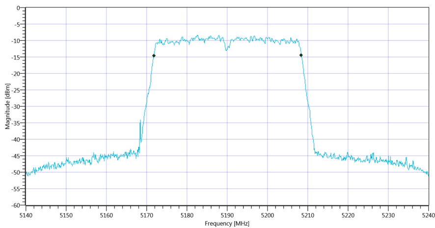
Plot_FCC Part 15.407 & ISCED Bandwidths ~ WLAN5Gx n-HT40 mode U-NII-1 99PCT_16012020_104305.png
