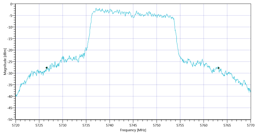
Plot_FCC Part 15.407 & ISSED Bandwidths ~ WLAN5Gx n-HT20 mode U-NII-3 26dB_16012020_101453.png
