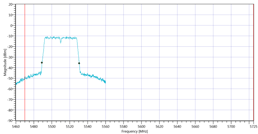
Plot_FCC Part 15.407 & ISSED Bandwidths ~ WLAN5Gx n-HT40 mode U-NII-2C_16012020_115839.png
