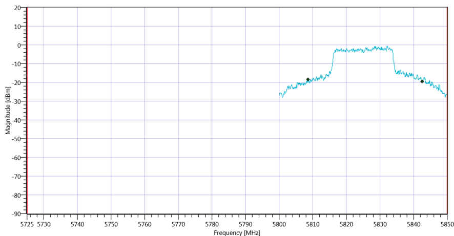
Plot_FCC Part 15.407 & ISCED Bandwidths ~ WLAN5Gx n-HT20 mode U-NII-3_16012020_103051.png
