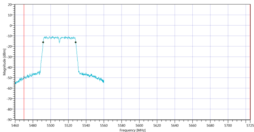
Plot_FCC Part 15.407 & ISSED Bandwidths ~ WLAN5Gx n-HT40 mode U-NII-2C_16012020_115829.png
