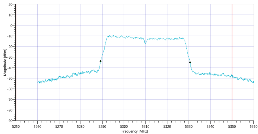
Plot_FCC Part 15.407 & ISM Bandwidths ~ WLAN5Gx n-HT40 mode U-NII-2A_16012020_115319.png
