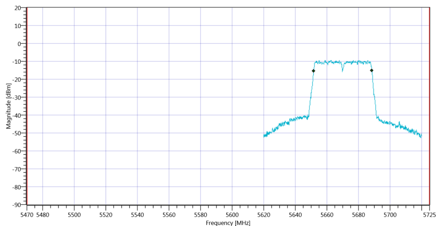
Plot_FCC Part 15.407 & ISSED Bandwidths ~ WLAN5Gx n-HT40 mode U-NII-2C_16012020_120733.png
