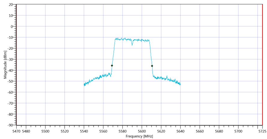
Plot_FCC Part 15.407 & ISSED Bandwidths ~ WLAN5Gx n-HT40 mode U-NII-2C_16012020_120316.png
