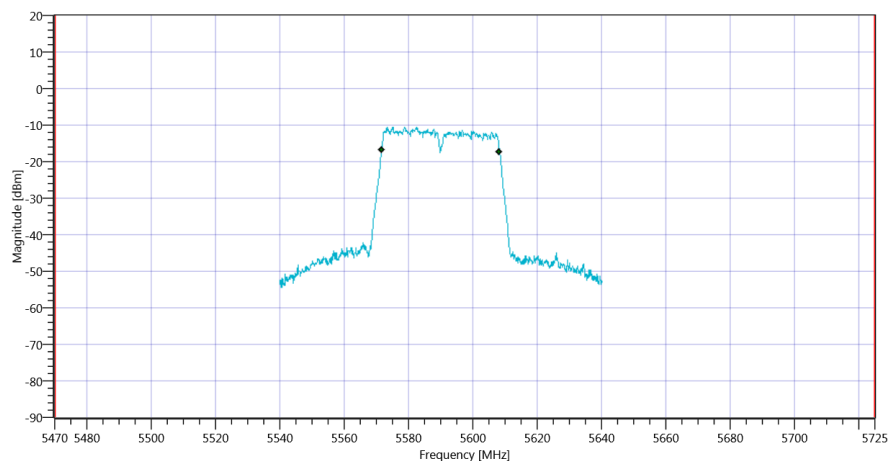
Plot_FCC Part 15.407 & ISSED Bandwidths ~ WLAN5Gx n-HT40 mode U-NII-2C_16012020_120307.png
