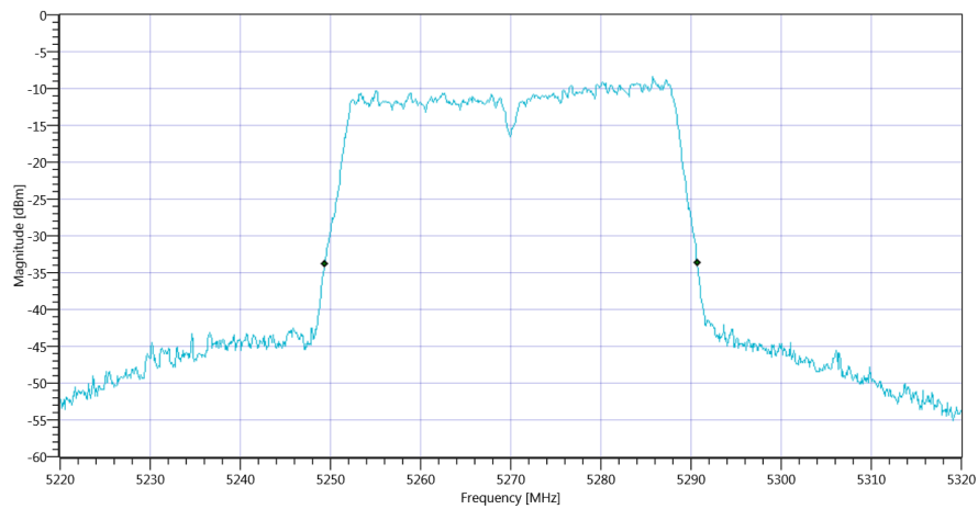
Plot_FCC Part 15.407 & ISSED Bandwidths ~ WLAN5Gx n-HT40 mode U-NII-2A 26dB_16012020_114705.png
