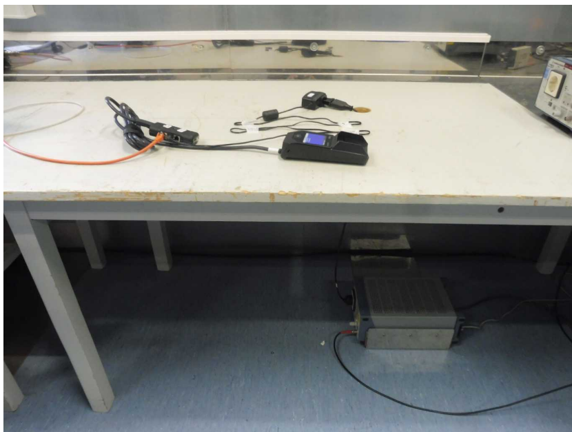
Photo 8: AC conducted emission test setup
