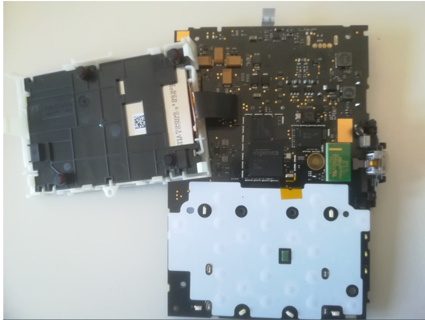
Photo 5: electronics underneath the display
