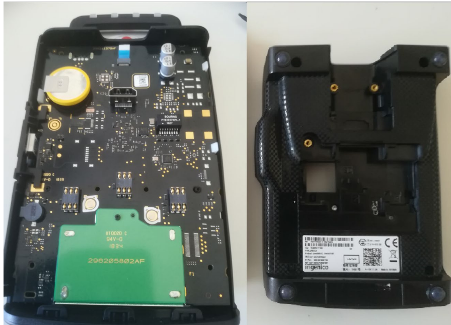
Photo 1: Bottom side back cover removed
