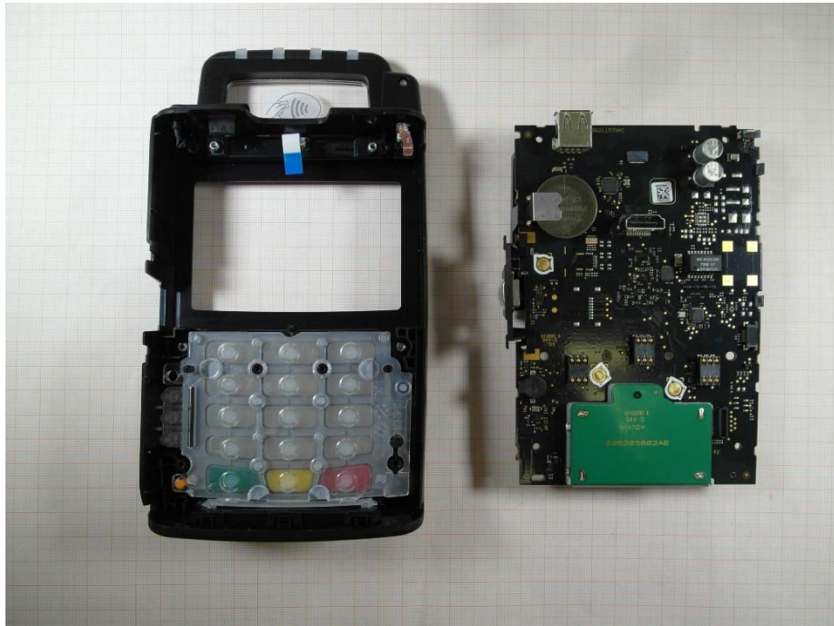
Photo 2: PCB removed from case
