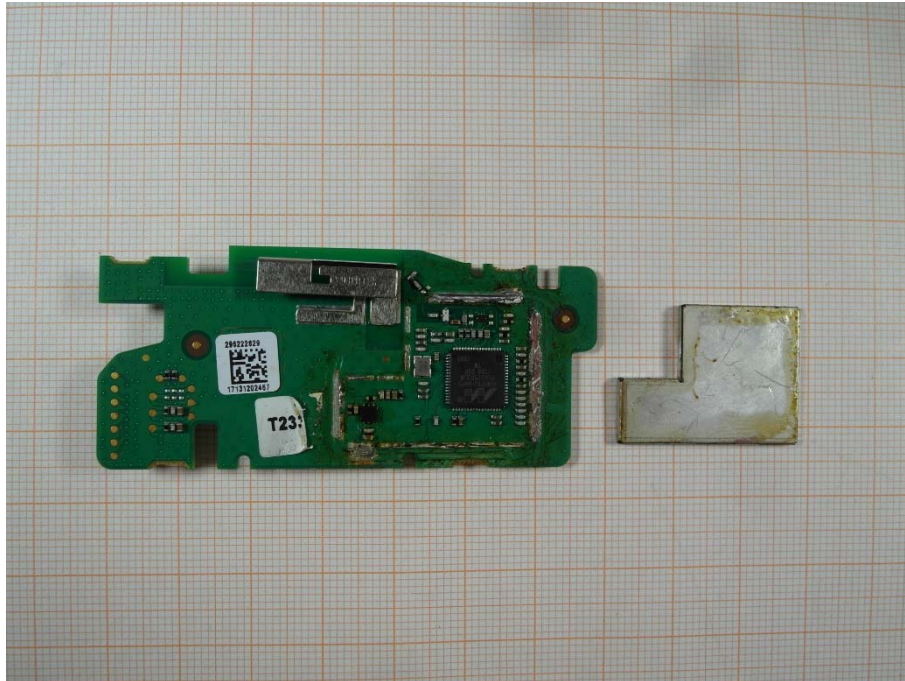
Photo 15: RF module shield removed
