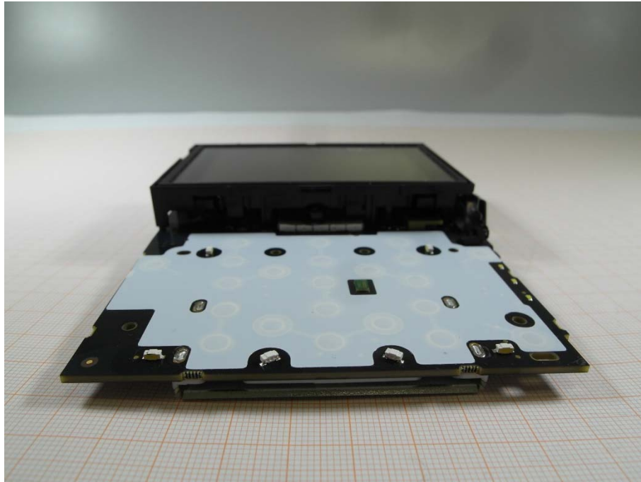
Photo 9: Bottom view on display and keypad
