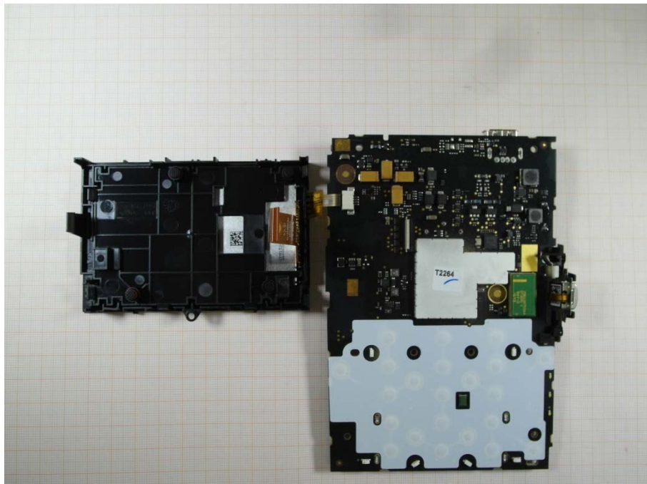
Photo 10: PCB with display removed
