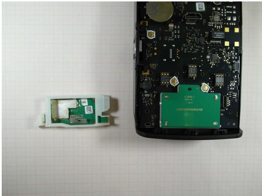
Photo 4: RF module removed
