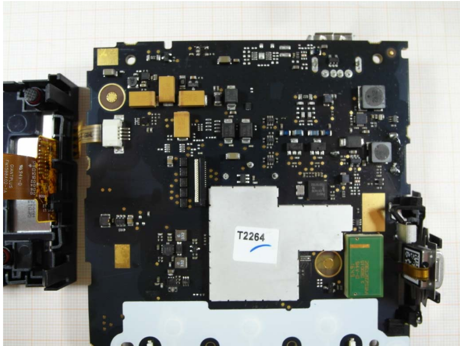
Photo 11: electronics underneath the display
