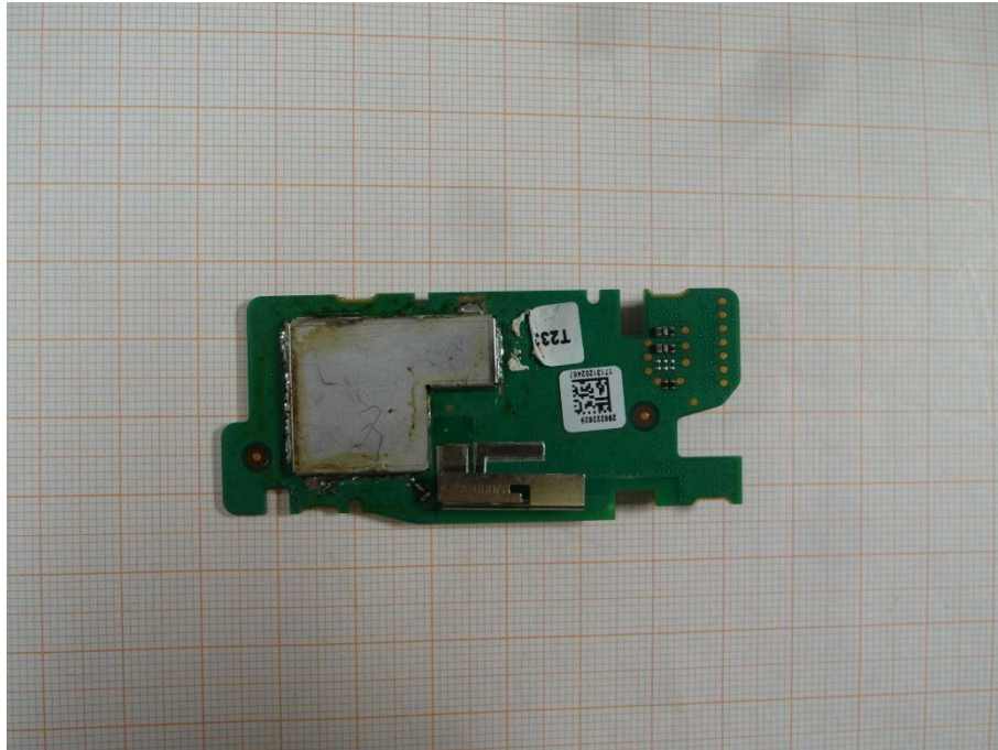
Photo 13: RF module top view
