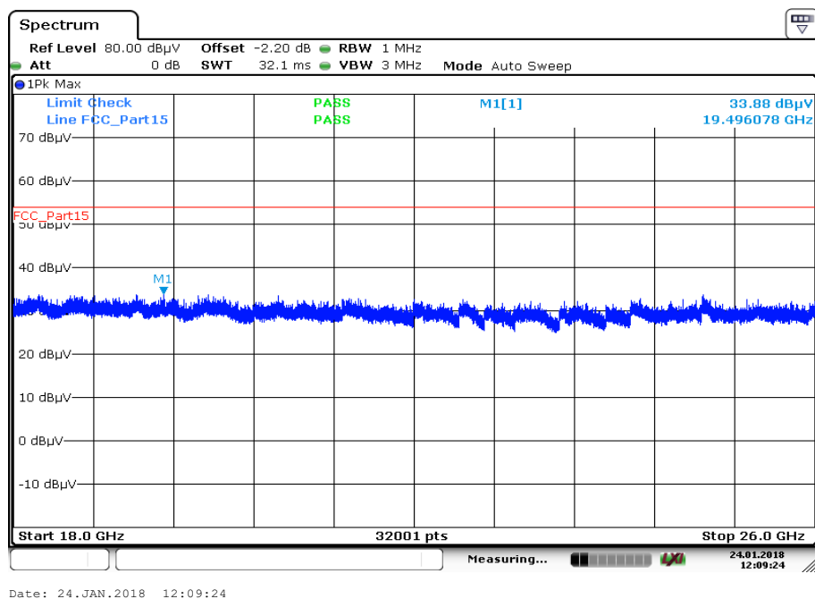
Plot 39: 18 GHz to 26 GHz; vertical & horizontal polarization; U-NII-3; lowest channel
