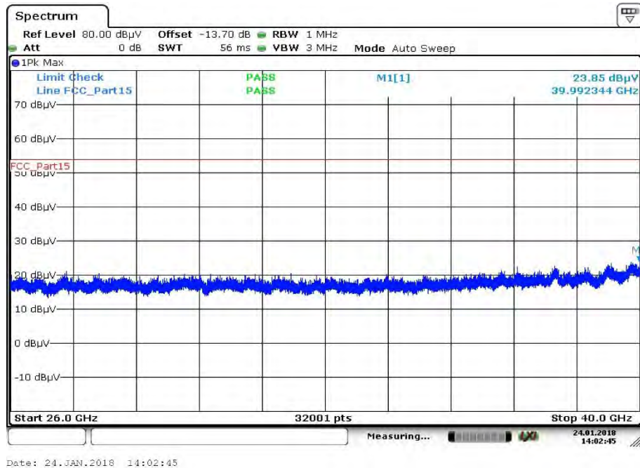
Plot 48: 26 GHz to 40 GHz; vertical & horizontal polarization; U-NII-3; highest channel
