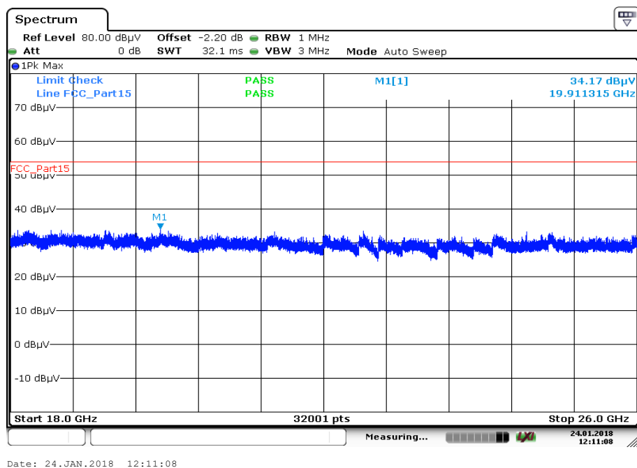
Plot 43: 18 GHz to 26 GHz; vertical & horizontal polarization; U-NII-3; middle channel
