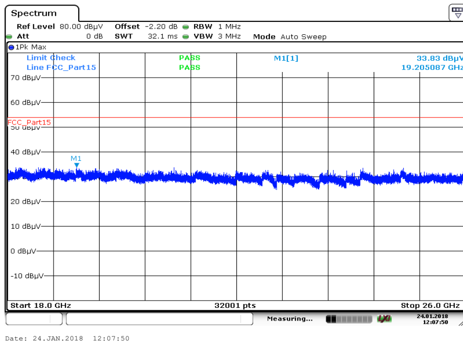
Plot 35: 18 GHz to 26 GHz; vertical & horizontal polarization; U-NII-2C; highest channel
