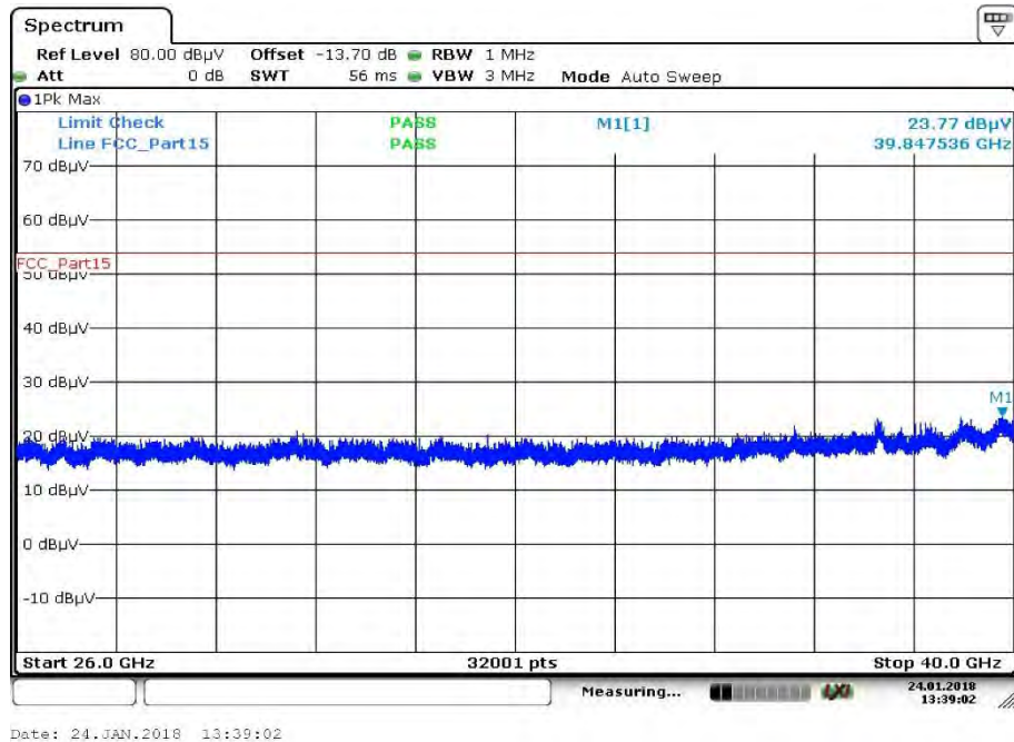
Plot 36: 26 GHz to 40 GHz; vertical & horizontal polarization; U-NII-2C; highest channel
