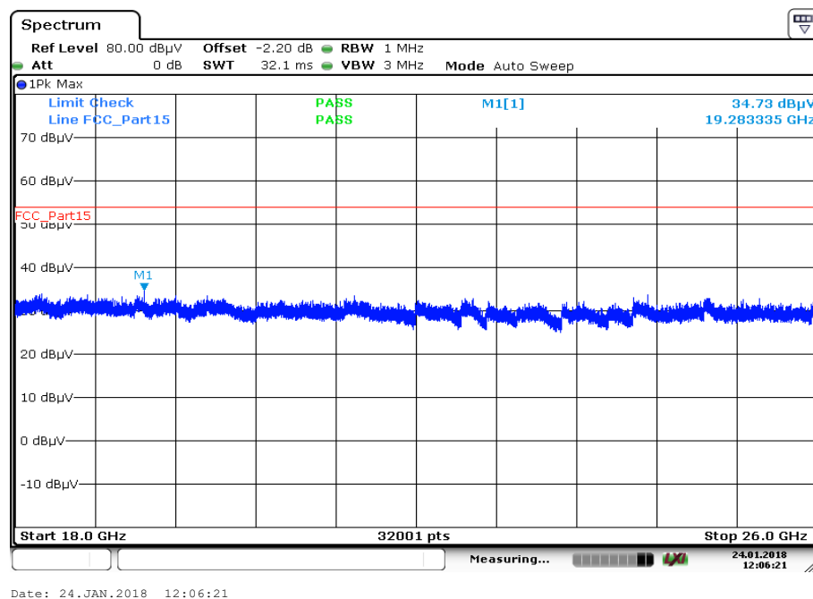
Plot 31: 18 GHz to 26 GHz; vertical & horizontal polarization; U-NII-2C; middle channel
