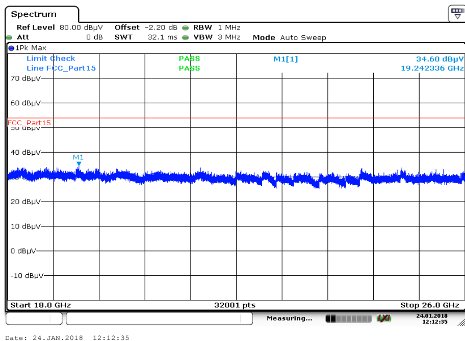
Plot 47: 18 GHz to 26 GHz; vertical & horizontal polarization; U-NII-3; highest channel
