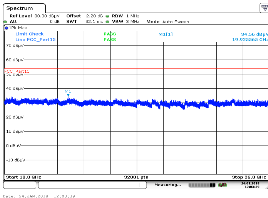
Plot 27: 18 GHz to 26 GHz; vertical & horizontal polarization; U-NII-2C; lowest channel
