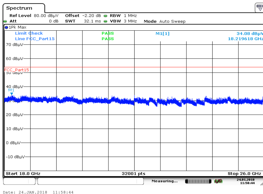
Plot 15: 18 GHz to 26 GHz; vertical & horizontal polarization; U-NII-2A; lowest channel
