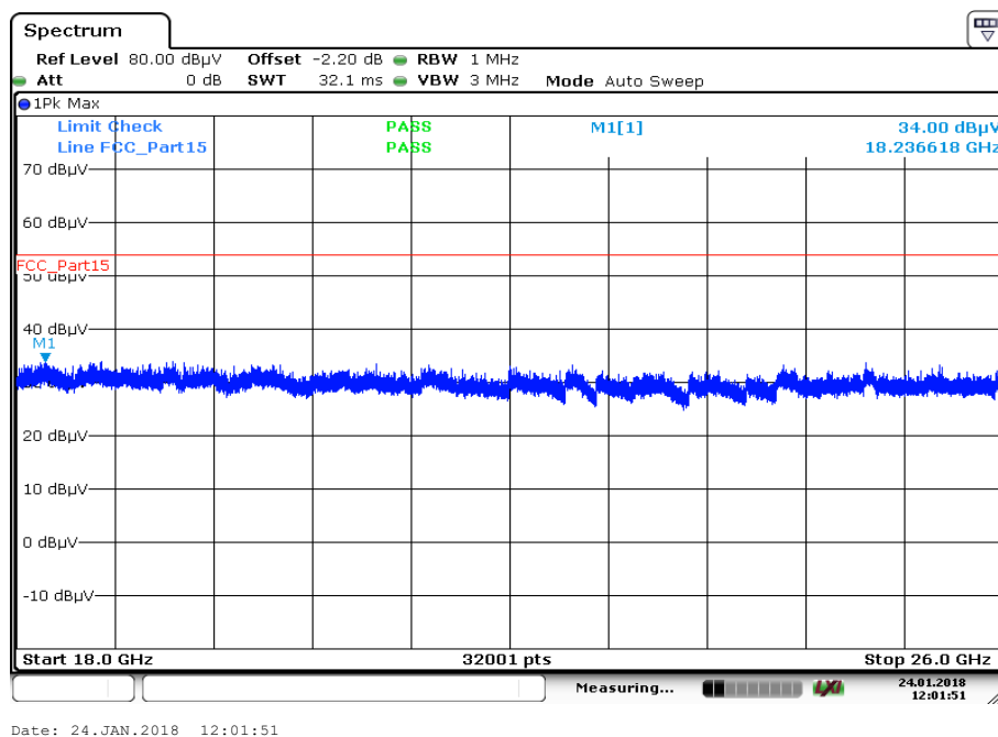
Plot 23: 18 GHz to 26 GHz; vertical & horizontal polarization; U-NII-2A; highest channel
