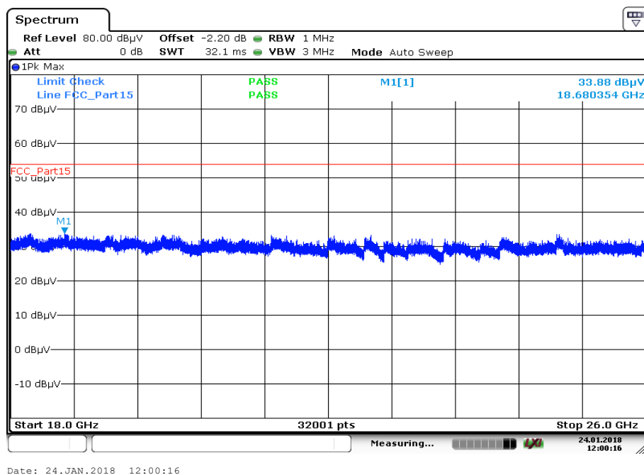
Plot 19: 18 GHz to 26 GHz; vertical & horizontal polarization; U-NII-2A; middle channel
