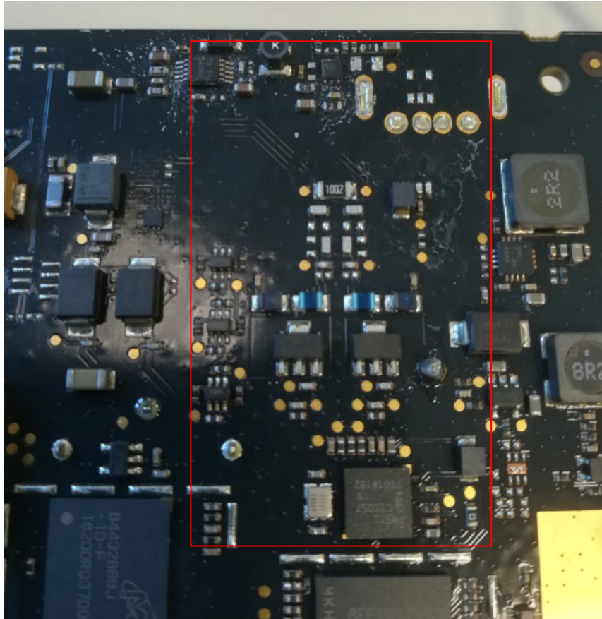
Photo 10: RFID electronics
