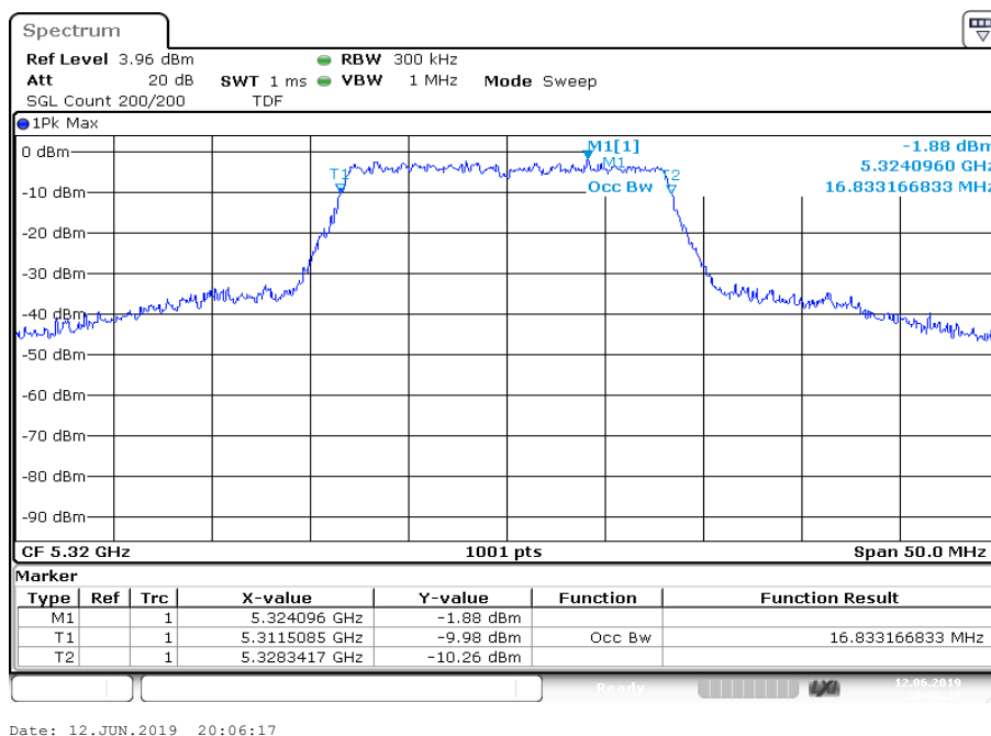
Plot 6: U-NII-2A; highest channel
