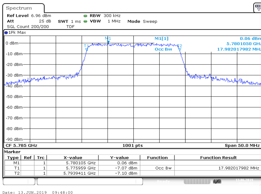
Plot 11: U-NII-3; middle channel
