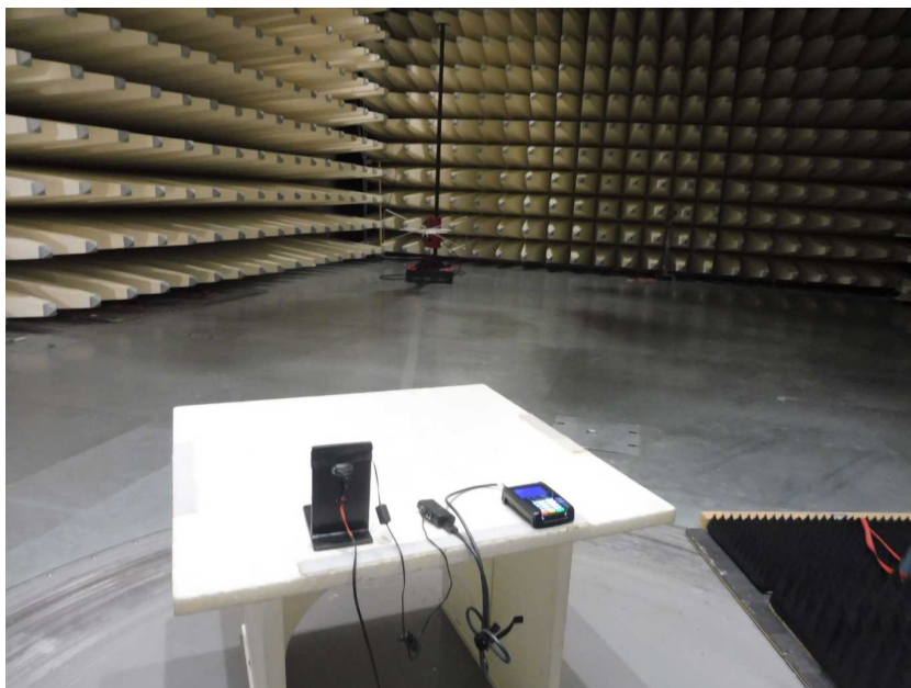
Photo 6: RSE test setup <1GHz
