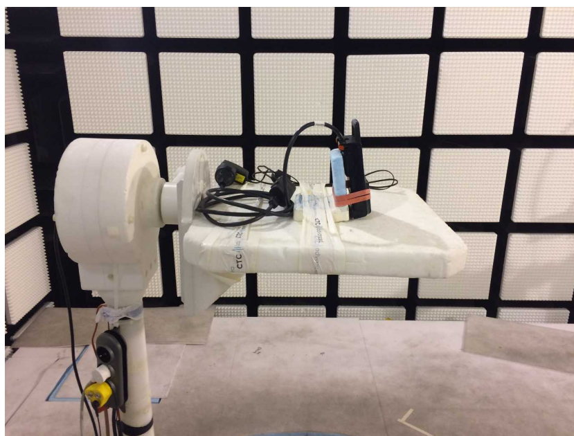
Photo 4: RSE test setup >1GHz
