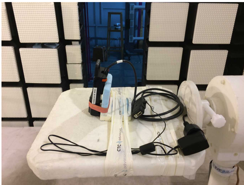
Photo 2: RSE test setup >1GHz
