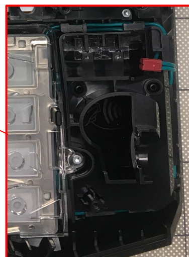
Contactless antenna
