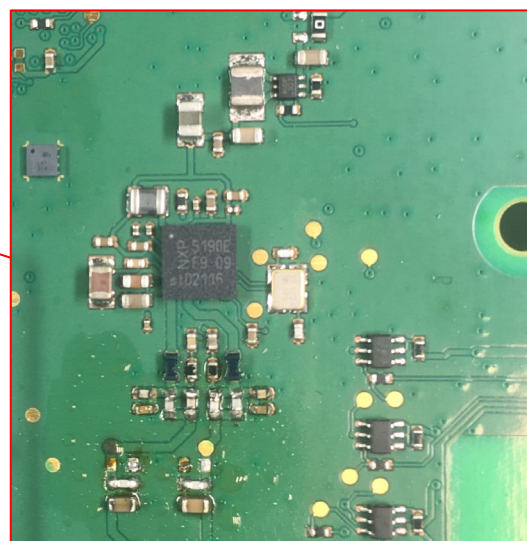
Contactless chip: NXP 5190E
