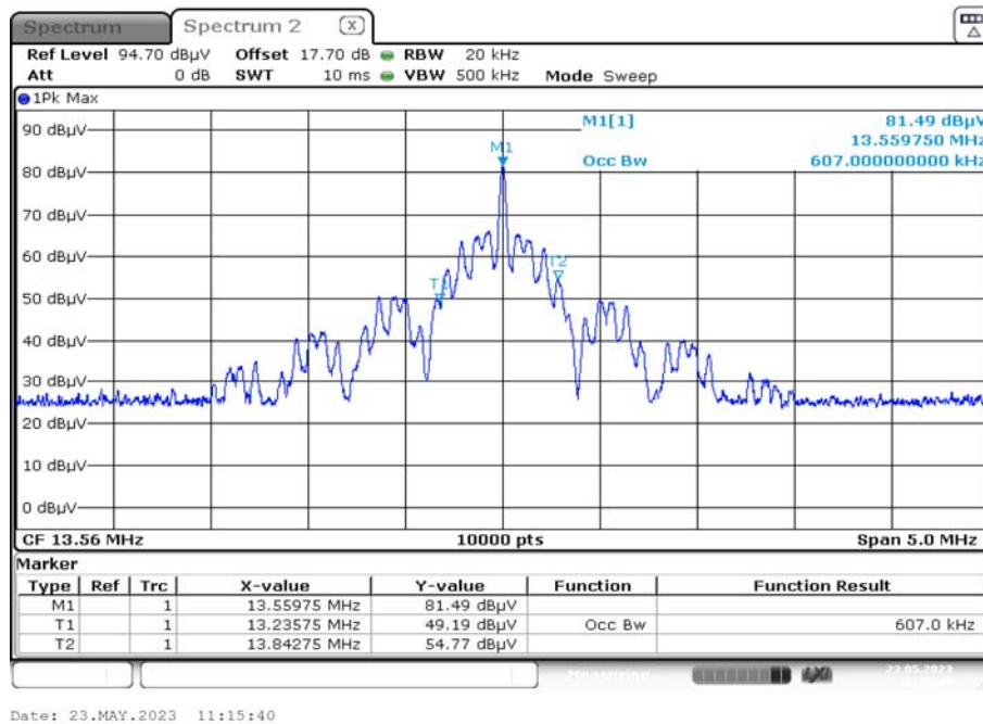
Plot 1: 99 % emission bandwidth Mode 1
