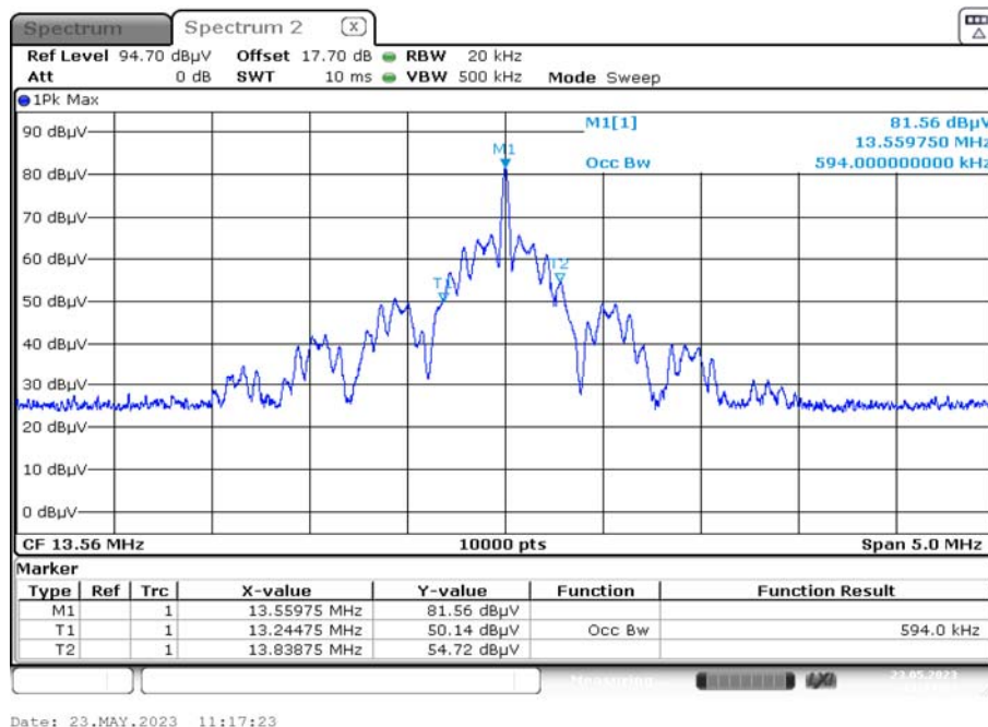
Plot 2: 99 % emission bandwidth Mode 2
