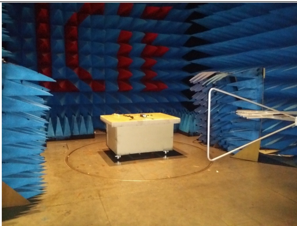
Photograph for Field strength outside of the bands 13.110-14.010 MHz
