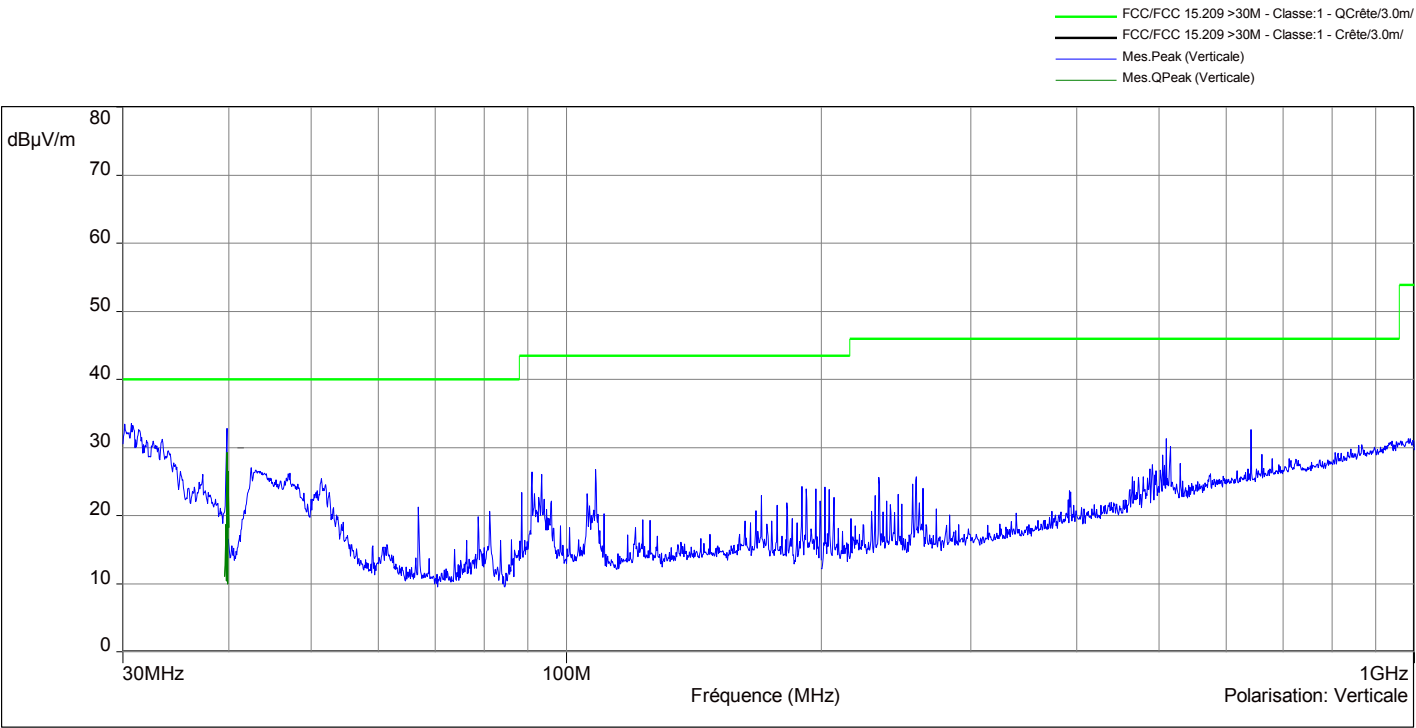
Vertical Polarization (30-1000MHz)
