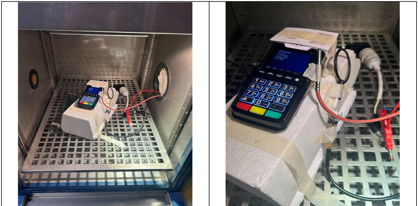
Photo of Field strength within the band 13.110-14.010MHz in Climatic Chamber
