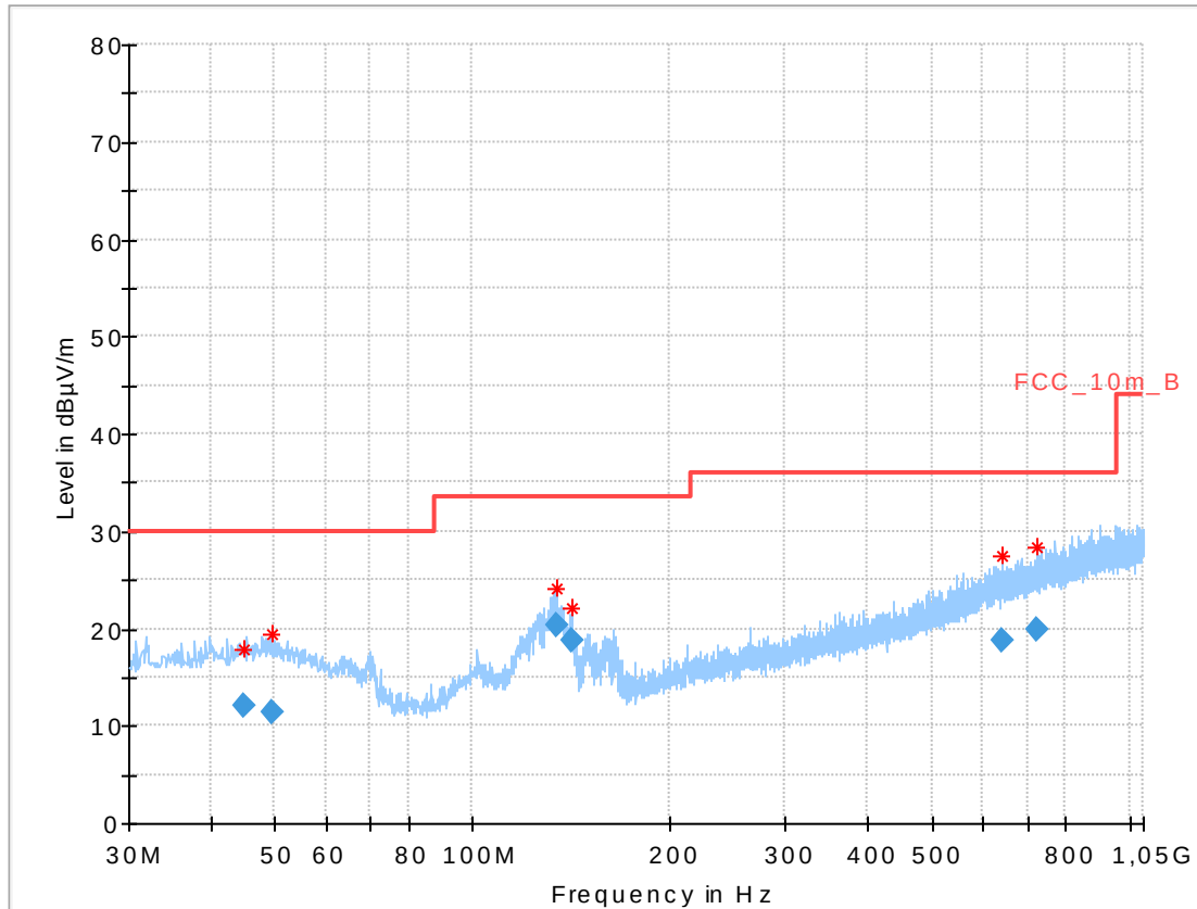
Plot 2: 30 MHz to 1 GHz, TX mode, channel 39, vertical & horizontal polarization
