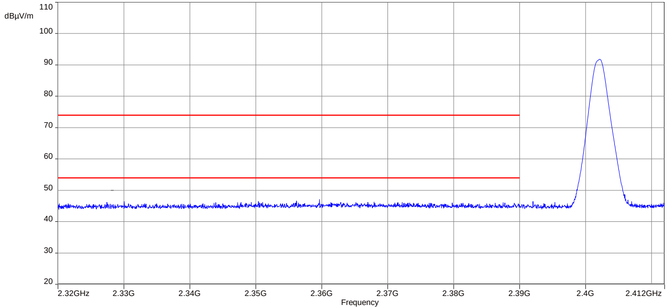
Plot 1: Lower band edge, GFSK modulation, vertical & horizontal polarization
