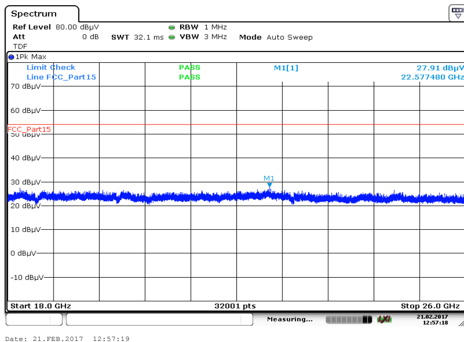
Plot 11: 18 GHz to 26 GHz, 5310 MHz, vertical & horizontal polarization
