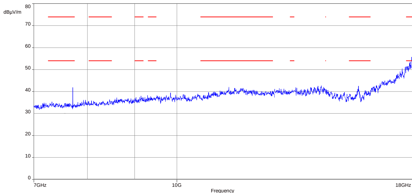
Plot 23: 7 GHz to 18 GHz, 5785 MHz, vertical & horizontal polarization
