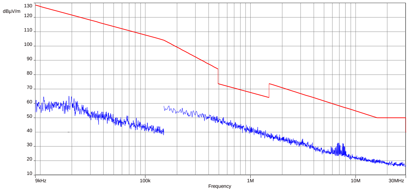
Plot 4: 9 kHz to 30 MHz, OFDM 20 MHz, 5745 MHz
