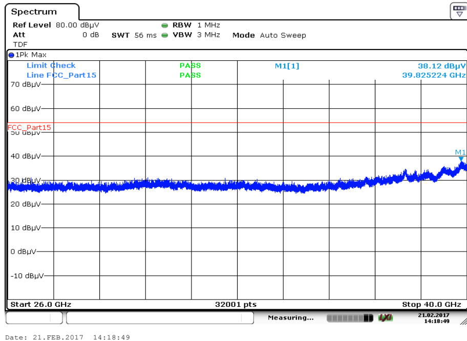
Plot 20: 26 GHz to 40 GHz, 5795 MHz, vertical & horizontal polarization
