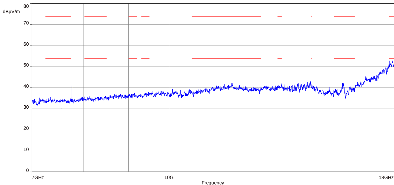
Plot 29: 7 GHz to 18 GHz, 5825 MHz, vertical & horizontal polarization
