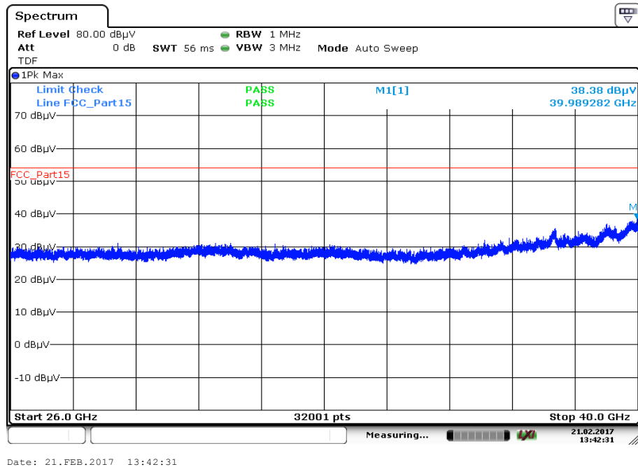
Plot 12: 26 GHz to 40 GHz, 5310 MHz, vertical & horizontal polarization
