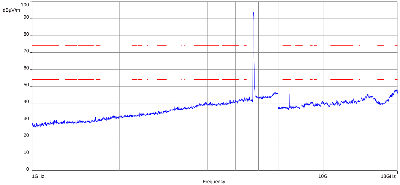
Plot 14: 1 GHz to 18 GHz, 5755 MHz, vertical & horizontal polarization
