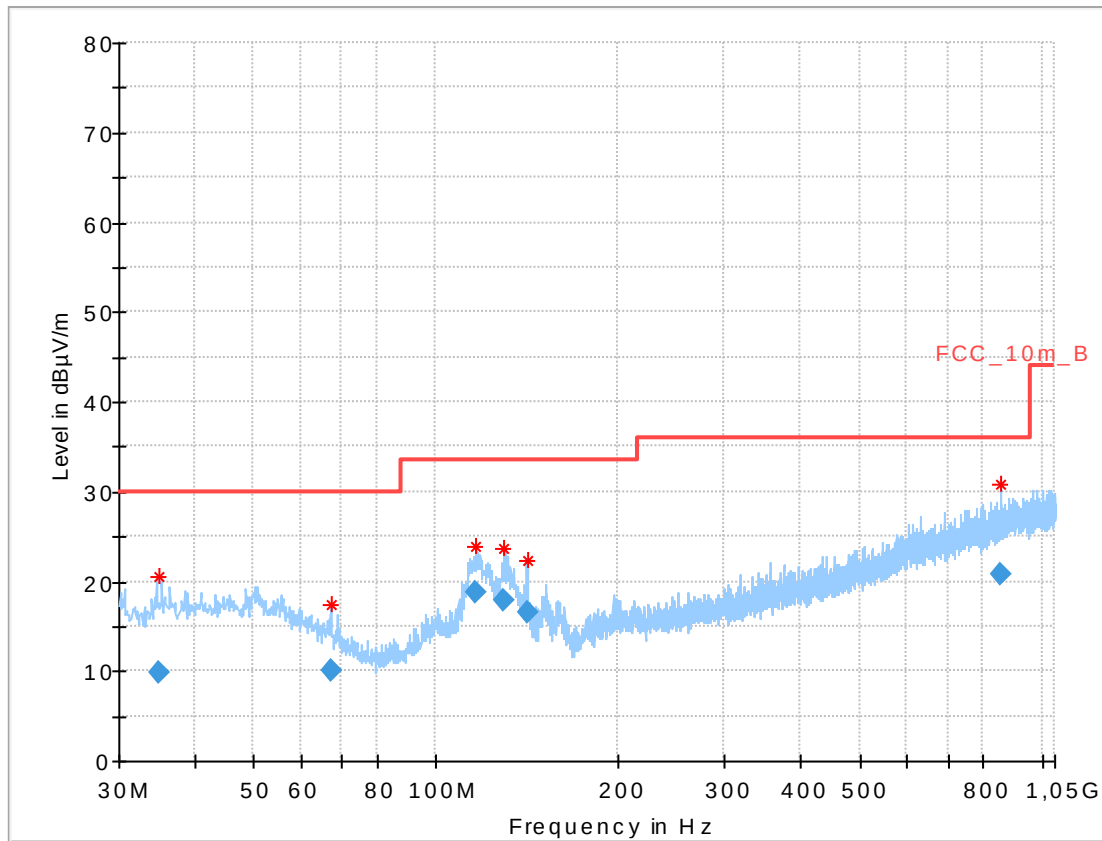
Plot 5: 30 MHz to 1 GHz, 5250 MHz, vertical & horizontal polarization
