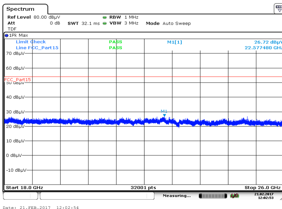
Plot 25: 18 GHz to 26 GHz, 5785 MHz, vertical & horizontal polarization
