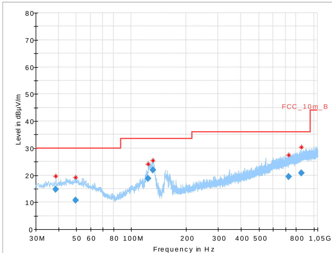
Plot 15: 30 MHz to 1 GHz, 5745 MHz, vertical & horizontal polarization
