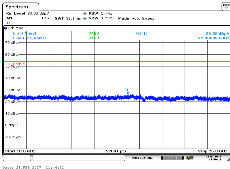
Plot 13: 18 GHz to 26 GHz, 5320 MHz, vertical & horizontal polarization
