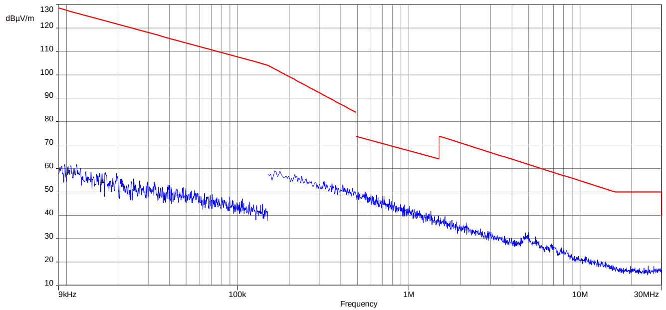
Plot 11: 9 kHz to 30 MHz, OFDM 40 MHz, 5795 MHz
