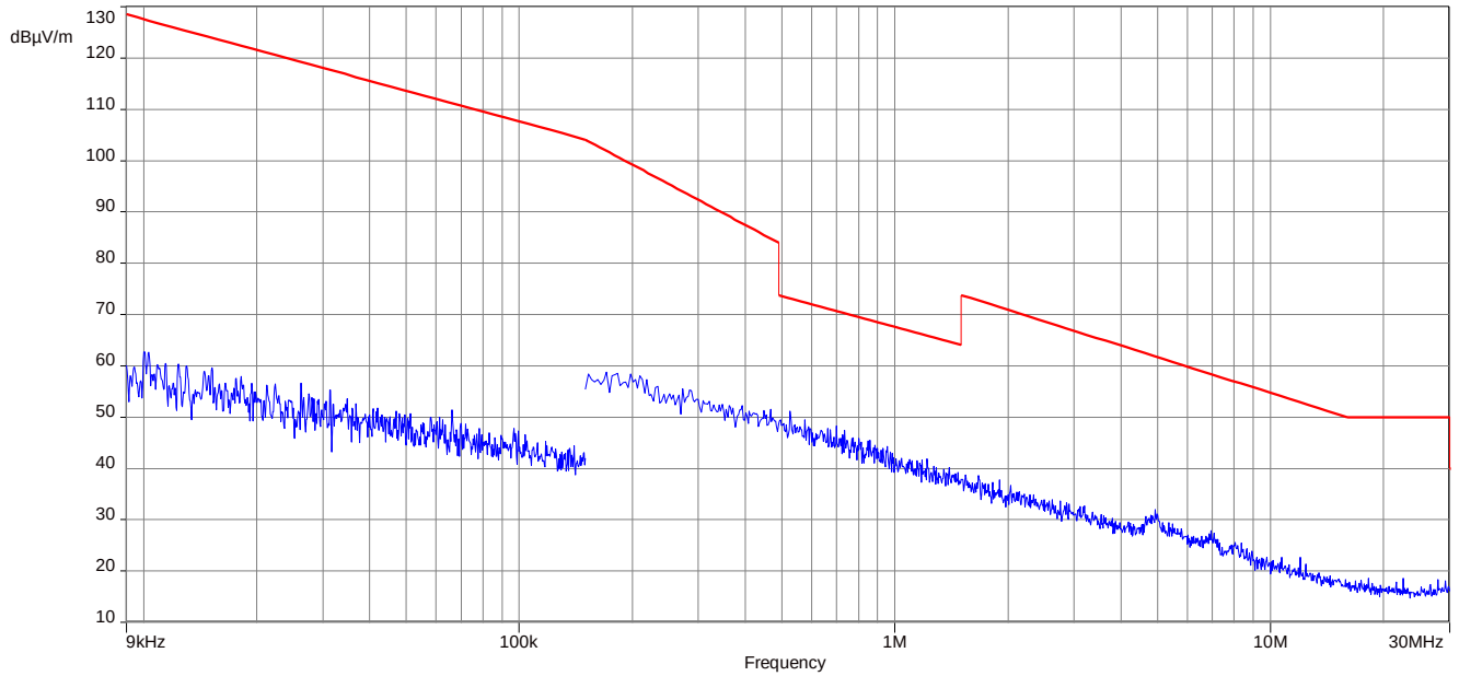
Plot 7: 9 kHz to 30 MHz, OFDM 40 MHz, 5190 MHz
