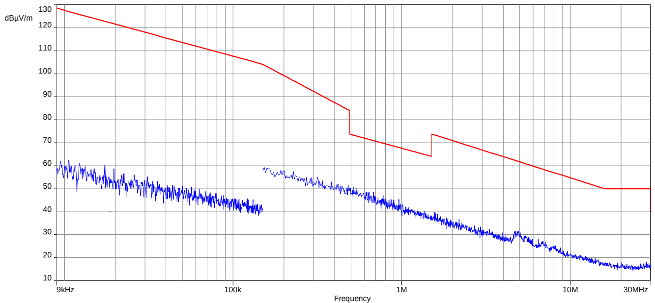
Plot 8: 9 kHz to 30 MHz, OFDM 40 MHz, 5250 MHz
