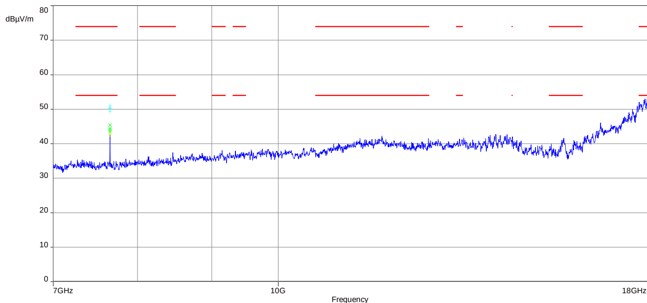
Plot 17: 7 GHz to 18 GHz, 5745 MHz, vertical & horizontal polarization
