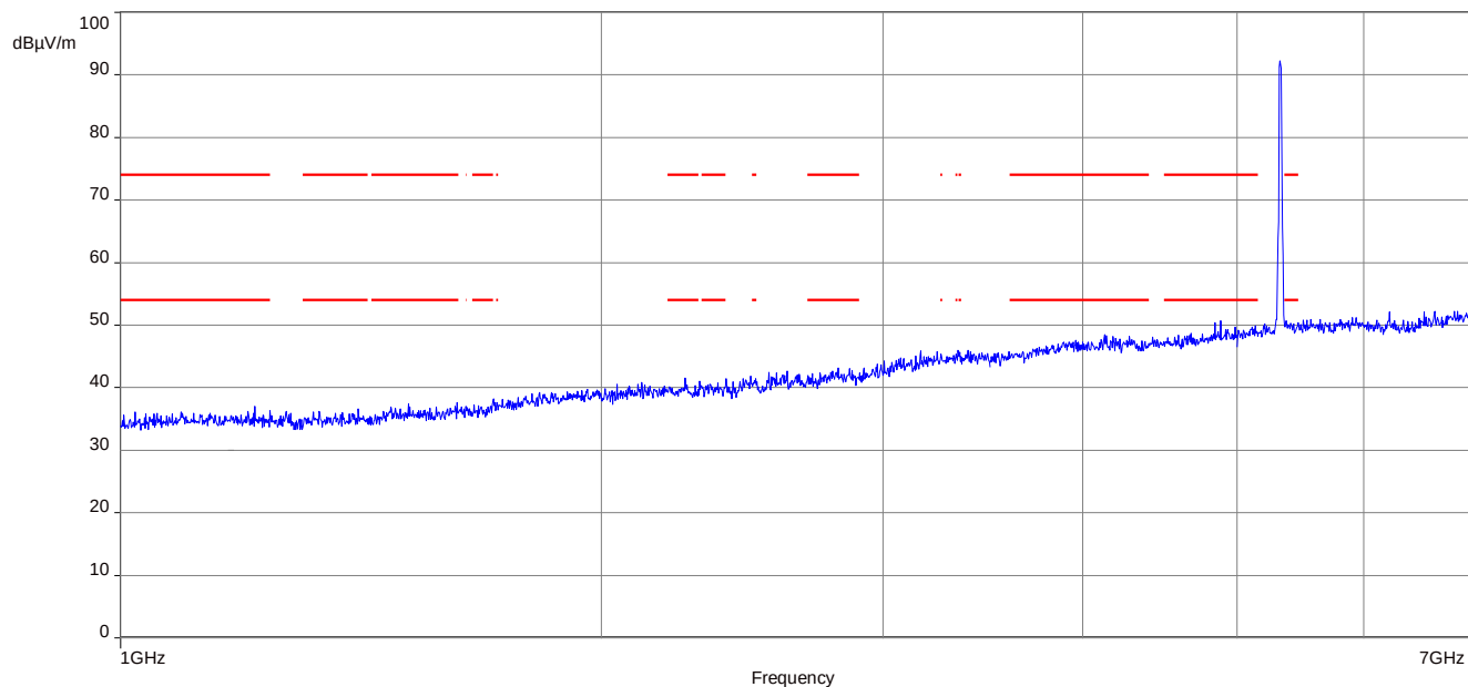
Plot 10: 1 GHz to 7 GHz, 5320 MHz, vertical & horizontal polarization
