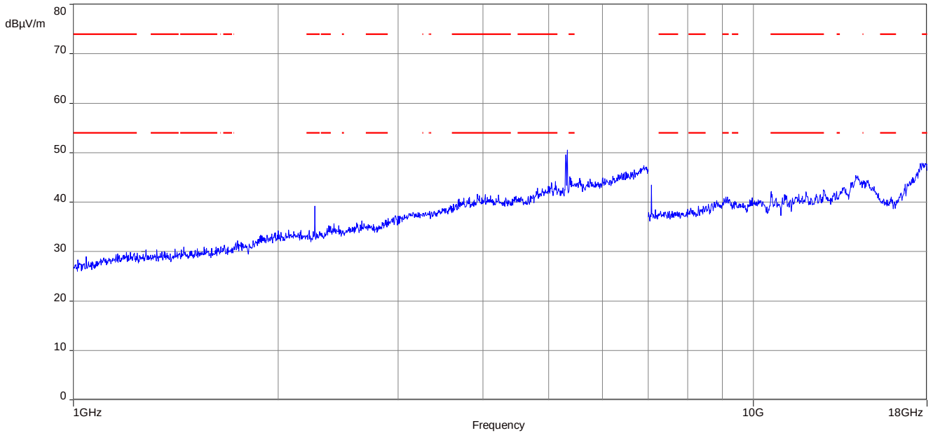
Plot 10: 1 GHz to 18 GHz, 5310 MHz, vertical & horizontal polarization
