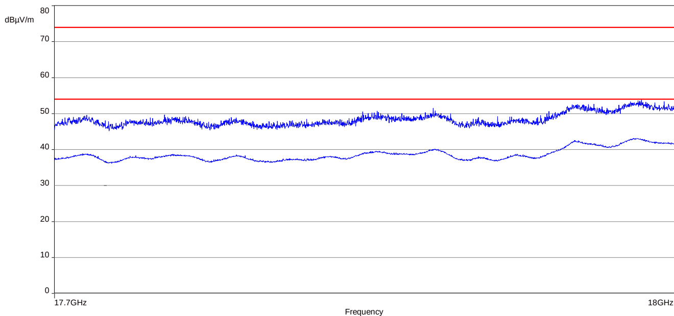
Plot 24: 17.7 GHz to 18 GHz, 5785 MHz, vertical & horizontal polarization
