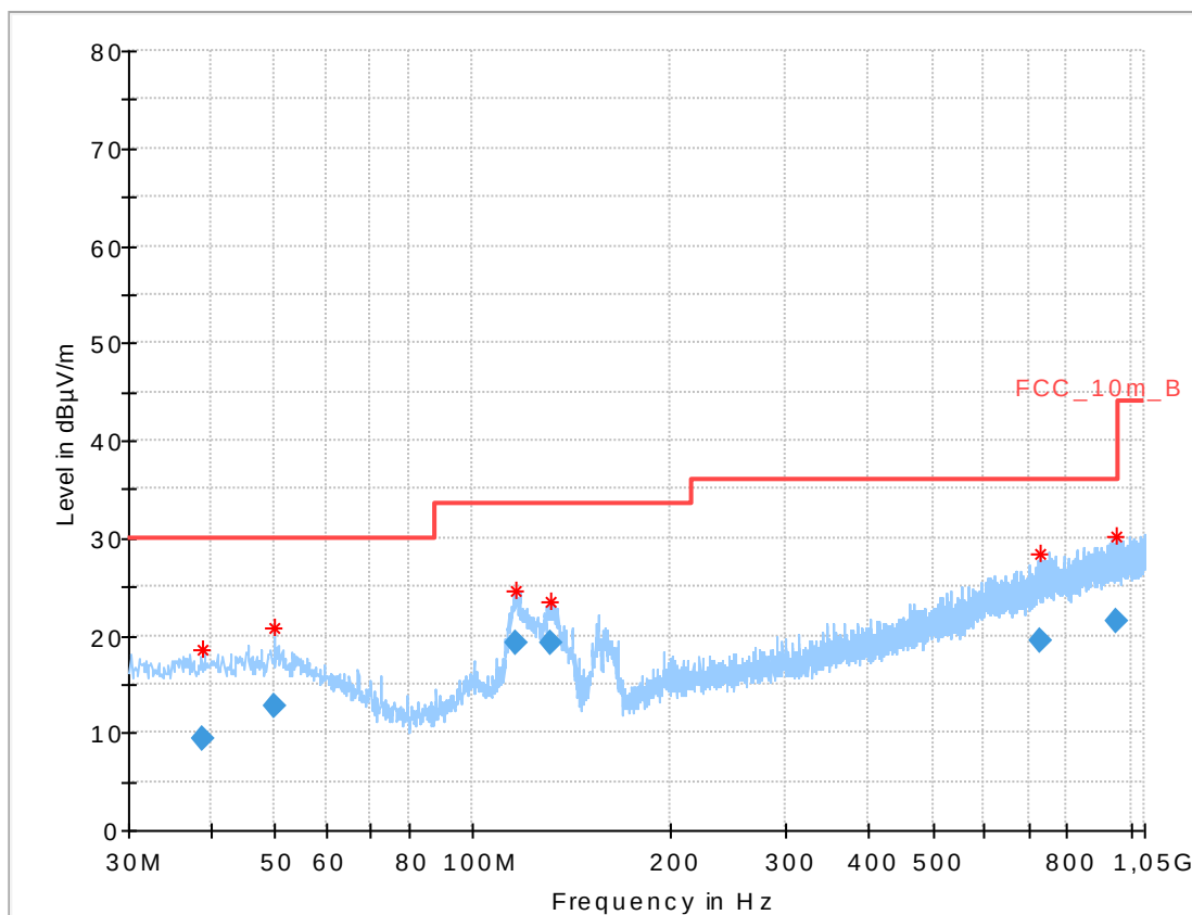
Plot 13: 30 MHz to 1 GHz, 5755 MHz, vertical & horizontal polarization
