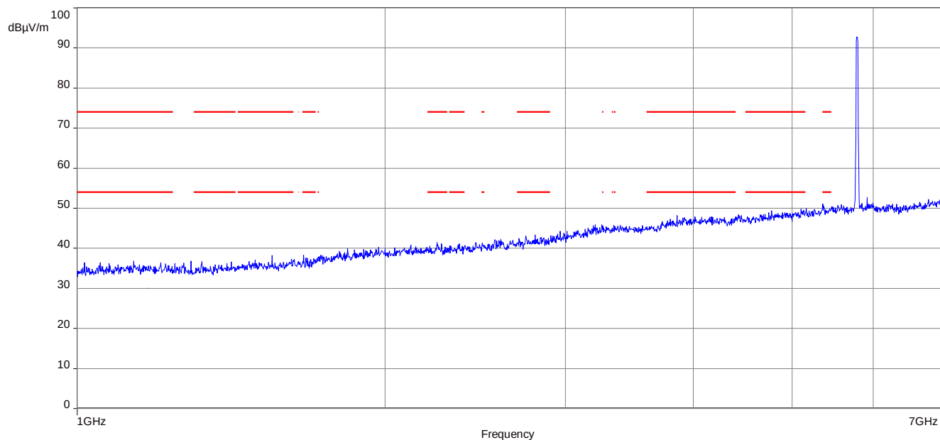
Plot 22: 1 GHz to 7 GHz, 5785 MHz, vertical & horizontal polarization
