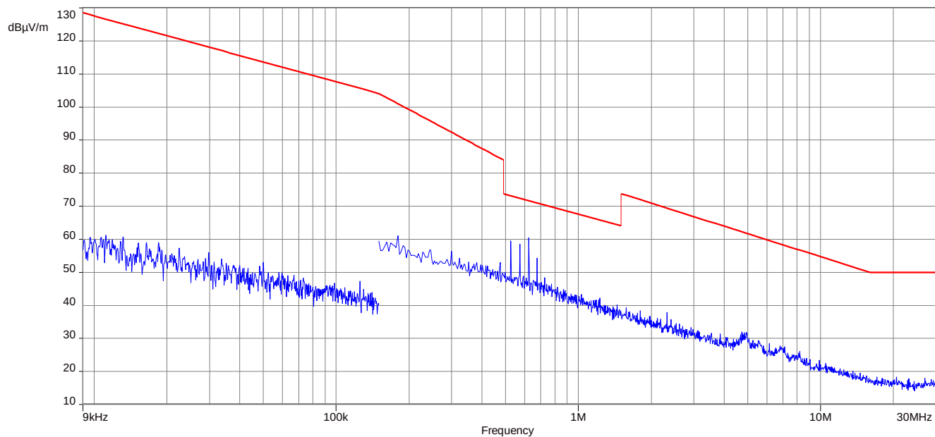
Plot 9: 9 kHz to 30 MHz, OFDM 40 MHz, 5310 MHz
