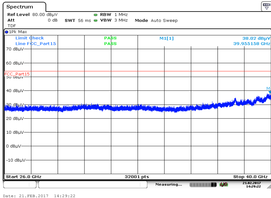
Plot 8: 26 GHz to 40 GHz, 5250 MHz, vertical & horizontal polarization
