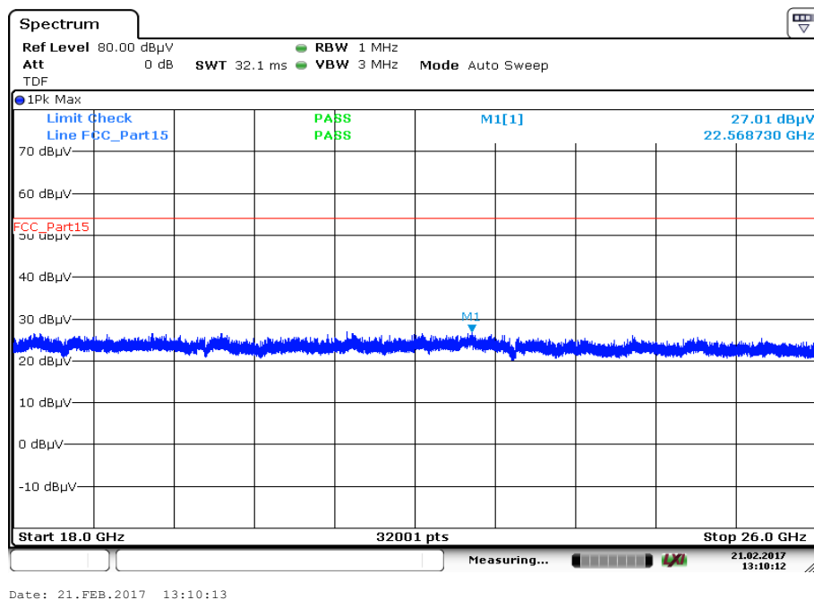
Plot 15: 18 GHz to 26 GHz, 5755 MHz, vertical & horizontal polarization
