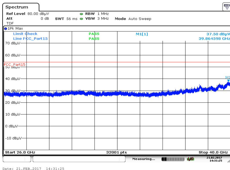
Plot 14: 26 GHz to 40 GHz, 5320 MHz, vertical & horizontal polarization
