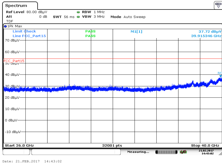
Plot 26: 26 GHz to 40 GHz, 5785 MHz, vertical & horizontal polarization
