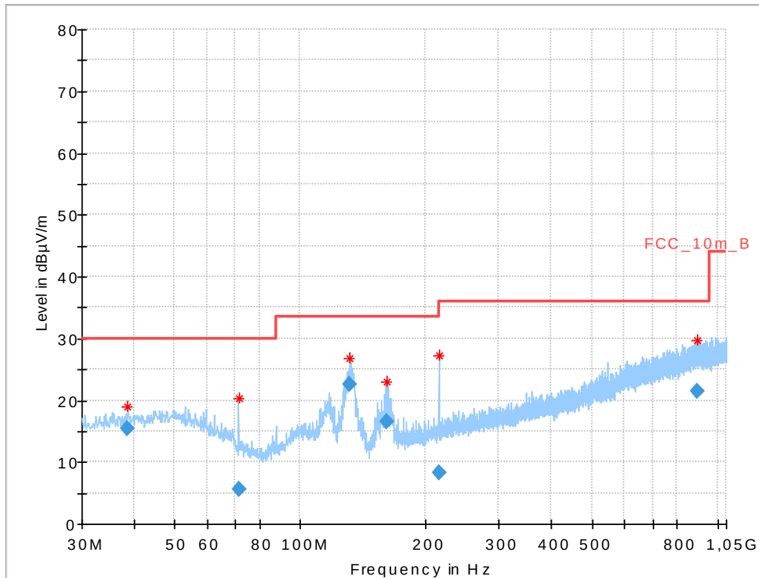
Plot 27: 30 MHz to 1 GHz, 5825 MHz, vertical & horizontal polarization
