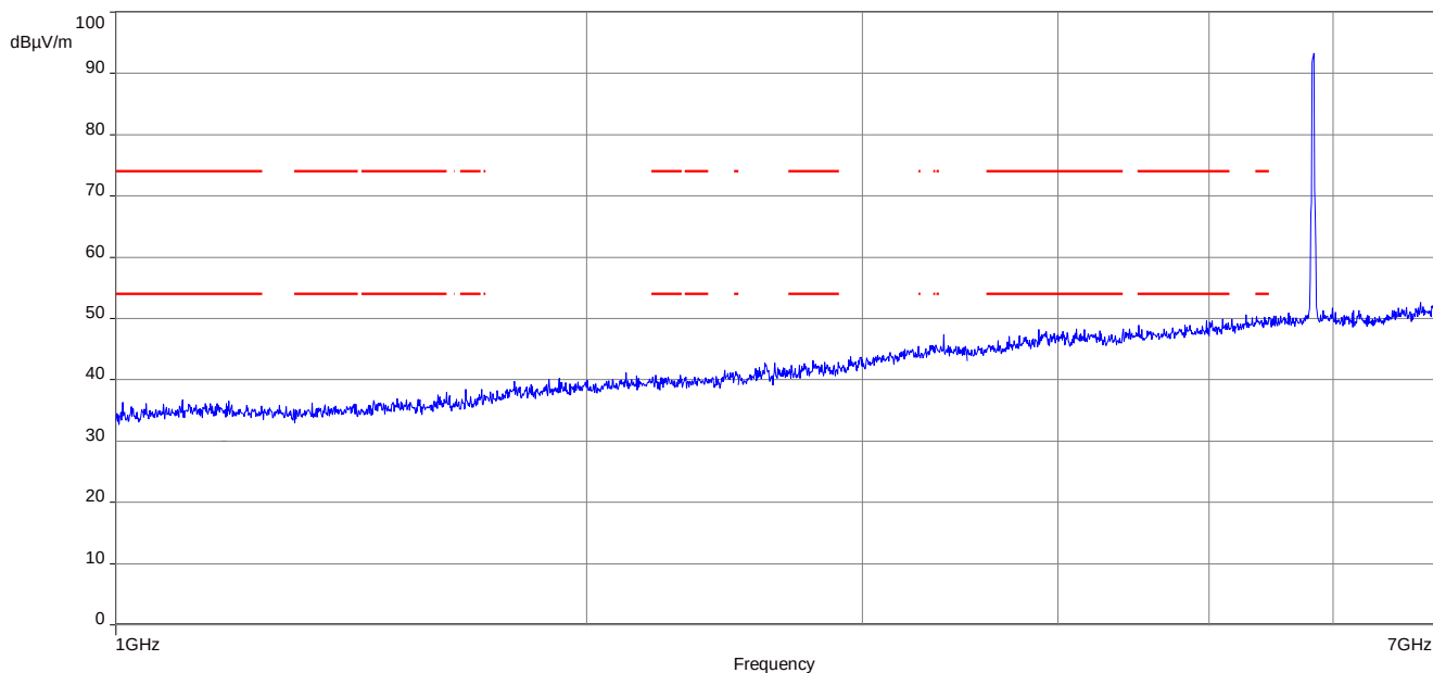
Plot 28: 1 GHz to 7 GHz, 5825 MHz, vertical & horizontal polarization
