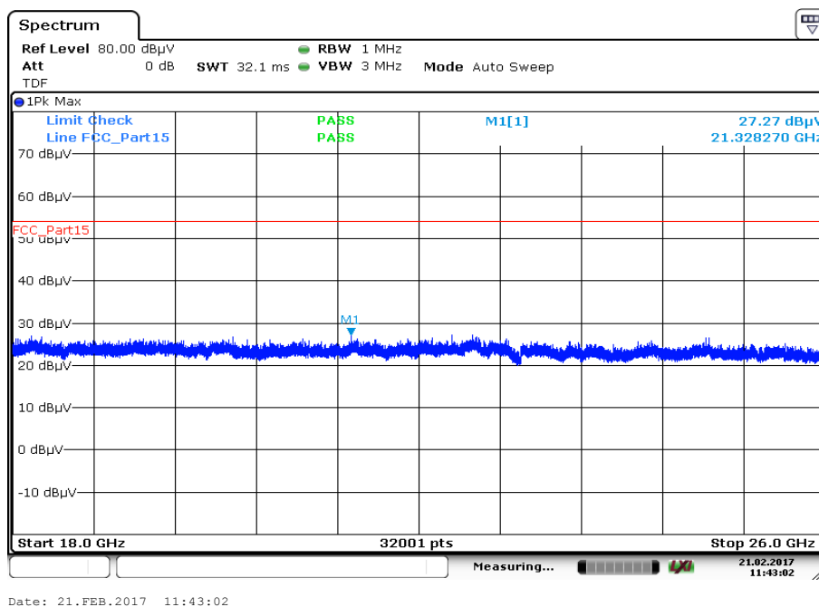
Plot 7: 18 GHz to 26 GHz, 5250 MHz, vertical & horizontal polarization
