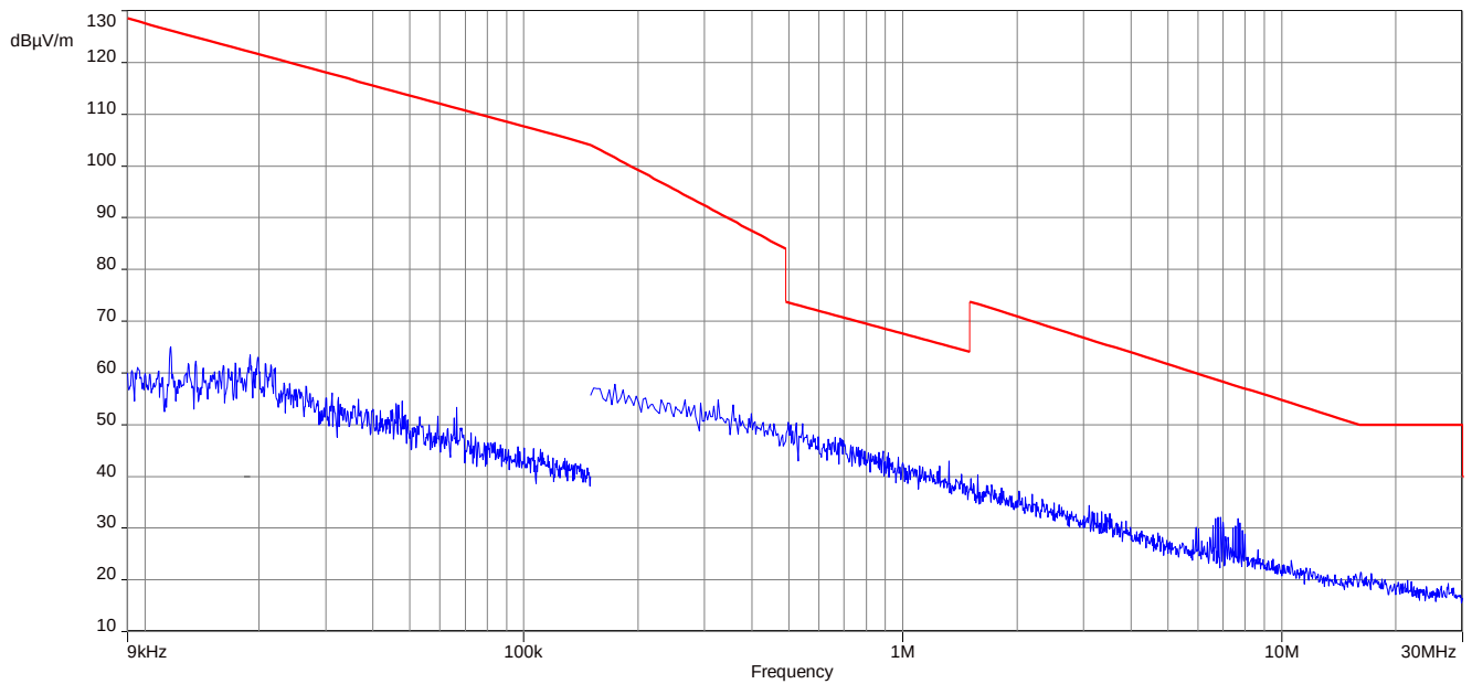
Plot 6: 9 kHz to 30 MHz, OFDM 20 MHz, 5825 MHz
