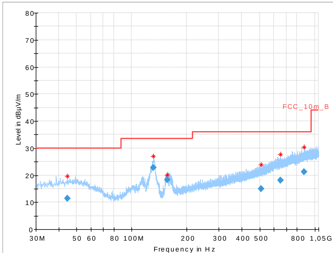
Plot 9: 30 MHz to 1 GHz, 5320 MHz, vertical & horizontal polarization
