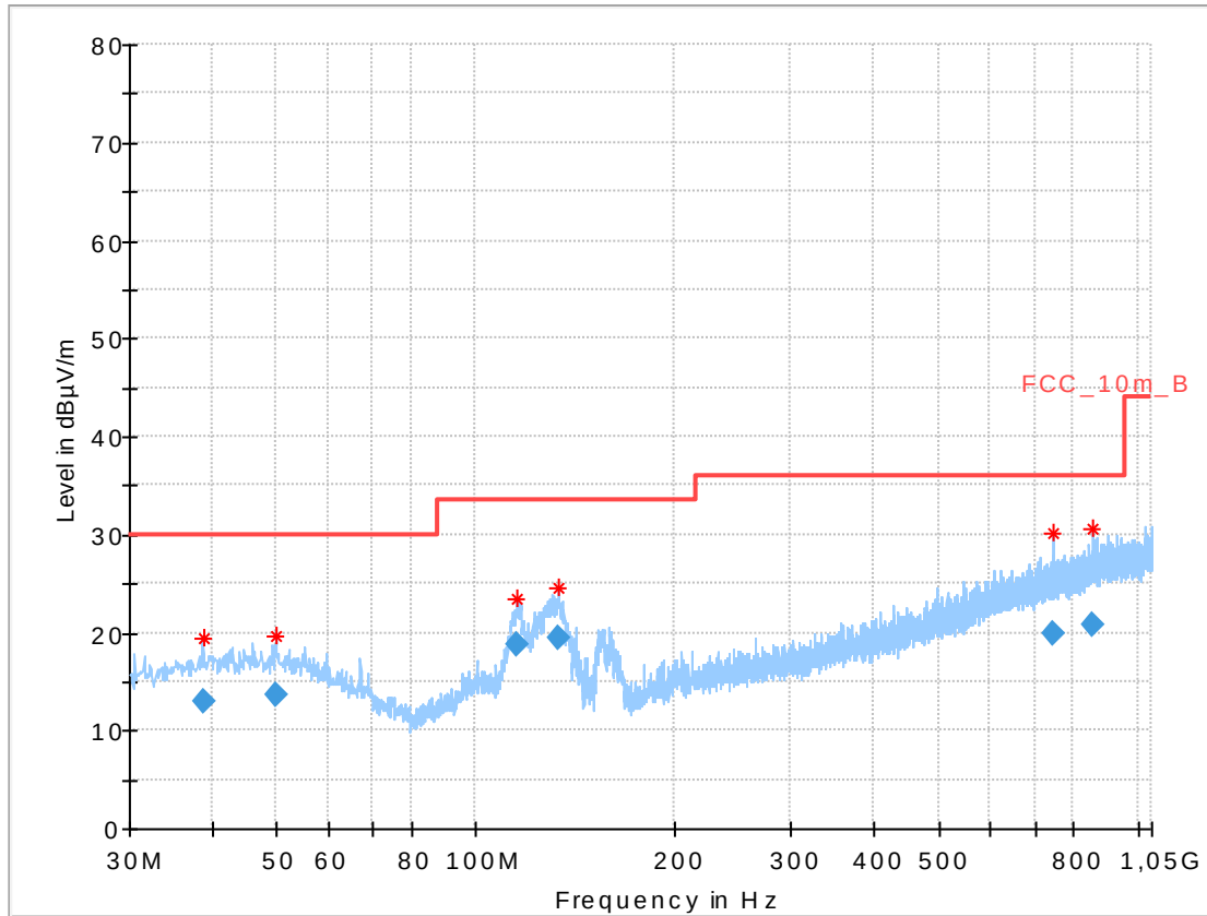
Plot 17: 30 MHz to 1 GHz, 5795 MHz, vertical & horizontal polarization
