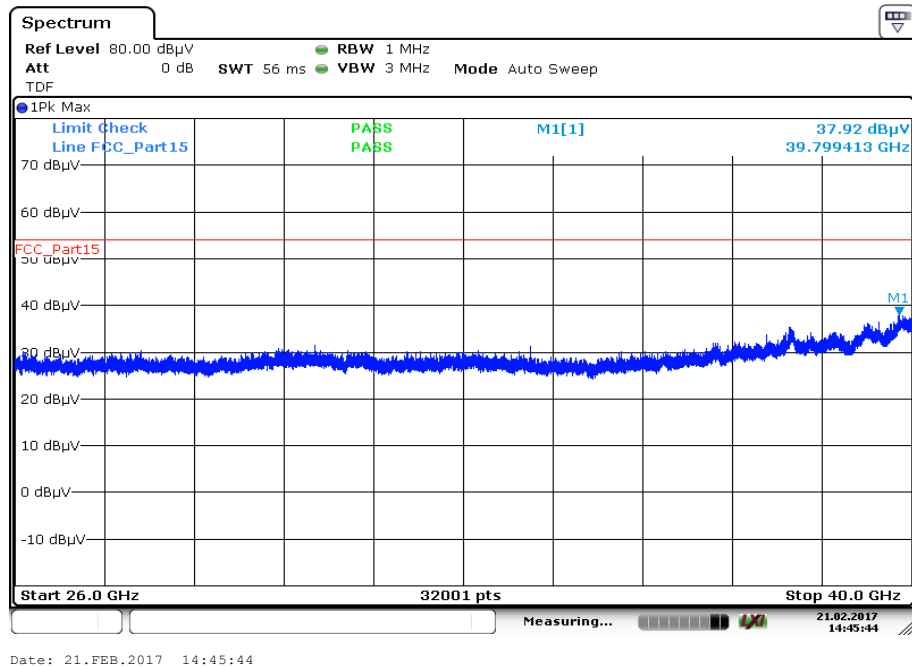
Plot 32: 26 GHz to 40 GHz, 5825 MHz, vertical & horizontal polarization
