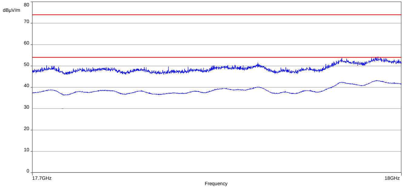
Plot 12: 17.7 GHz to 18 GHz, 5320 MHz, vertical & horizontal polarization
