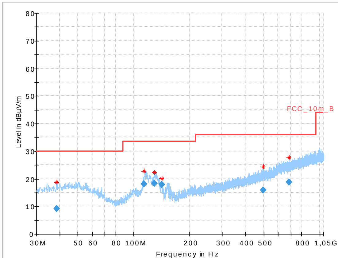
Plot 9: 30 MHz to 1 GHz, 5310 MHz, vertical & horizontal polarization
