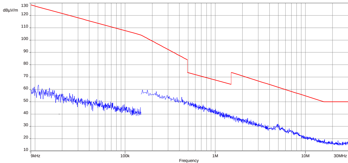
Plot 10: 9 kHz to 30 MHz, OFDM 40 MHz, 5755 MHz
