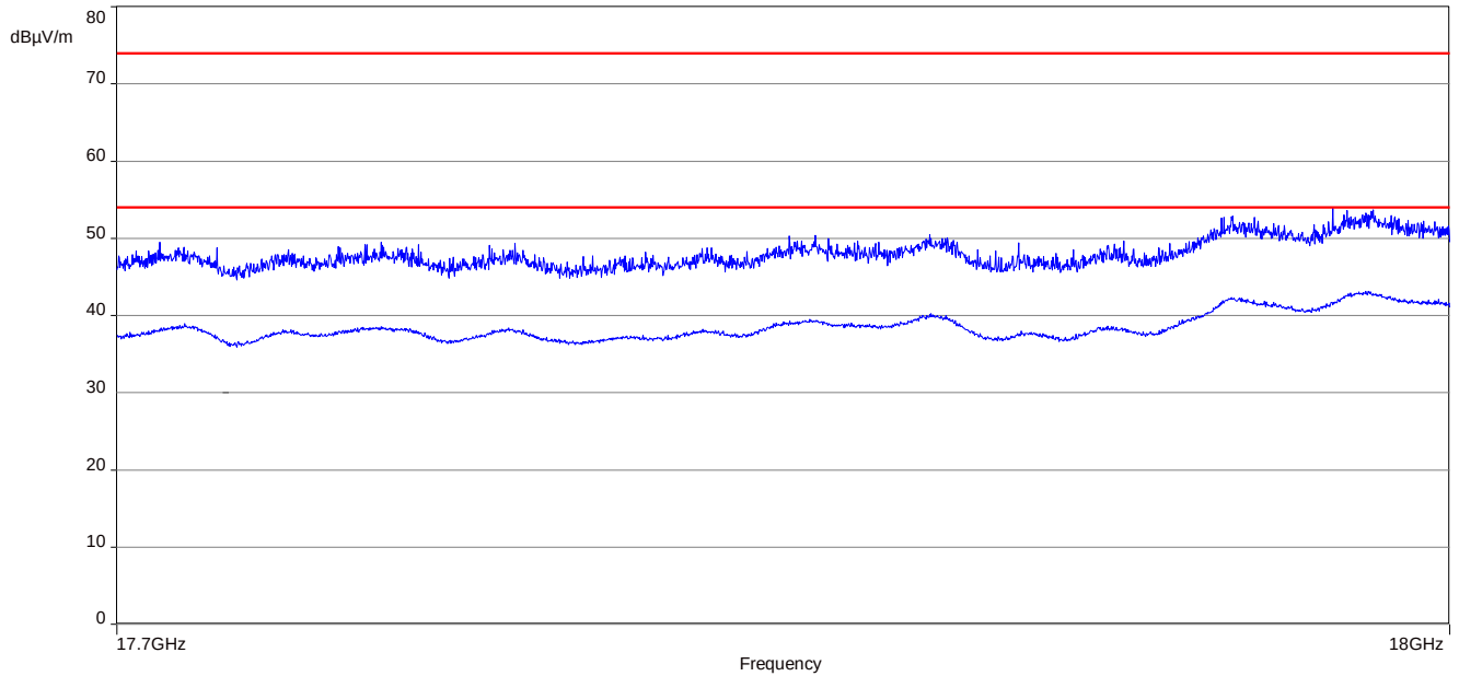
Plot 30: 17.7 GHz to 18 GHz, 5825 MHz, vertical & horizontal polarization
