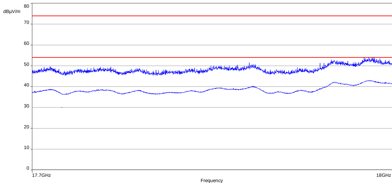
Plot 18: 17.7 GHz to 18 GHz, 5745 MHz, vertical & horizontal polarization
