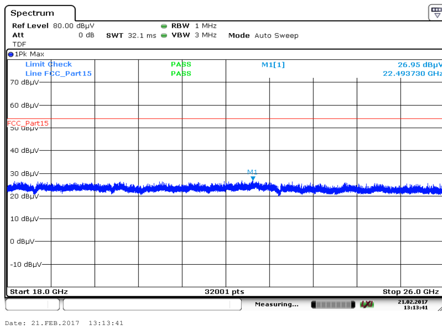
Plot 19: 18 GHz to 26 GHz, 5795 MHz, vertical & horizontal polarization
