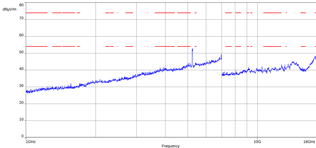
Plot 6: 1 GHz to 18 GHz, 5250 MHz, vertical & horizontal polarization
