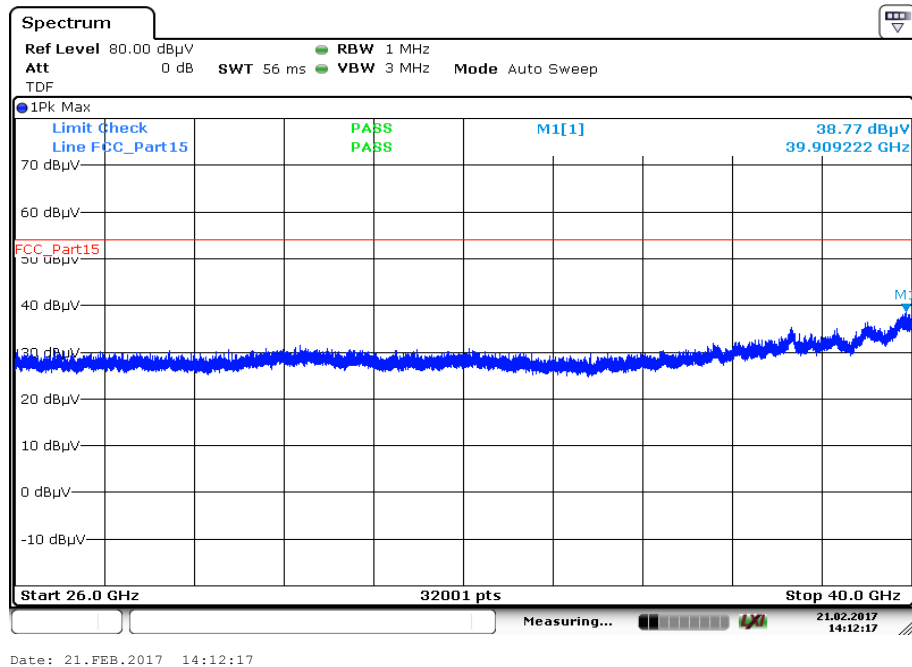
Plot 16: 26 GHz to 40 GHz, 5755 MHz, vertical & horizontal polarization
