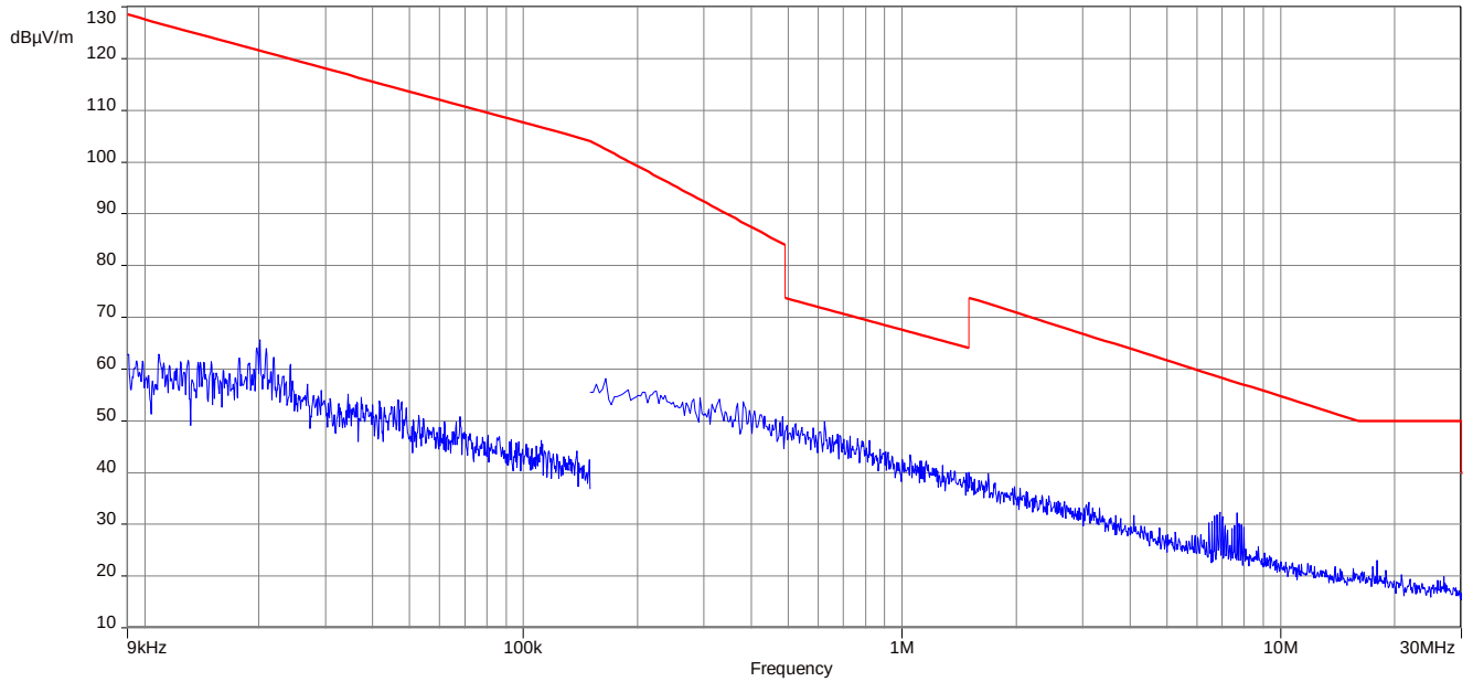
Plot 3: 9 kHz to 30 MHz, OFDM 20 MHz, 5320 MHz
