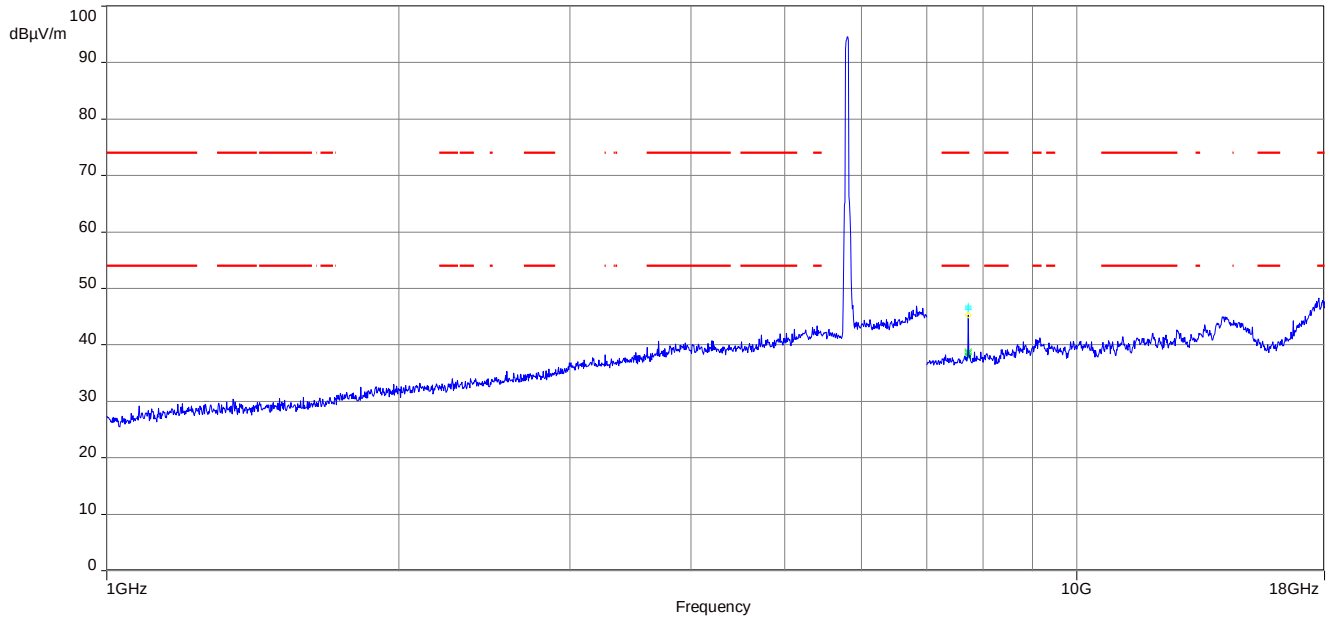
Plot 18: 1 GHz to 18 GHz, 5795 MHz, vertical & horizontal polarization
