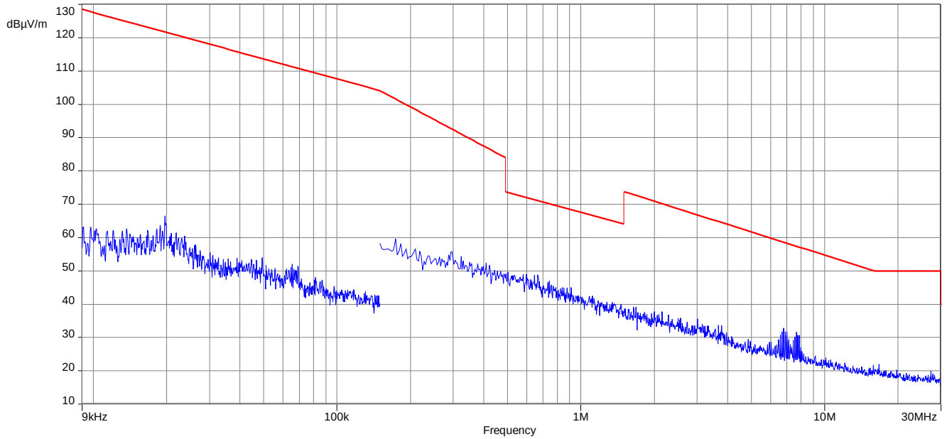
Plot 5: 9 kHz to 30 MHz, OFDM 20 MHz, 5785 MHz
