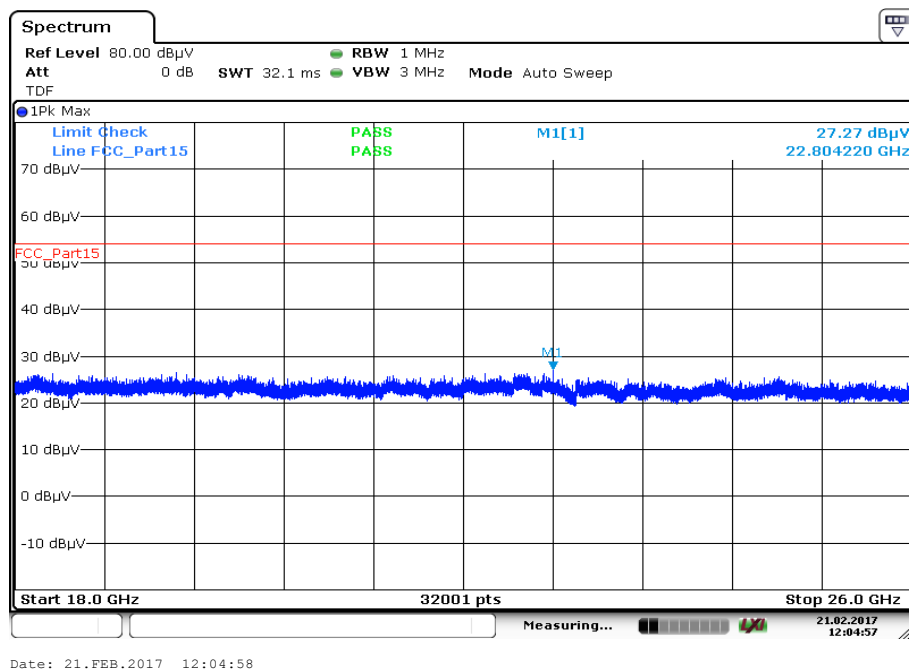
Plot 31: 18 GHz to 26 GHz, 5825 MHz, vertical & horizontal polarization
