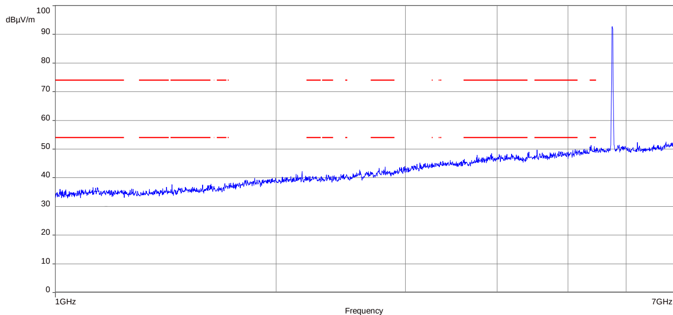
Plot 16: 1 GHz to 7 GHz, 5745 MHz, vertical & horizontal polarization
