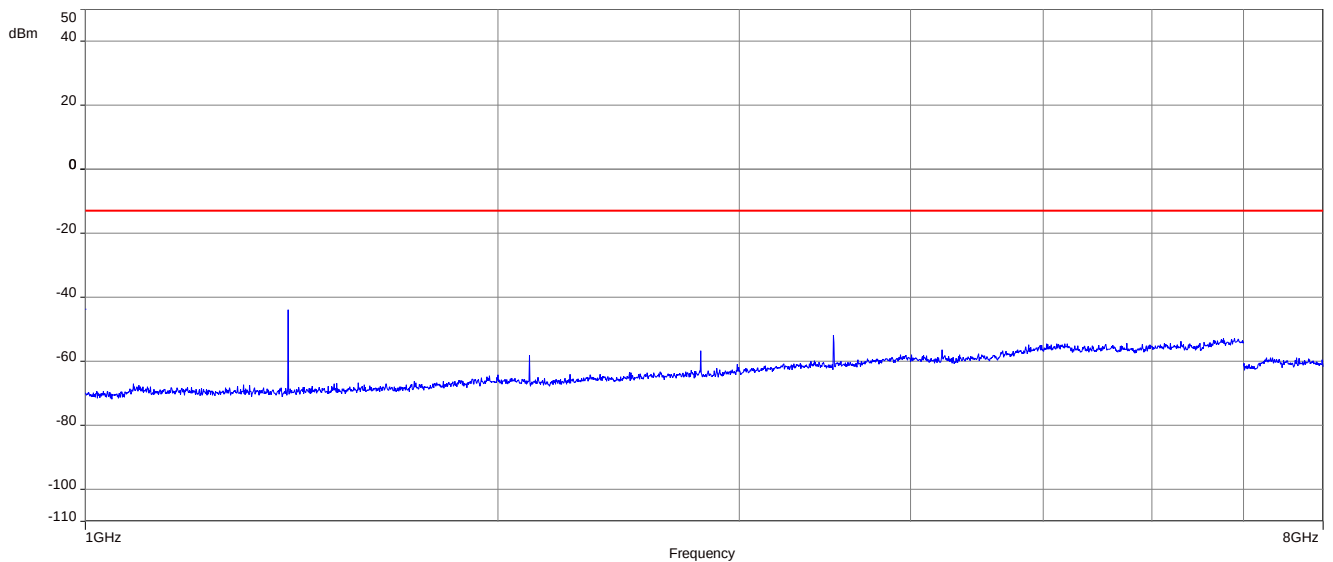
Plot 2: Middle channel (1 GHz – 8 GHz), LTE band 12
