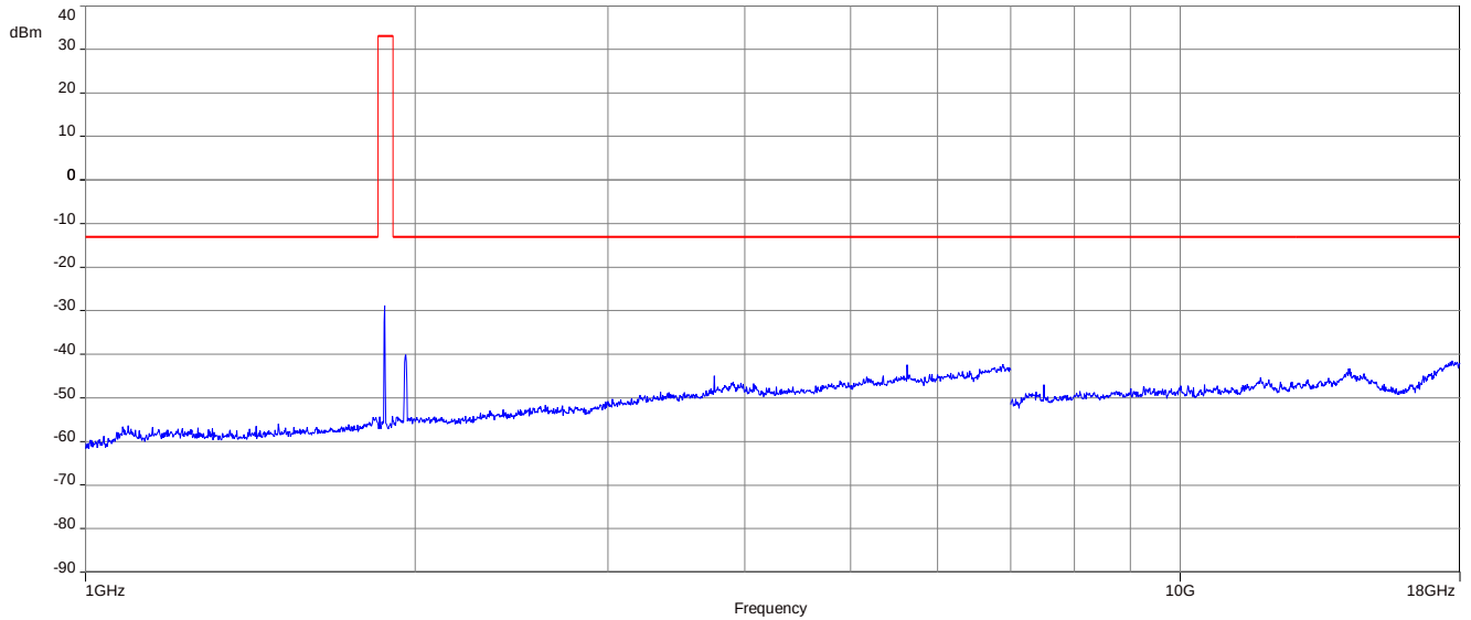
Plot 1: Middle channel (1 GHz – 18 GHz), LTE band 2
