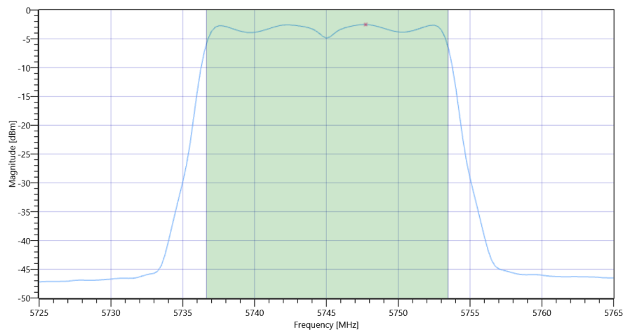
ISSED RSS247 # Max output power and psd ~ WLAN5Gx a mode U-NII-3 Max OP and PSD
