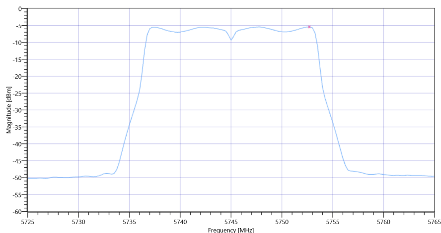
ISSED RSS247 # Max output power and psd ~ WLAN5Gx a mode U-NII-3 PSD UNII-3
