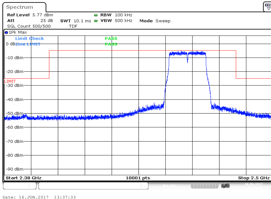
Plot 12: Channel 11, zoomed carrier
