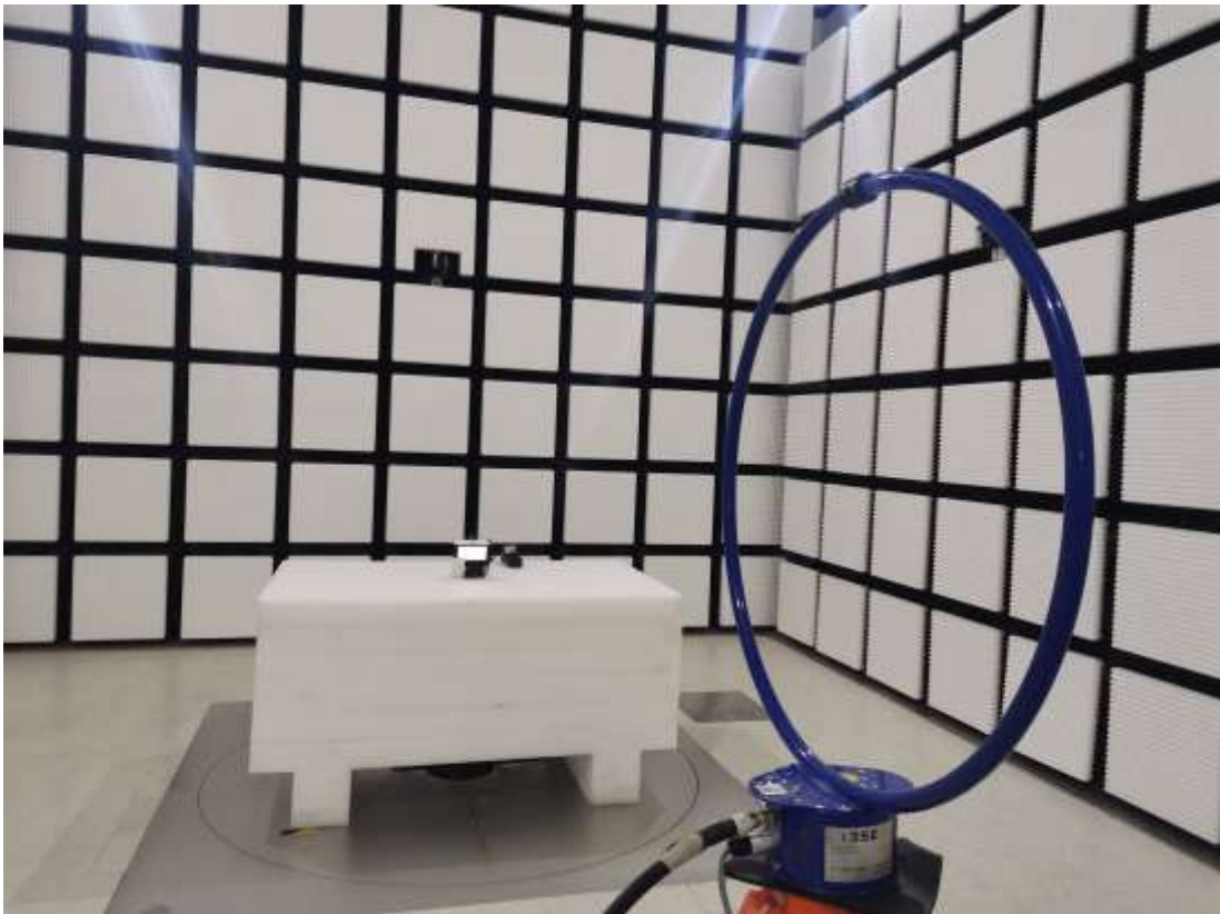
Radiated Emission Below 1G View Perpendicular
