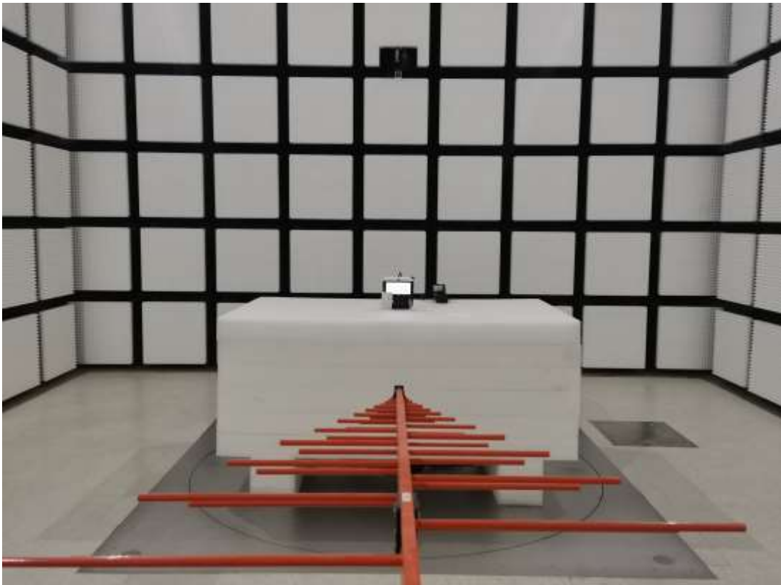
Radiated Emission Below 1G View
