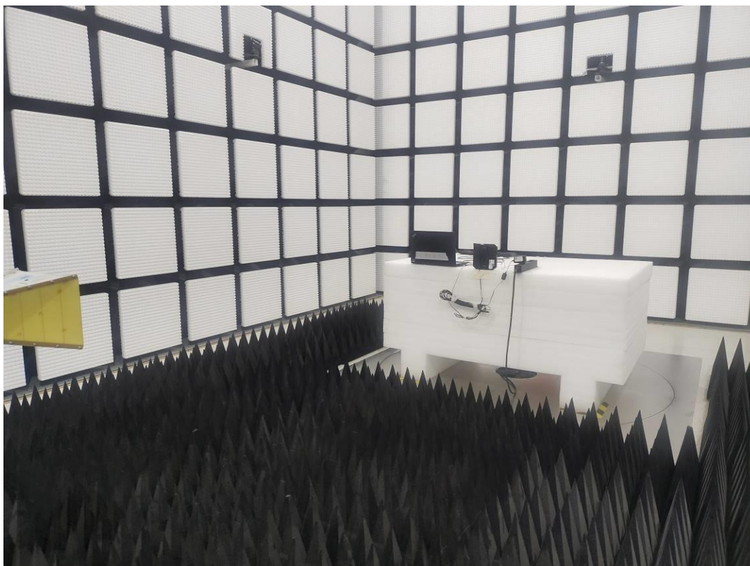
Radiated Emission Above 1GHz rear View M5
