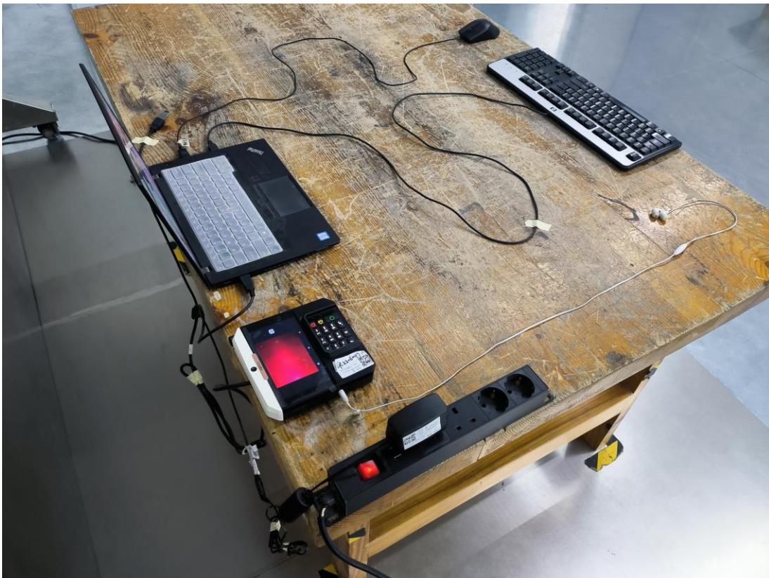
Conducted Emissions Side View M5
