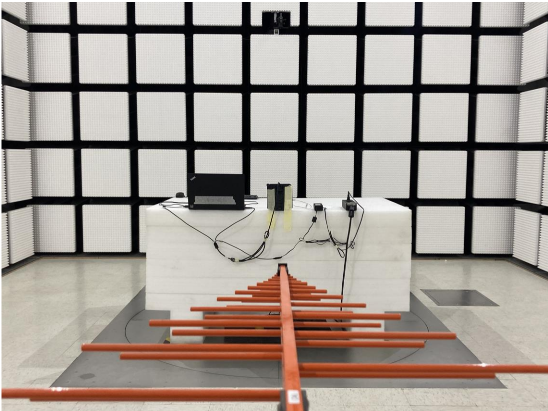
Radiated Emission Below 1GHz rear View Adapter 3#M5
