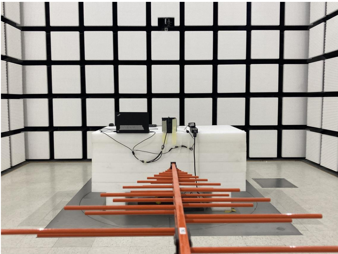
Radiated Emission Below 1GHz rear View M5
