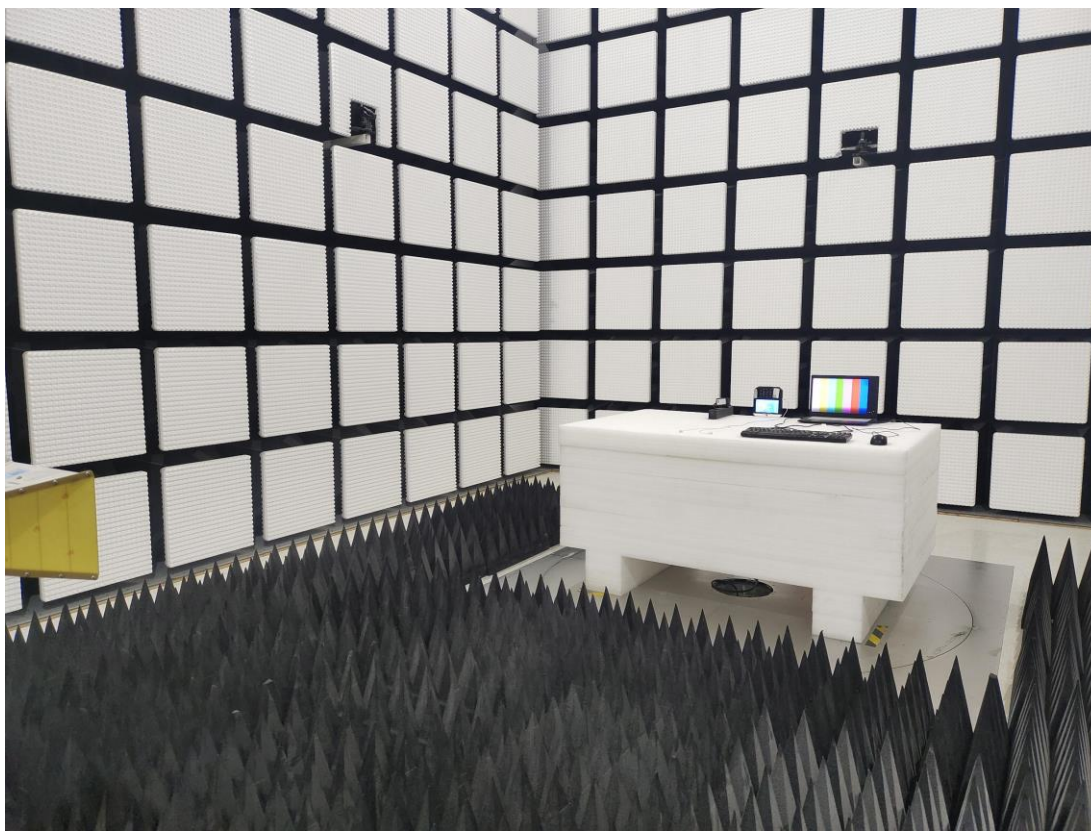
Radiated Emission Above 1GHz rear View M4
