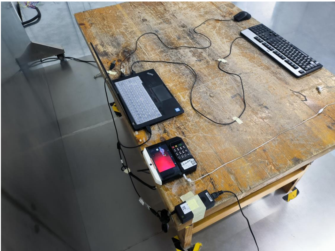
Conducted Emissions Side View Adapter 3# M5
